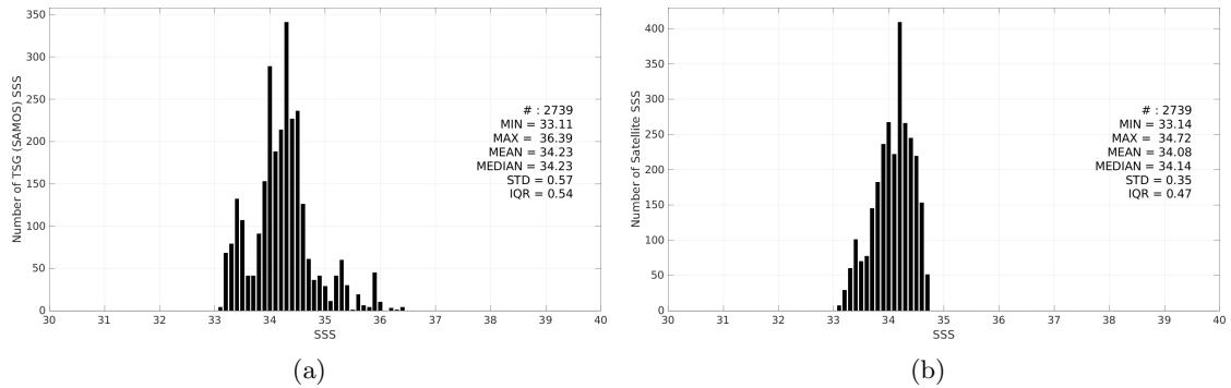
Figure 3: Histograms of SSS from TSG (SAMOS) (a) and SMOS SSS L3 v335 - Monthly - 25 km (CATDS-CPDC) (b) considering all match-up pairs per bins of 0.1 over the SPURS 2 Pi-MEP region and for the full satellite product period.
