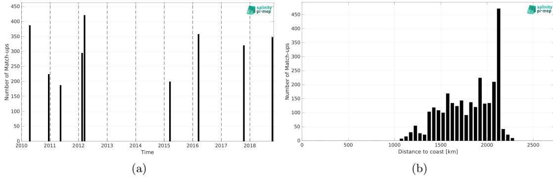
Figure 2: Number of match-ups between TSG (SAMOS) and SMOS SSS L3 v335 - Monthly - 25 km (CATDS-CPDC) SSS as a function of time (a) and as function of the distance to coast (b) over the SPURS 2 Pi-MEP region and for the full satellite product period.
