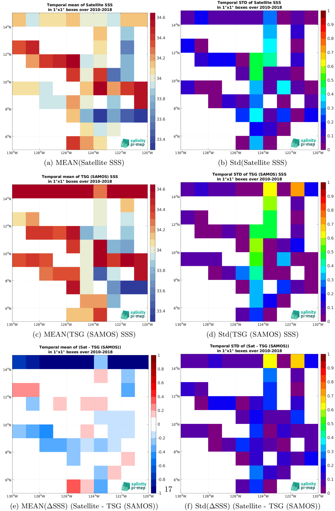
Figure 7: Temporal mean (left) and Std (right) of SSS from SMOS SSS L3 v335 - Monthly - 25 km (CATDS-CPDC) (top), TSG (SAMOS) (middle), and of \Delta SSS (Satellite - TSG (SAMOS)). Only match-up pairs are used to generate these maps.
