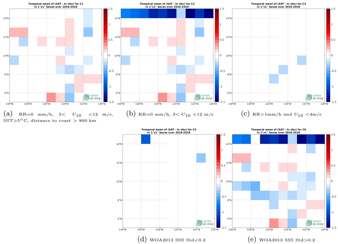
Figure 12: Temporal mean gridded over spatial boxes of size 1^\circ \times 1^\circ of \Delta SSS (SMOS SSS L3 v335 - Monthly - 25 km (CATDS-CPDC) - TSG (SAMOS)) for 5 different subdatasets corresponding to:RR=0 mm/h, 3 < U_{10} < 12 m/s, SST >5^\circ\text{C} , distance to coast > 800 km (a), RR=0 mm/h, 3 < U_{10} < 12 m/s (b), RR >1 mm/h and U_{10} < 4 m/s (c), WOA2013 SSS Std <0.2 (d), WOA2013 SSS Std >0.2 (e).
