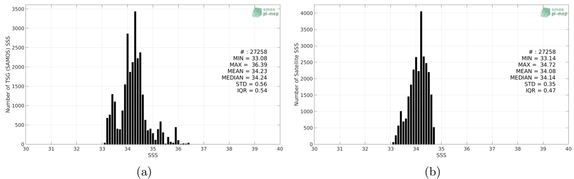
Figure 2: Histograms of SSS from TSG (SAMOS) (a) and SMOS SSS L3 v335 - Monthly - 25 km (CATDS-CPDC) (b) considering all match-up pairs per bins of 0.1 over the SPURS 2 Pi-MEP region and for the full satellite product period.
