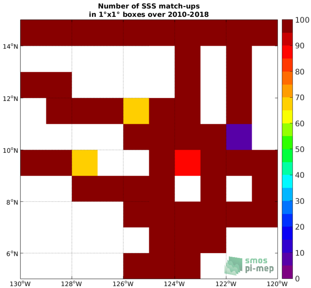
Figure 4: Number of SSS match-ups between TSG (SAMOS) SSS and the SMOS SSS L3 v335 - Monthly - 25 km (CATDS-CPDC) SSS product for the SPURS 2 Pi-MEP region over 1^\circ \times 1^\circ boxes and for the full satellite product period.
