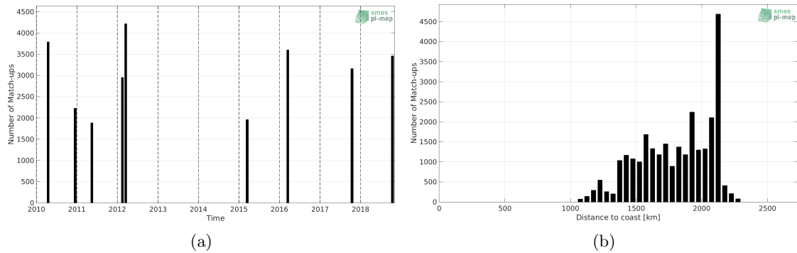
Figure 1: Number of match-ups between TSG (SAMOS) and SMOS SSS L3 v335 - Monthly - 25 km (CATDS-CPDC) SSS as a function of time (a) and as function of the distance to coast (b) over the SPURS 2 Pi-MEP region and for the full satellite product period.
