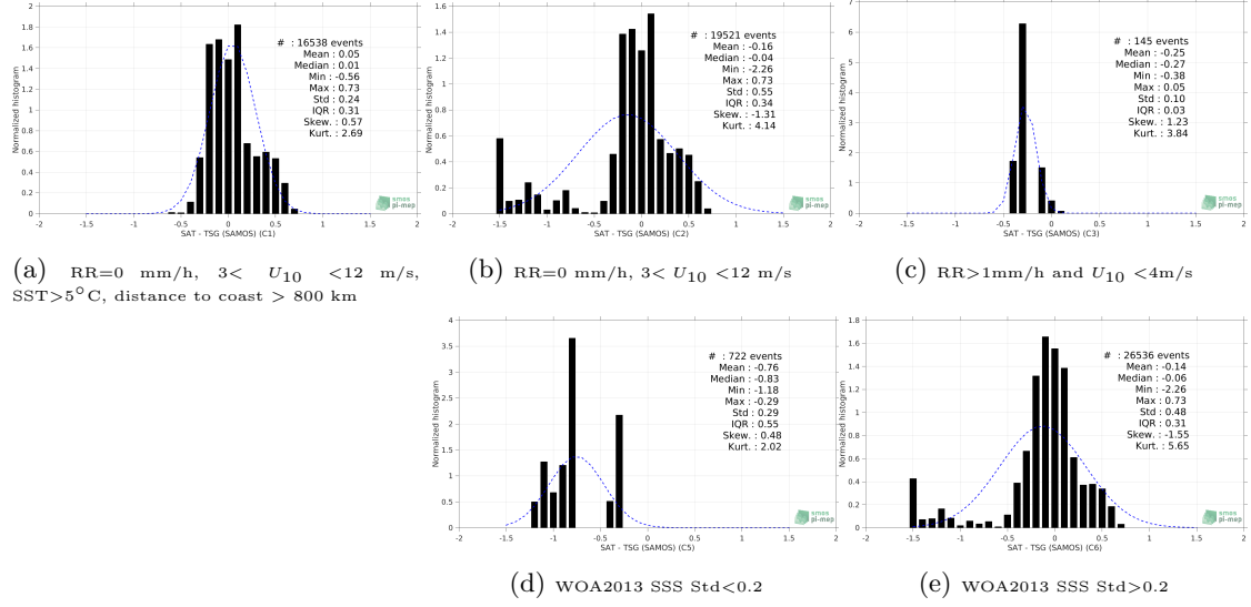
Figure 13: Normalized histogram of \Delta\text{SSS} (SMOS SSS L3 v335 - Monthly - 25 km (CATDS-CPDC) - TSG (SAMOS)) for 5 different subdatasets corresponding to: RR=0 mm/h, 3 < U_{10} < 12 m/s, SST>5°C, distance to coast > 800 km (a), RR=0 mm/h, 3 < U_{10} < 12 m/s (b), RR>1mm/h and U_{10} < 4 m/s (c), WOA2013 SSS Std<0.2 (d), WOA2013 SSS Std>0.2 (e).
