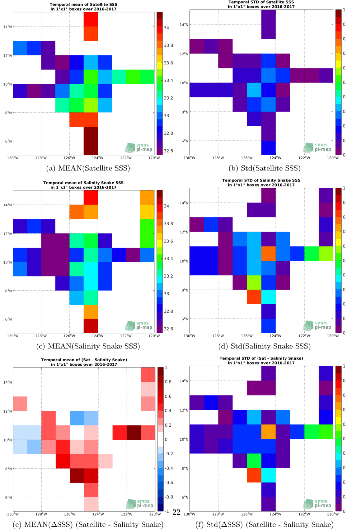
Figure 5: Temporal mean (left) and Std (right) of SSS from SMOS SSS L3 v335 - Monthly - 25 km (CATDS-CPDC) (top), Salinity Snake (middle), and of \Delta SSS (Satellite - Salinity Snake). Only match-up pairs are used to generate these maps.
