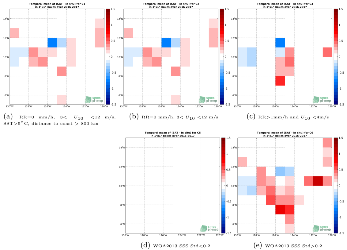
Figure 11: Temporal mean gridded over spatial boxes of size 1^\circ \times 1^\circ of \Delta SSS (SMOS SSS L3 v335 - Monthly - 25 km (CATDS-CPDC) - Salinity Snake) for 5 different subdatasets corresponding to:RR=0 mm/h, 3 < U_{10} < 12 m/s, SST >5^\circ\text{C} , distance to coast > 800 km (a), RR=0 mm/h, 3 < U_{10} < 12 m/s (b), RR >1 mm/h and U_{10} < 4 m/s (c), WOA2013 SSS Std <0.2 (d), WOA2013 SSS Std >0.2 (e).
