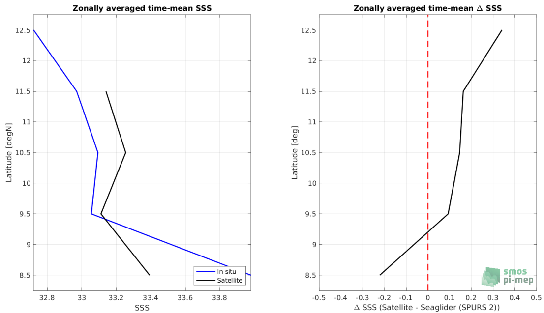
Figure 8: Left panel: Zonal mean SSS from SMOS SSS L3 v335 - Monthly - 25 km (CATDS-CPDC) satellite product (black) and from Seaglider (SPURS 2) (blue). Right panel: Zonal mean of \Delta SSS (Satellite - Seaglider (SPURS 2)) for all the collected Pi-MEP match-up pairs estimated over the full satellite product period.
