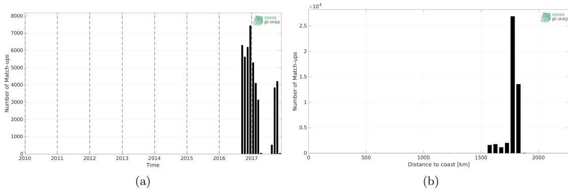
Figure 1: Number of match-ups between Seaglider (SPURS 2) and SMOS SSS L3 v335 - Monthly - 25 km (CATDS-CPDC) SSS as a function of time (a) and as function of the distance to coast (b) over the SPURS 2 Pi-MEP region and for the full satellite product period.
