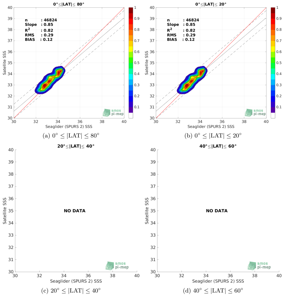
Figure 9: Contour maps of the concentration of SMOS SSS L3 v335 - Monthly - 25 km (CATDS-CPDC) SSS (y-axis) versus Seaglider (SPURS 2) SSS (x-axis) at match-up pairs for different latitude bands. For each plot, the red line shows x=y . The black thin and dashed lines indicate a linear fit through the data cloud and the \pm 95\% confidence levels, respectively. The number match-up pairs n , the slope and R^2 coefficient of the linear fit, the root mean square (RMS) and the mean bias between satellite and in situ data are indicated for each latitude band in each plots.
