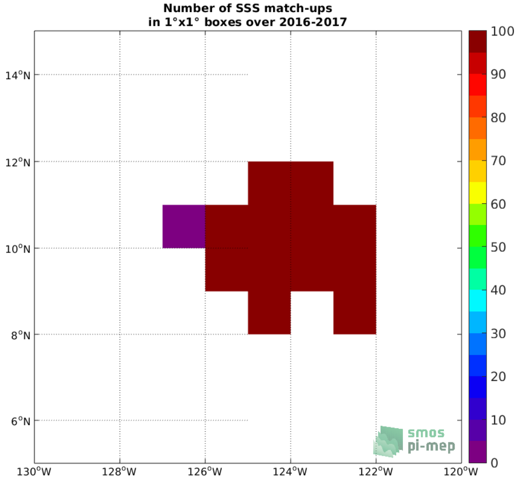
Figure 3: Number of SSS match-ups between Seaglider SSS and the SMOS SSS L3 v335 - Monthly - 25 km (CATDS-CPDC) SSS product for the SPURS 2 Pi-MEP region over 1^\circ \times 1^\circ boxes and for the full satellite product period.
