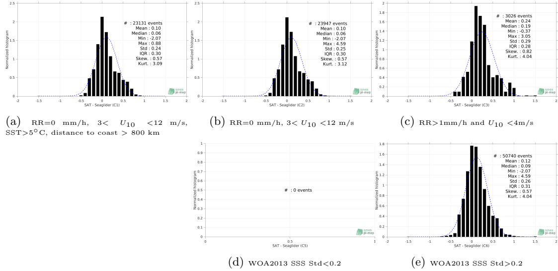
Figure 12: Normalized histogram of \Delta SSS (SMOS SSS L3 v335 - Monthly - 25 km (CATDS-CPDC) - Seaglider) for 5 different subdatasets corresponding to: RR=0 mm/h, 3 < U_{10} < 12 m/s, SST>5°C, distance to coast > 800 km (a), RR=0 mm/h, 3 < U_{10} < 12 m/s (b), RR>1mm/h and U_{10} < 4 m/s (c), WOA2013 SSS Std<0.2 (d), WOA2013 SSS Std>0.2 (e).
