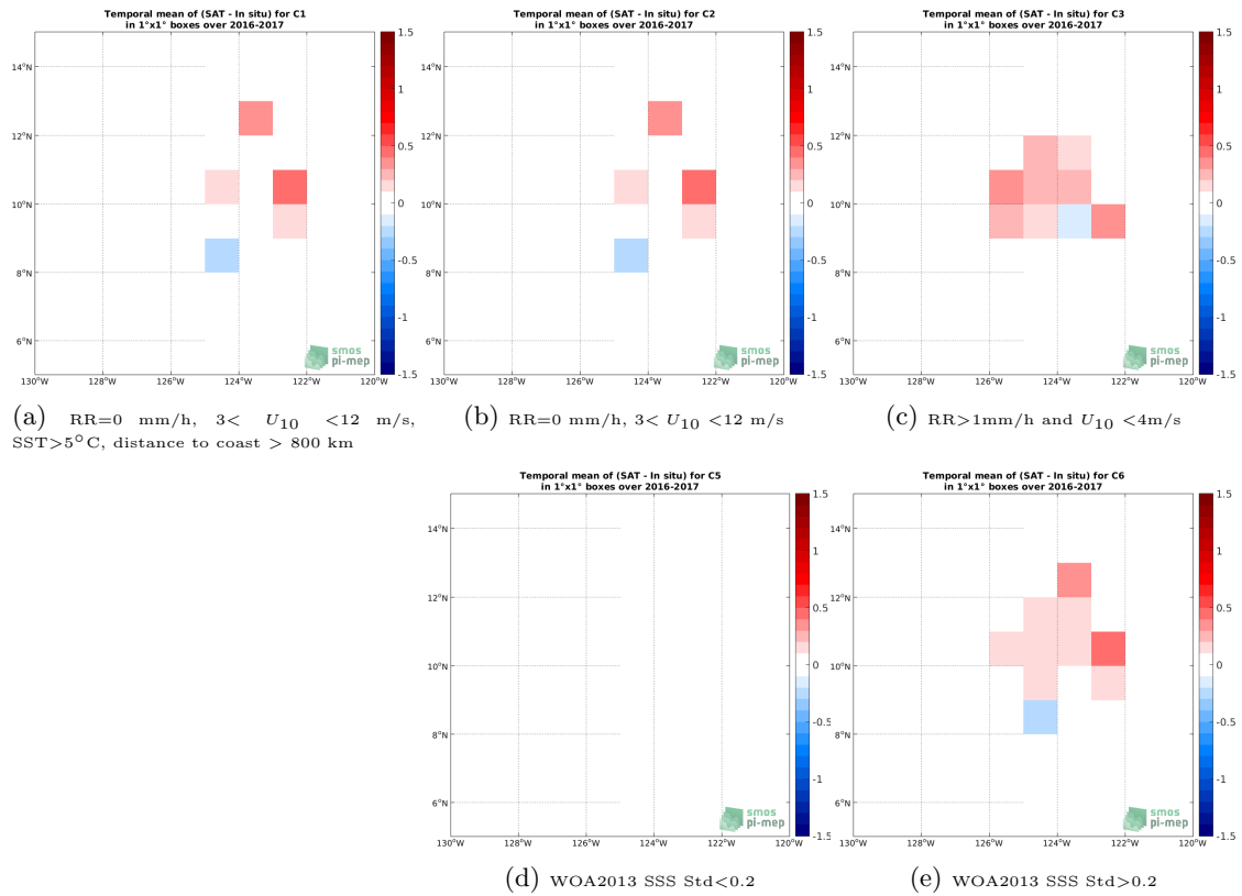
Figure 11: Temporal mean gridded over spatial boxes of size 1^\circ \times 1^\circ of \Delta SSS (SMOS SSS L3 v335 - Monthly - 25 km (CATDS-CPDC) - Seaglider) for 5 different subdatasets corresponding to:RR=0 mm/h, 3 < U_{10} < 12 m/s, SST >5^\circ\text{C} , distance to coast > 800 km (a), RR=0 mm/h, 3 < U_{10} < 12 m/s (b), RR >1 mm/h and U_{10} < 4 m/s (c), WOA2013 SSS Std <0.2 (d), WOA2013 SSS Std >0.2 (e).
