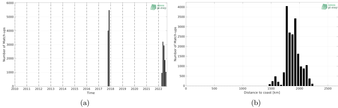
Figure 1: Number of match-ups between Sairdrone and SMOS SSS L3 v335 - Monthly - 25 km (CATDS-CPDC) SSS as a function of time (a) and as function of the distance to coast (b) over the SPURS 2 Pi-MEP region and for the full satellite product period.
