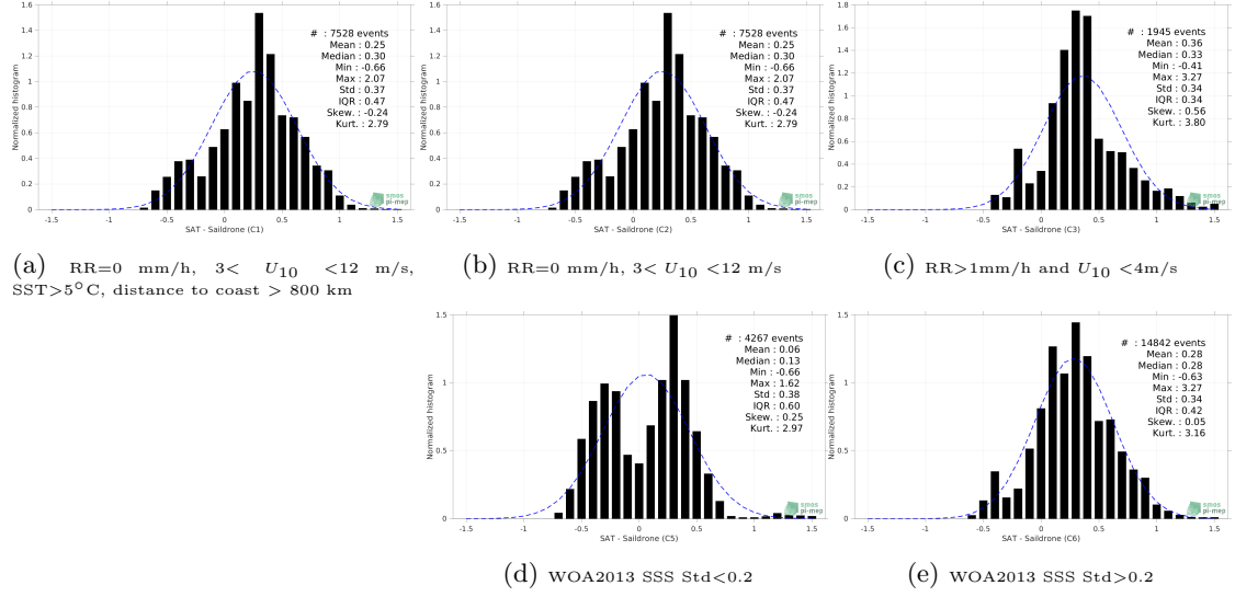
Figure 13: Normalized histogram of \Delta SSS (SMOS SSS L3 v335 - Monthly - 25 km (CATDS-CPDC) - Sairdrone) for 5 different subdatasets corresponding to: RR=0 mm/h, 3 < U_{10} < 12 m/s, SST>5°C, distance to coast > 800 km (a), RR=0 mm/h, 3 < U_{10} < 12 m/s (b), RR>1mm/h and U_{10} < 4 m/s (c), WOA2013 SSS Std<0.2 (d), WOA2013 SSS Std>0.2 (e).
