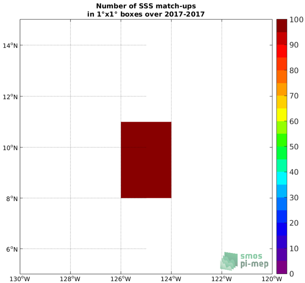
Figure 3: Number of SSS match-ups between Sairdrone SSS and the SMOS SSS L3 v335 - Monthly - 25 km (CATDS-CPDC) SSS product for the SPURS 2 Pi-MEP region over 1°x1° boxes and for the full satellite product period.
