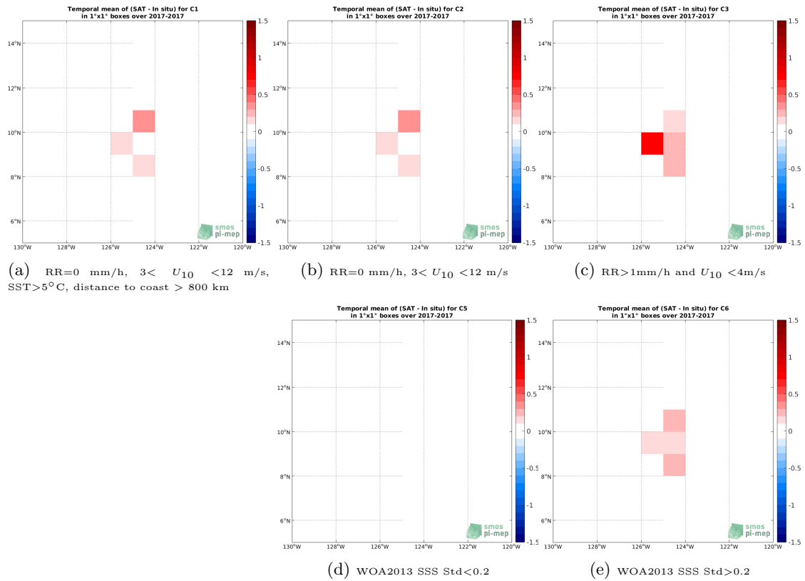
Figure 11: Temporal mean gridded over spatial boxes of size 1^\circ \times 1^\circ of \Delta SSS (SMOS SSS L3 v335 - Monthly - 25 km (CATDS-CPDC) - Saildrone) for 5 different subdatasets corresponding to:RR=0 mm/h, 3 < U_{10} < 12 m/s, SST >5^\circ\text{C} , distance to coast > 800 km (a), RR=0 mm/h, 3 < U_{10} < 12 m/s (b), RR >1 mm/h and U_{10} < 4 m/s (c), WOA2013 SSS Std <0.2 (d), WOA2013 SSS Std >0.2 (e).
