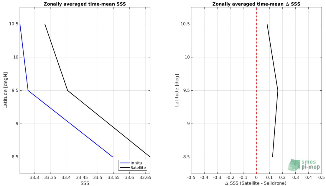
Figure 7: Left panel: Zonal mean SSS from SMOS SSS L3 v335 - Monthly - 25 km (CATDS-CPDC) satellite product (black) and from Saiddrone (blue). Right panel: Zonal mean of \Delta SSS (Satellite - Saiddrone) for all the collected Pi-MEP match-up pairs estimated over the full satellite product period.
