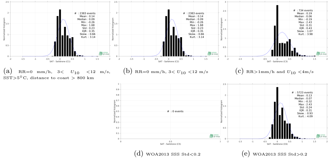
Figure 12: Normalized histogram of \Delta SSS (SMOS SSS L3 v335 - Monthly - 25 km (CATDS-CPDC) - Saildrone) for 5 different subdatasets corresponding to: RR=0 mm/h, 3 < U_{10} < 12 m/s, SST > 5°C, distance to coast > 800 km (a), RR=0 mm/h, 3 < U_{10} < 12 m/s (b), RR > 1mm/h and U_{10} < 4 m/s (c), WOA2013 SSS Std < 0.2 (d), WOA2013 SSS Std > 0.2 (e).
