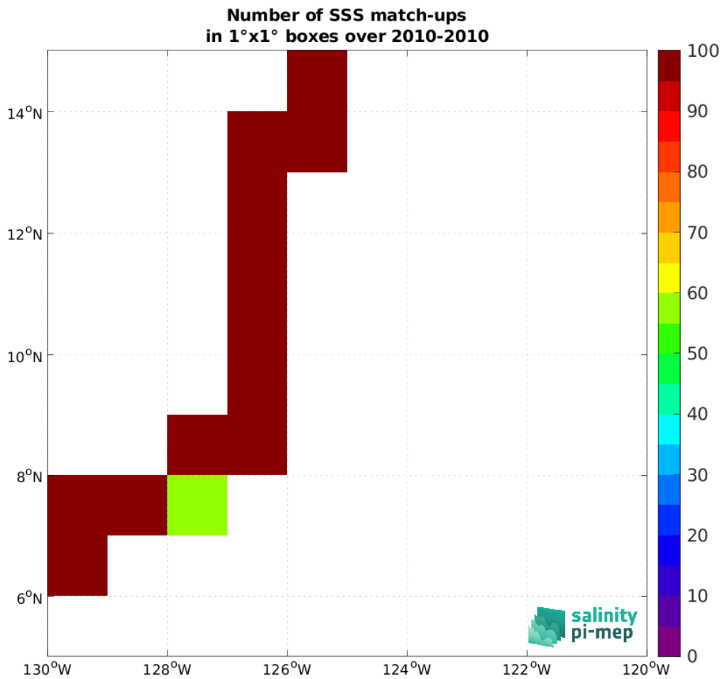
Figure 4: Number of SSS match-ups between TSG (GOSUD-Sailing-ship) SSS and the SMOS SSS L3 v335 - 10 Days - 25 km (CATDS-CPDC) SSS product for the SPURS 2 Pi-MEP region over 1^\circ \times 1^\circ boxes and for the full satellite product period.
