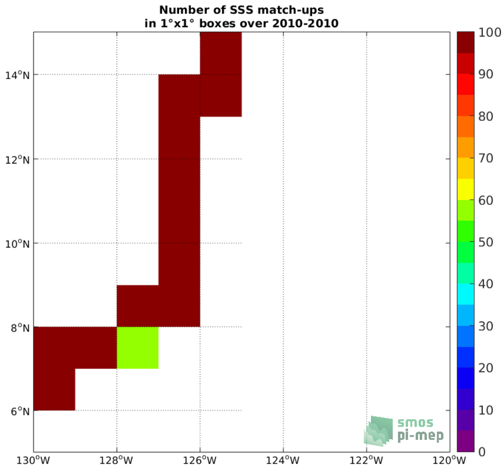
Figure 4: Number of SSS match-ups between TSG (GOSUD-Sailing-ship) SSS and the SMOS SSS L3 v335 - 10 Days - 25 km (CATDS-CPDC) SSS product for the SPURS 2 Pi-MEP region over 1°x1° boxes and for the full satellite product period.
