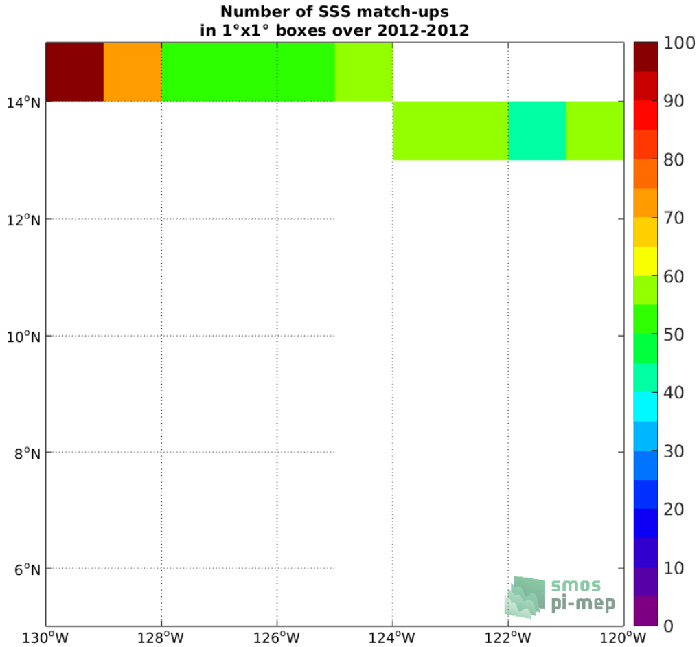
Figure 4: Number of SSS match-ups between TSG (GOSUD-Research-vessel) SSS and the SMOS SSS L3 v335 - 10 Days - 25 km (CATDS-CPDC) SSS product for the SPURS 2 Pi-MEP region over 1°×1° boxes and for the full satellite product period.
