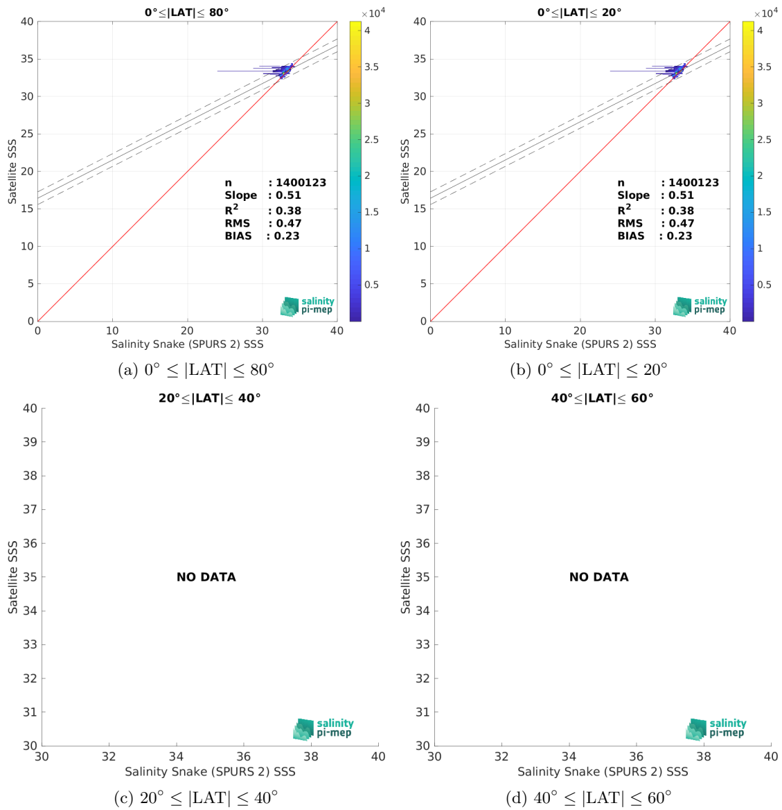
Figure 10: Contour maps of the concentration of SMOS SSS L3 v335 - 10 Days - 25 km (CATDS-CPDC) SSS (y-axis) versus Salinity Snake (SPURS 2) SSS (x-axis) at match-up pairs for different latitude bands. For each plot, the red line shows x=y . The black thin and dashed lines indicate a linear fit through the data cloud and the \pm 95\% confidence levels, respectively. The number match-up pairs n , the slope and R^2 coefficient of the linear fit, the root mean square (RMS) and the mean bias between satellite and in situ data are indicated for each latitude band in each plots.
