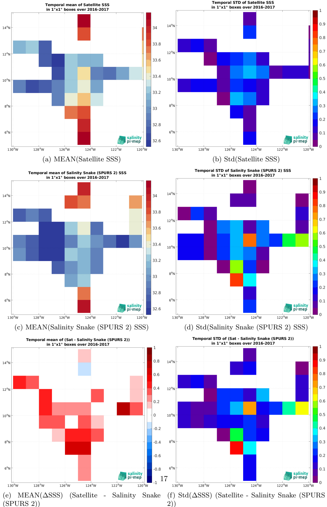
Figure 7: Temporal mean (left) and Std (right) of SSS from SMOS SSS L3 v335 - 10 Days - 25 km (CATDS-CPDC) (top), Salinity Snake (SPURS 2) (middle), and of \Delta SSS (Satellite - Salinity Snake (SPURS 2)). Only match-up pairs are used to generate these maps.
