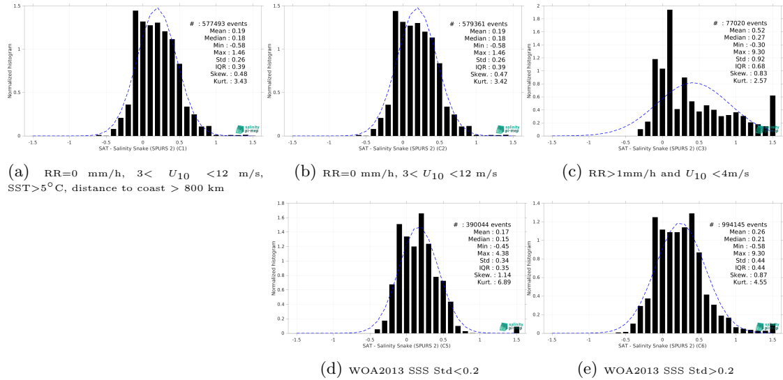
Figure 15: Normalized histogram of \Delta\text{SSS} (SMOS SSS L3 v335 - 10 Days - 25 km (CATDS-CPDC) - Salinity Snake (SPURS 2)) for 5 different subdatasets corresponding to: RR=0 mm/h, 3 < U_{10} < 12 m/s, SST>5°C, distance to coast > 800 km (a), RR=0 mm/h, 3 < U_{10} < 12 m/s (b), RR>1mm/h and U_{10} < 4 m/s (c), WOA2013 SSS Std<0.2 (d), WOA2013 SSS Std>0.2 (e).
