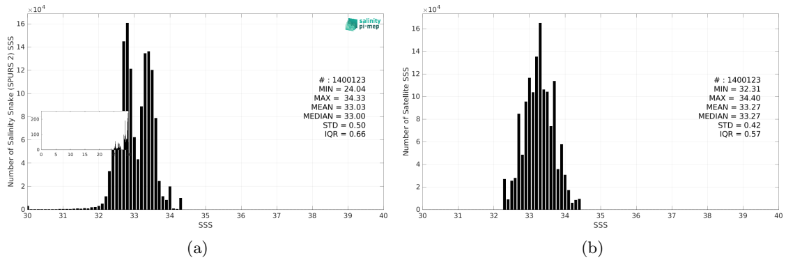
Figure 3: Histograms of SSS from Salinity Snake (SPURS 2) (a) and SMOS SSS L3 v335 - 10 Days - 25 km (CATDS-CPDC) (b) considering all match-up pairs per bins of 0.1 over the SPURS 2 Pi-MEP region and for the full satellite product period.
