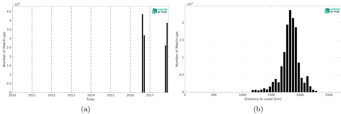
Figure 2: Number of match-ups between Salinity Snake (SPURS 2) and SMOS SSS L3 v335 - 10 Days - 25 km (CATDS-CPDC) SSS as a function of time (a) and as function of the distance to coast (b) over the SPURS 2 Pi-MEP region and for the full satellite product period.
