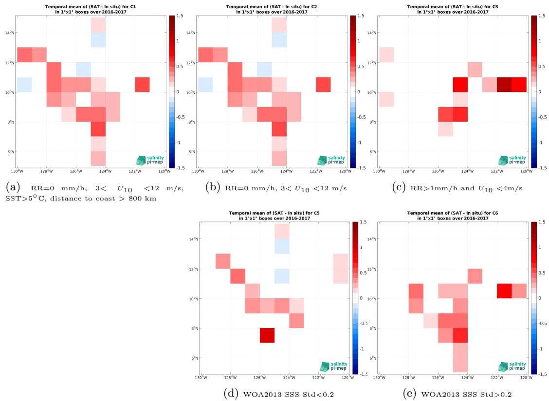
Figure 14: Temporal mean gridded over spatial boxes of size 1^\circ \times 1^\circ of \Delta\text{SSS} (SMOS SSS L3 v335 - 10 Days - 25 km (CATDS-CPDC) - Salinity Snake (SPURS 2)) for 5 different subdatasets corresponding to:RR=0 mm/h, 3 < U_{10} < 12 m/s, SST>5°C, distance to coast > 800 km (a), RR=0 mm/h, 3 < U_{10} < 12 m/s (b), RR>1mm/h and U_{10} < 4 m/s (c), WOA2013 SSS Std<0.2 (d), WOA2013 SSS Std>0.2 (e).
