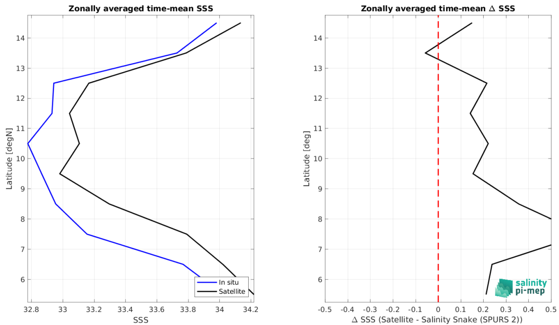
Figure 9: Left panel: Zonal mean SSS from SMOS SSS L3 v335 - 10 Days - 25 km (CATDS-CPDC) satellite product (black) and from Salinity Snake (SPURS 2) (blue). Right panel: Zonal mean of \Delta SSS (Satellite - Salinity Snake (SPURS 2)) for all the collected Pi-MEP match-up pairs estimated over the full satellite product period.
