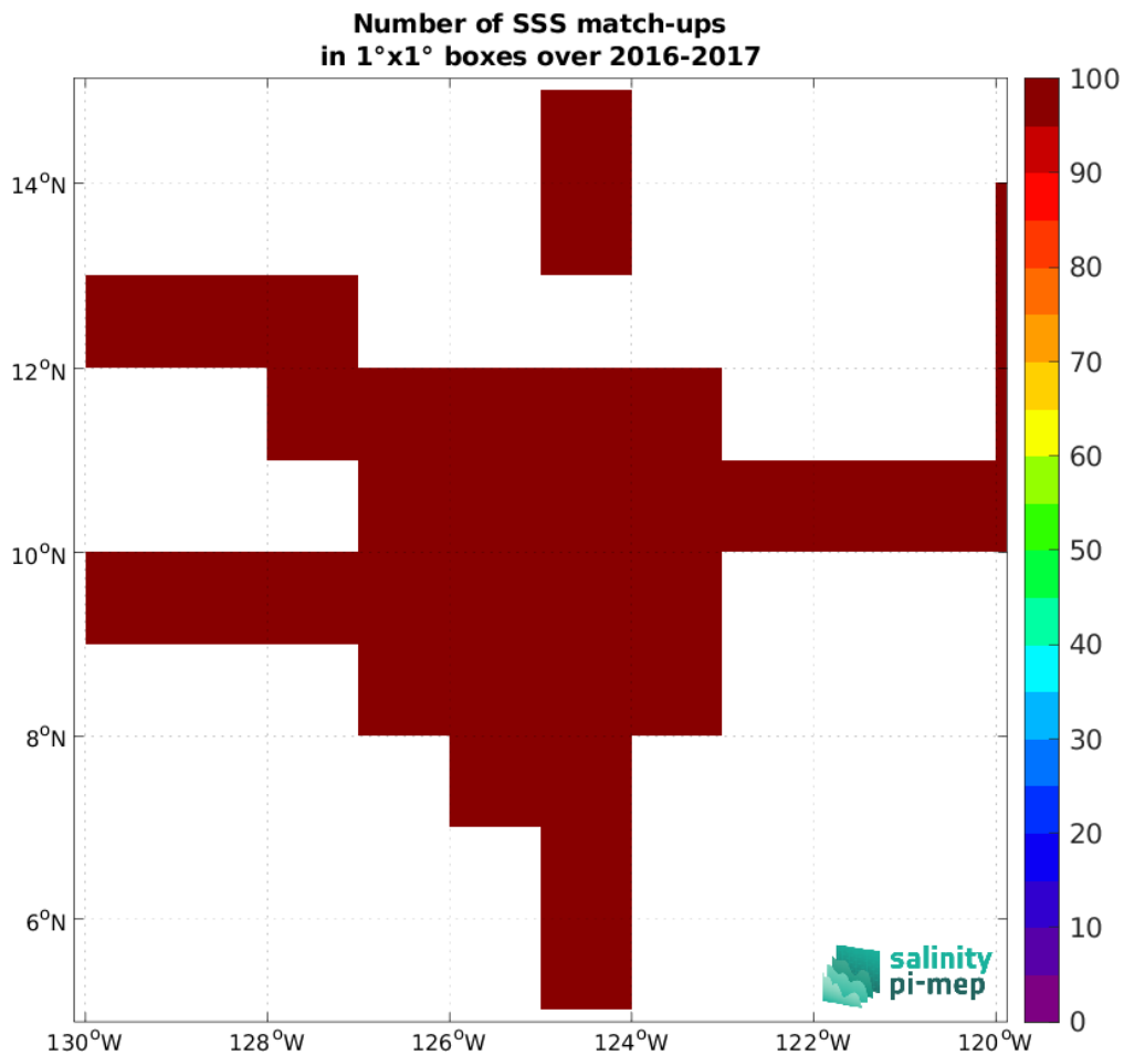
Figure 5: Number of SSS match-ups between Salinity Snake (SPURS 2) SSS and the SMOS SSS L3 v335 - 10 Days - 25 km (CATDS-CPDC) SSS product for the SPURS 2 Pi-MEP region over 1^\circ \times 1^\circ boxes and for the full satellite product period.
