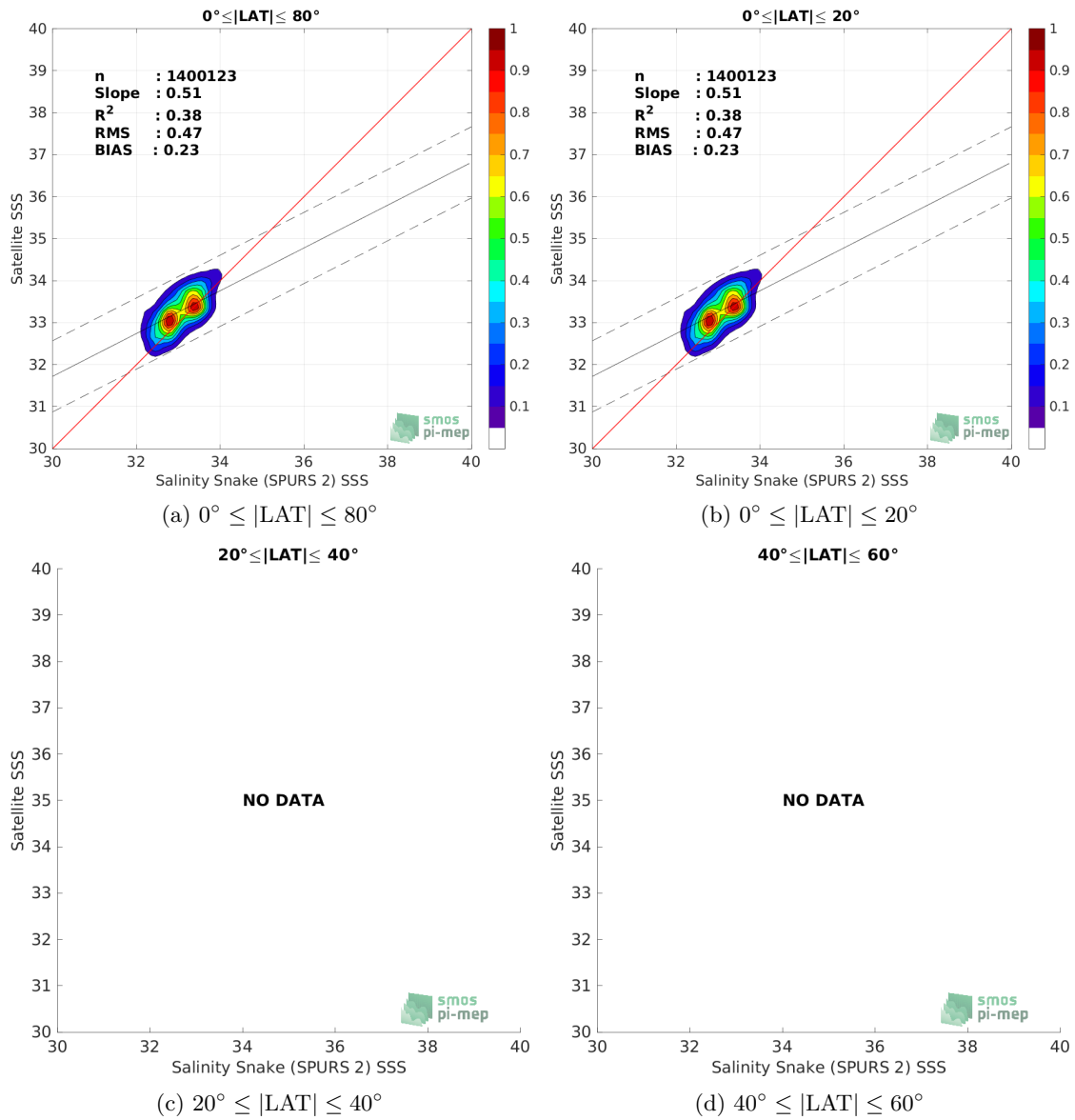
Figure 9: Contour maps of the concentration of SMOS SSS L3 v335 - 10 Days - 25 km (CATDS-CPDC) SSS (y-axis) versus Salinity Snake (SPURS 2) SSS (x-axis) at match-up pairs for different latitude bands. For each plot, the red line shows x=y . The black thin and dashed lines indicate a linear fit through the data cloud and the \pm 95\% confidence levels, respectively. The number match-up pairs n , the slope and R^2 coefficient of the linear fit, the root mean square (RMS) and the mean bias between satellite and in situ data are indicated for each latitude band in each plots.
