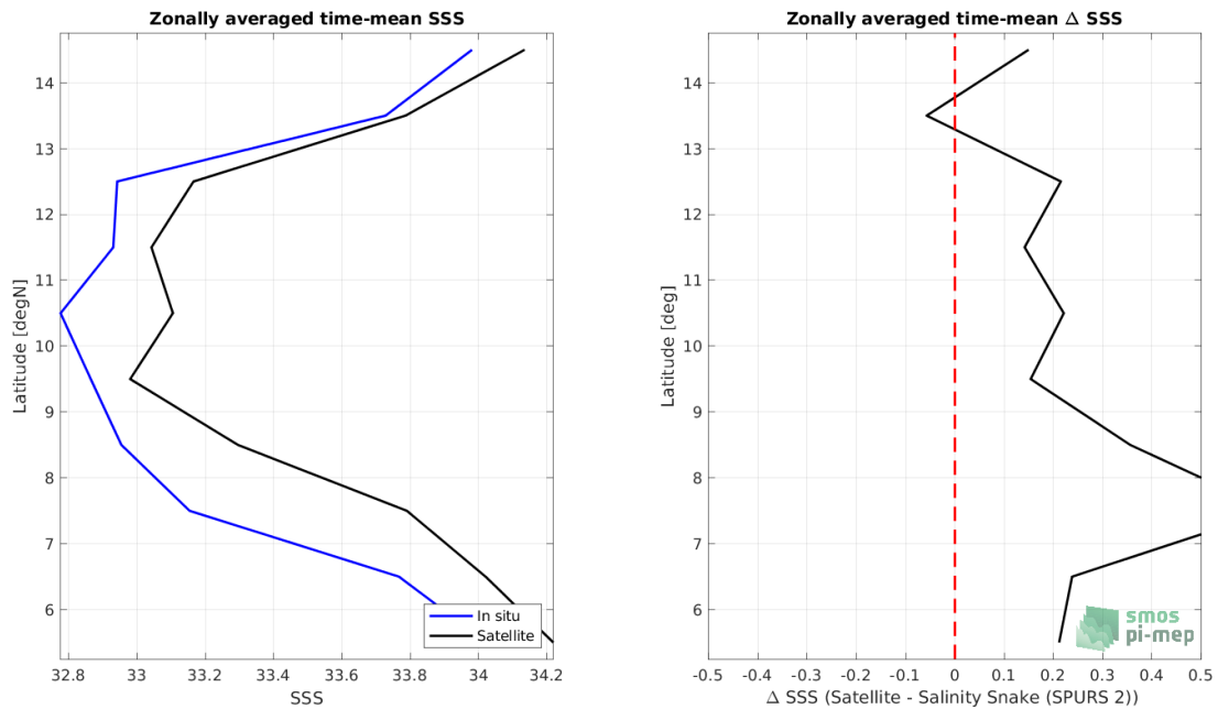
Figure 8: Left panel: Zonal mean SSS from SMOS SSS L3 v335 - 10 Days - 25 km (CATDS-CPDC) satellite product (black) and from Salinity Snake (SPURS 2) (blue). Right panel: Zonal mean of \Delta SSS (Satellite - Salinity Snake (SPURS 2)) for all the collected Pi-MEP match-up pairs estimated over the full satellite product period.
