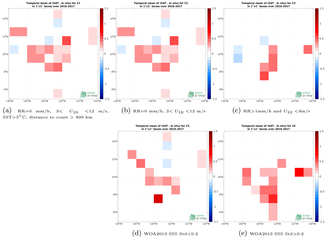
Figure 12: Temporal mean gridded over spatial boxes of size 1^\circ \times 1^\circ of \Delta SSS (SMOS SSS L3 v335 - 10 Days - 25 km (CATDS-CPDC) - Salinity Snake (SPURS 2)) for 5 different subdatasets corresponding to: RR=0 mm/h, 3 < U_{10} < 12 m/s, SST > 5°C, distance to coast > 800 km (a), RR=0 mm/h, 3 < U_{10} < 12 m/s (b), RR > 1mm/h and U_{10} < 4 m/s (c), WOA2013 SSS Std < 0.2 (d), WOA2013 SSS Std > 0.2 (e).
