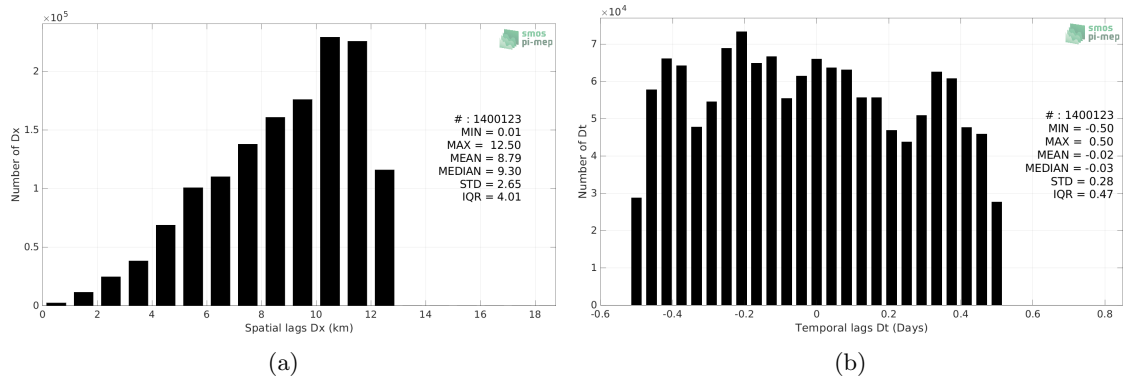
Figure 5: Histograms of the spatial (a) and temporal (b) lags between the location/time of the Salinity Snake (SPURS 2) measurement and the date of the corresponding SMOS SSS L3 v335 - 10 Days - 25 km (CATDS-CPDC) SSS pixel.
