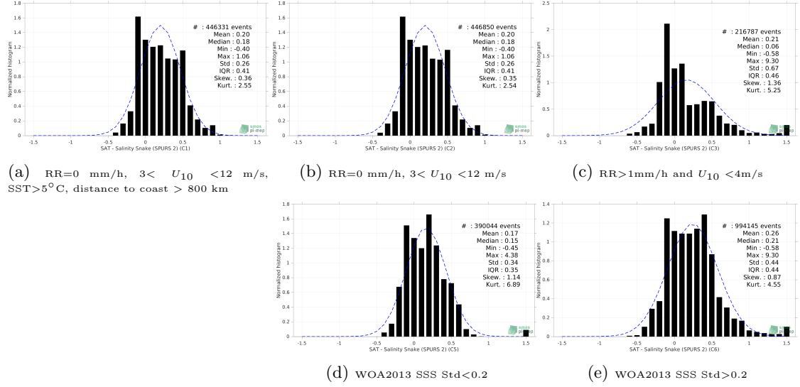
Figure 13: Normalized histogram of \Delta SSS (SMOS SSS L3 v335 - 10 Days - 25 km (CATDS-CPDC) - Salinity Snake (SPURS 2)) for 5 different subdatasets corresponding to: RR=0 mm/h, 3 < U_{10} < 12 m/s, SST>5°C, distance to coast > 800 km (a), RR=0 mm/h, 3 < U_{10} < 12 m/s (b), RR>1mm/h and U_{10} < 4 m/s (c), WOA2013 SSS Std<0.2 (d), WOA2013 SSS Std>0.2 (e).
