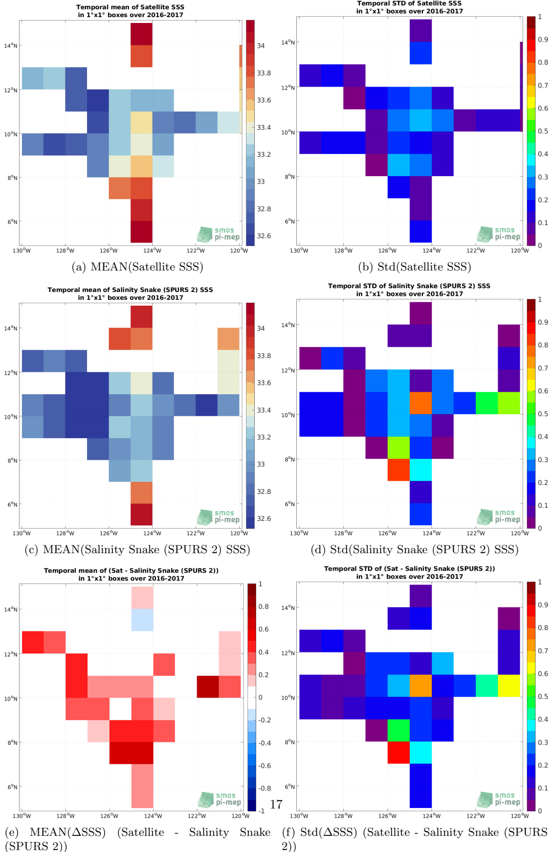
Figure 6: Temporal mean (left) and Std (right) of SSS from SMOS SSS L3 v335 - 10 Days - 25 km (CATDS-CPDC) (top), Salinity Snake (SPURS 2) (middle), and of \Delta SSS (Satellite - Salinity Snake (SPURS 2)). Only match-up pairs are used to generate these maps.
