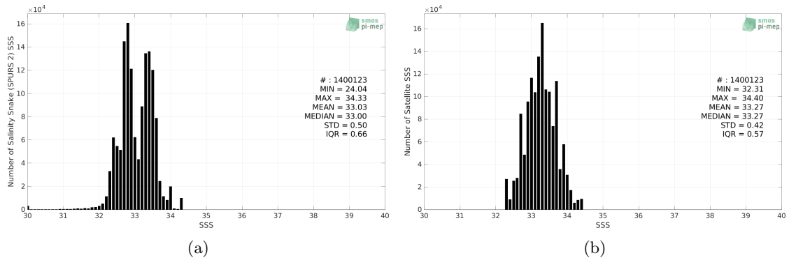
Figure 2: Histograms of SSS from Salinity Snake (SPURS 2) (a) and SMOS SSS L3 v335 - 10 Days - 25 km (CATDS-CPDC) (b) considering all match-up pairs per bins of 0.1 over the SPURS 2 Pi-MEP region and for the full satellite product period.
