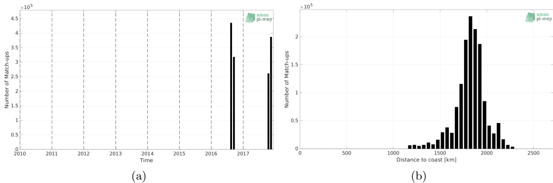
Figure 1: Number of match-ups between Salinity Snake (SPURS 2) and SMOS SSS L3 v335 - 10 Days - 25 km (CATDS-CPDC) SSS as a function of time (a) and as function of the distance to coast (b) over the SPURS 2 Pi-MEP region and for the full satellite product period.
