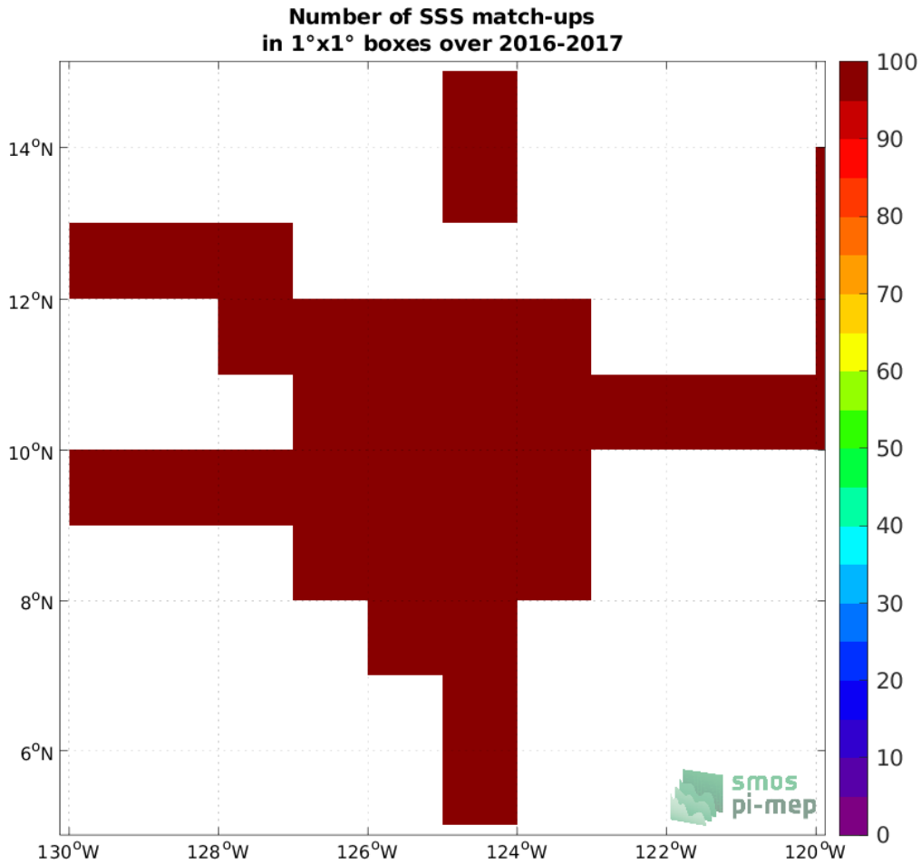
Figure 4: Number of SSS match-ups between Salinity Snake (SPURS 2) SSS and the SMOS SSS L3 v335 - 10 Days - 25 km (CATDS-CPDC) SSS product for the SPURS 2 Pi-MEP region over 1^\circ \times 1^\circ boxes and for the full satellite product period.
