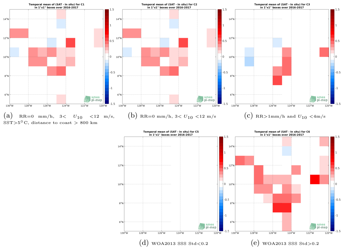
Figure 11: Temporal mean gridded over spatial boxes of size 1^\circ \times 1^\circ of \Delta SSS (SMOS SSS L3 v335 - 10 Days - 25 km (CATDS-CPDC) - Salinity Snake) for 5 different subdatasets corresponding to:RR=0 mm/h, 3 < U_{10} < 12 m/s, SST >5^\circ\text{C} , distance to coast > 800 km (a), RR=0 mm/h, 3 < U_{10} < 12 m/s (b), RR >1 mm/h and U_{10} < 4 m/s (c), WOA2013 SSS Std <0.2 (d), WOA2013 SSS Std >0.2 (e).
