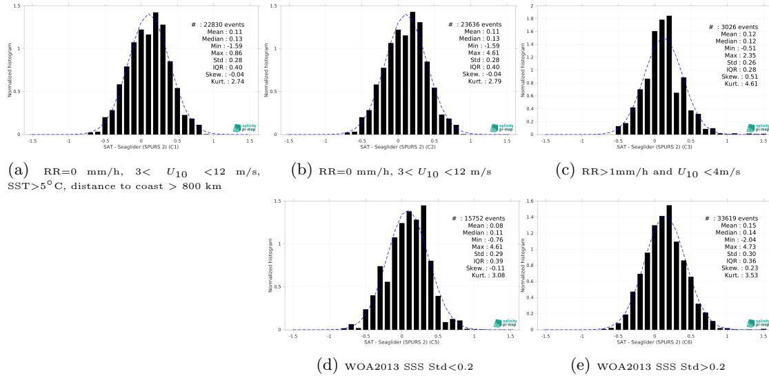
Figure 13: Normalized histogram of \Delta SSS (SMOS SSS L3 v335 - 10 Days - 25 km (CATDS-CPDC) - Seaglider (SPURS 2)) for 5 different subdatasets corresponding to: RR=0 mm/h, 3 < U_{10} < 12 m/s, SST>5°C, distance to coast > 800 km (a), RR=0 mm/h, 3 < U_{10} < 12 m/s (b), RR>1mm/h and U_{10} < 4 m/s (c), WOA2013 SSS Std<0.2 (d), WOA2013 SSS Std>0.2 (e).
