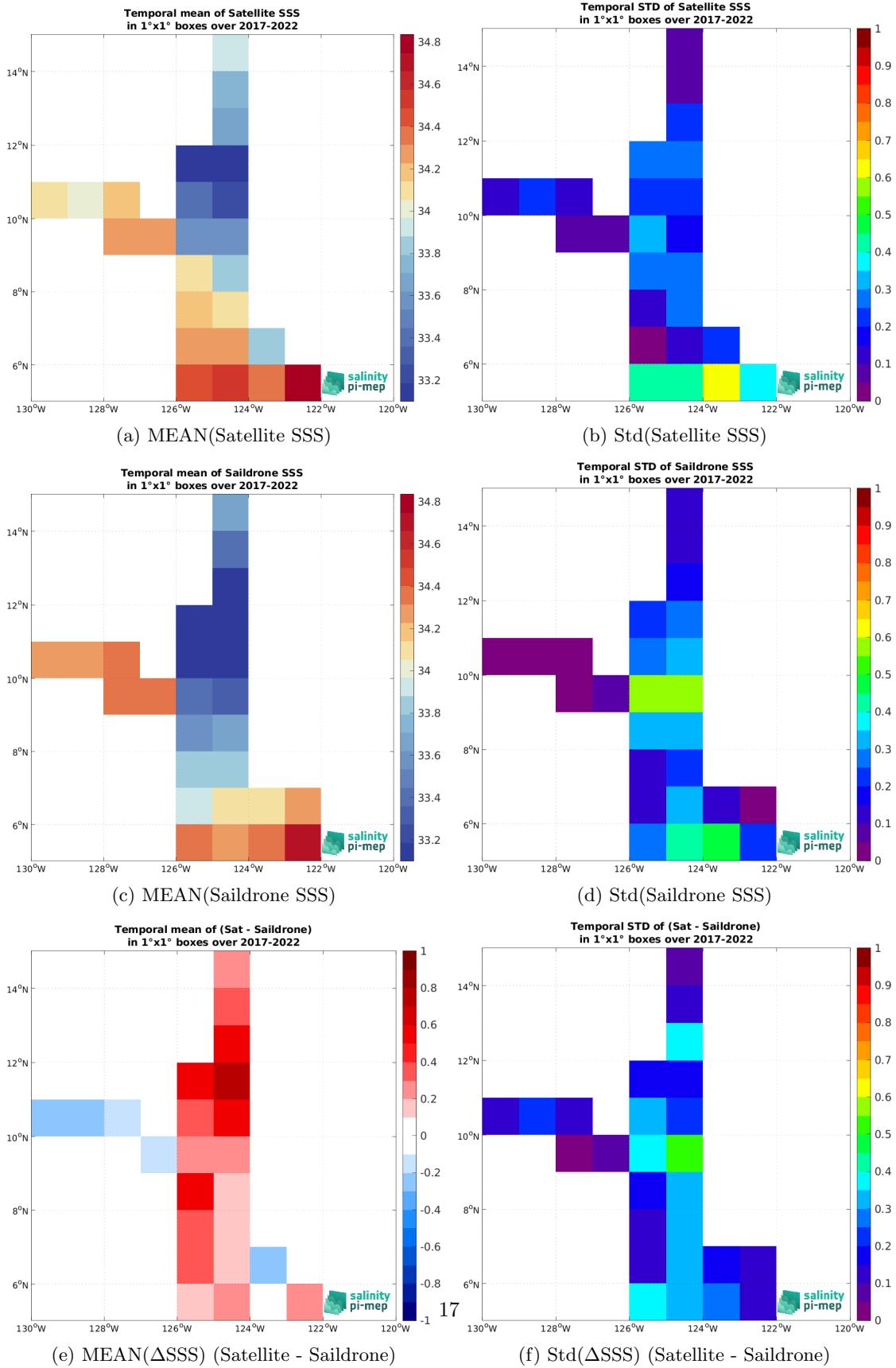
Figure 7: Temporal mean (left) and Std (right) of SSS from SMOS SSS L3 v335 - 10 Days - 25 km (CATDS-CPDC) (top), Saildrone (middle), and of \Delta SSS (Satellite - Saildrone). Only match-up pairs are used to generate these maps.
