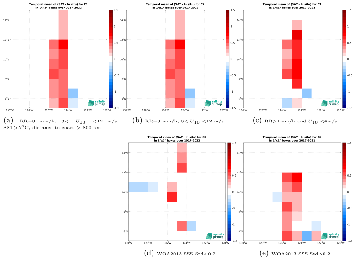
Figure 14: Temporal mean gridded over spatial boxes of size 1^\circ \times 1^\circ of \Delta SSS (SMOS SSS L3 v335 - 10 Days - 25 km (CATDS-CPDC) - Saildrone) for 5 different subdatasets corresponding to:RR=0 mm/h, 3 < U_{10} < 12 m/s, SST>5°C, distance to coast > 800 km (a), RR=0 mm/h, 3 < U_{10} < 12 m/s (b), RR>1mm/h and U_{10} < 4 m/s (c), WOA2013 SSS Std<0.2 (d), WOA2013 SSS Std>0.2 (e).
