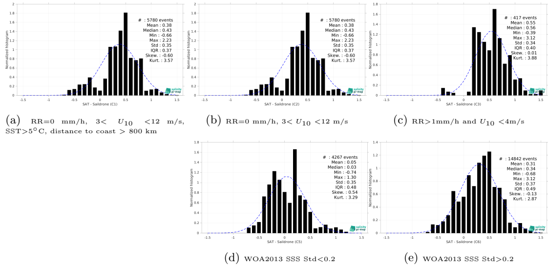
Figure 15: Normalized histogram of \Delta SSS (SMOS SSS L3 v335 - 10 Days - 25 km (CATDS-CPDC) - Saldrone) for 5 different subdatasets corresponding to: RR=0 mm/h, 3 < U_{10} < 12 m/s, SST > 5°C, distance to coast > 800 km (a), RR=0 mm/h, 3 < U_{10} < 12 m/s (b), RR > 1mm/h and U_{10} < 4 m/s (c), WOA2013 SSS Std < 0.2 (d), WOA2013 SSS Std > 0.2 (e).
