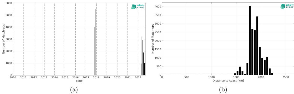
Figure 2: Number of match-ups between Saildrone and SMOS SSS L3 v335 - 10 Days - 25 km (CATDS-CPDC) SSS as a function of time (a) and as function of the distance to coast (b) over the SPURS 2 Pi-MEP region and for the full satellite product period.
