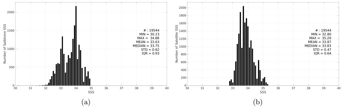
Figure 3: Histograms of SSS from Saildrone (a) and SMOS SSS L3 v335 - 10 Days - 25 km (CATDS-CPDC) (b) considering all match-up pairs per bins of 0.1 over the SPURS 2 Pi-MEP region and for the full satellite product period.
