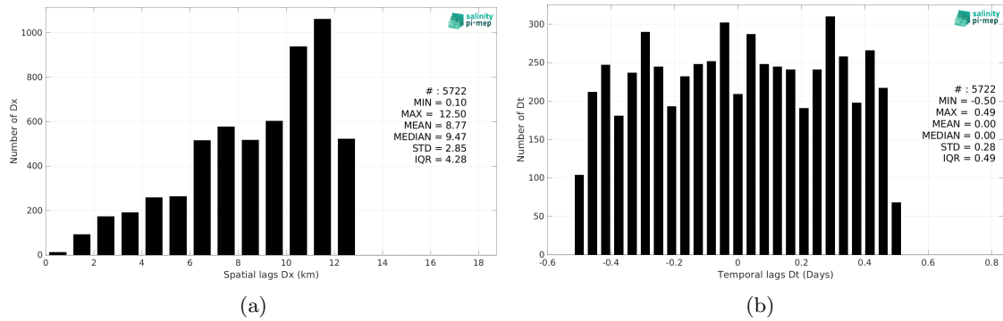
Figure 6: Histograms of the spatial (a) and temporal (b) lags between the location/time of the Saildrone (SPURS 2) measurement and the date of the corresponding SMOS SSS L3 v335 - 10 Days - 25 km (CATDS-CPDC) SSS pixel.
