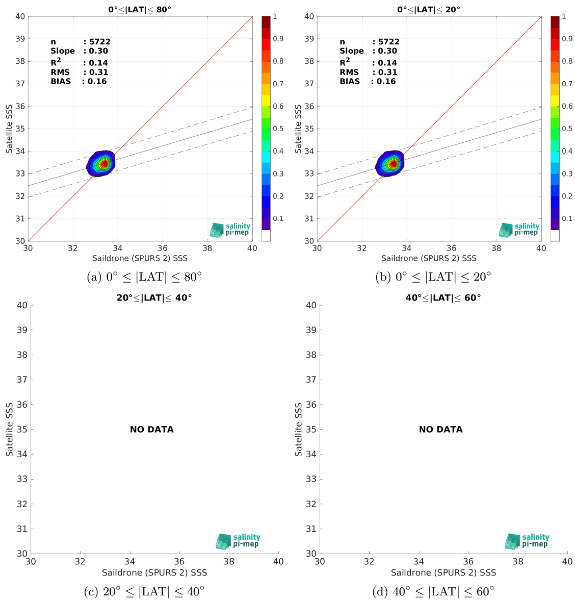
Figure 10: Contour maps of the concentration of SMOS SSS L3 v335 - 10 Days - 25 km (CATDS-CPDC) SSS (y-axis) versus Saildrone (SPURS 2) SSS (x-axis) at match-up pairs for different latitude bands. For each plot, the red line shows x=y . The black thin and dashed lines indicate a linear fit through the data cloud and the \pm 95\% confidence levels, respectively. The number match-up pairs n , the slope and R^2 coefficient of the linear fit, the root mean square (RMS) and the mean bias between satellite and in situ data are indicated for each latitude band in each plots.
