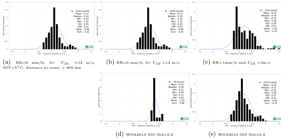
Figure 15: Normalized histogram of \Delta SSS (SMOS SSS L3 v335 - 10 Days - 25 km (CATDS-CPDC) - Saïdrone (SPURS 2)) for 5 different subdatasets corresponding to: RR=0 mm/h, 3 < U_{10} < 12 m/s, SST > 5°C, distance to coast > 800 km (a), RR=0 mm/h, 3 < U_{10} < 12 m/s (b), RR > 1mm/h and U_{10} < 4 m/s (c), WOA2013 SSS Std < 0.2 (d), WOA2013 SSS Std > 0.2 (e).
