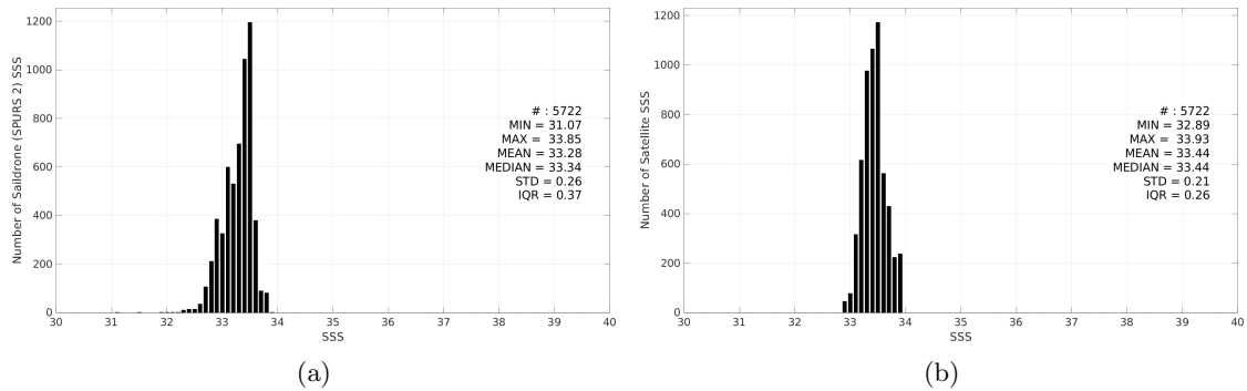
Figure 3: Histograms of SSS from Saildrone (SPURS 2) (a) and SMOS SSS L3 v335 - 10 Days - 25 km (CATDS-CPDC) (b) considering all match-up pairs per bins of 0.1 over the SPURS 2 Pi-MEP region and for the full satellite product period.
