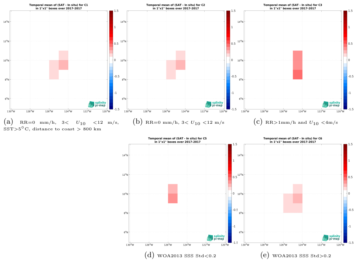
Figure 14: Temporal mean gridded over spatial boxes of size 1^\circ \times 1^\circ of \Delta SSS (SMOS SSS L3 v335 - 10 Days - 25 km (CATDS-CPDC) - Saildrone (SPURS 2)) for 5 different subdatasets corresponding to:RR=0 mm/h, 3 < U_{10} < 12 m/s, SST >5^\circ C, distance to coast > 800 km (a), RR=0 mm/h, 3 < U_{10} < 12 m/s (b), RR >1 mm/h and U_{10} < 4 m/s (c), WOA2013 SSS Std <0.2 (d), WOA2013 SSS Std >0.2 (e).
