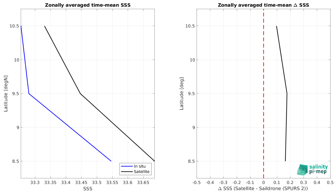
Figure 9: Left panel: Zonal mean SSS from SMOS SSS L3 v335 - 10 Days - 25 km (CATDS-CPDC) satellite product (black) and from Sairdron (SPURS 2) (blue). Right panel: Zonal mean of \Delta SSS (Satellite - Sairdron (SPURS 2)) for all the collected Pi-MEP match-up pairs estimated over the full satellite product period.
