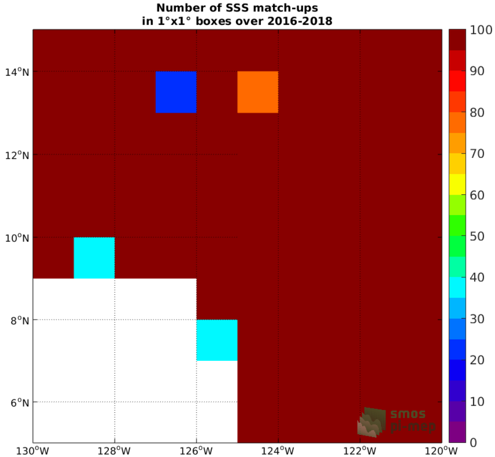
Figure 3: Number of SSS match-ups between Surface drifters SSS and the SMOS SSS L3 v335 - 10 Days - 25 km (CATDS-CPDC) SSS product for the SPURS 2 Pi-MEP region over 1^\circ \times 1^\circ boxes and for the full satellite product period.
