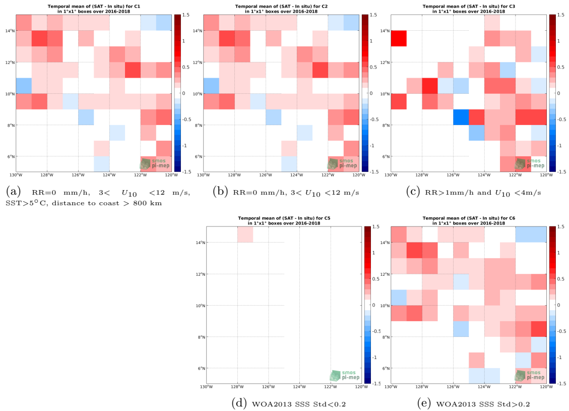
Figure 11: Temporal mean gridded over spatial boxes of size 1^\circ \times 1^\circ of \Delta\text{SSS} (SMOS SSS L3 v335 - 10 Days - 25 km (CATDS-CPDC) - Surface drifters) for 5 different subdatasets corresponding to: \text{RR}=0 mm/h, 3 < U_{10} < 12 m/s, \text{SST} > 5^\circ\text{C} , distance to coast > 800 km (a), \text{RR}=0 mm/h, 3 < U_{10} < 12 m/s (b), \text{RR} > 1\text{mm/h} and U_{10} < 4\text{m/s} (c), WOA2013 SSS Std < 0.2 (d), WOA2013 SSS Std > 0.2 (e).
