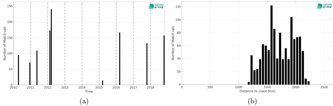
Figure 2: Number of match-ups between TSG (SAMOS) and SMOS SSS L2Q v333 - 0.25 Deg (CATDS-CPDC) SSS as a function of time (a) and as function of the distance to coast (b) over the SPURS 2 Pi-MEP region and for the full satellite product period.
