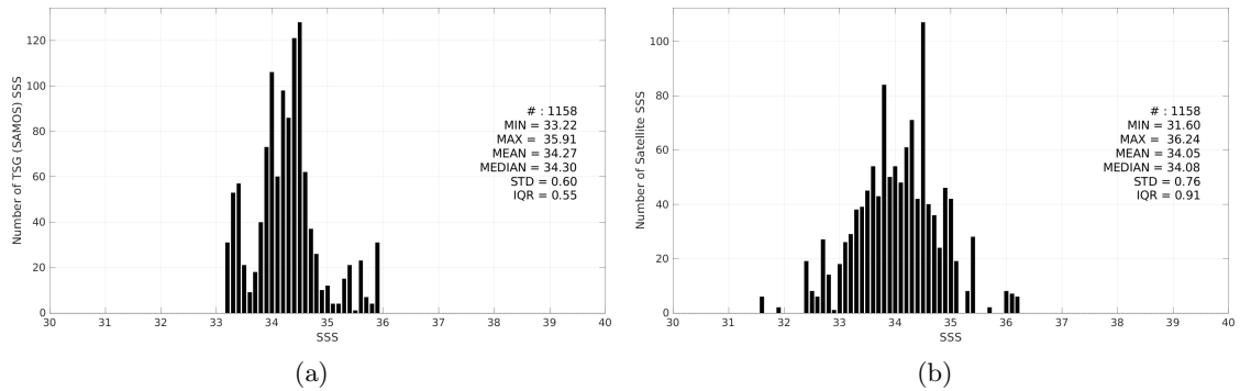
Figure 3: Histograms of SSS from TSG (SAMOS) (a) and SMOS SSS L2Q v333 - 0.25 Deg (CATDS-CPDC) (b) considering all match-up pairs per bins of 0.1 over the SPURS 2 Pi-MEP region and for the full satellite product period.
