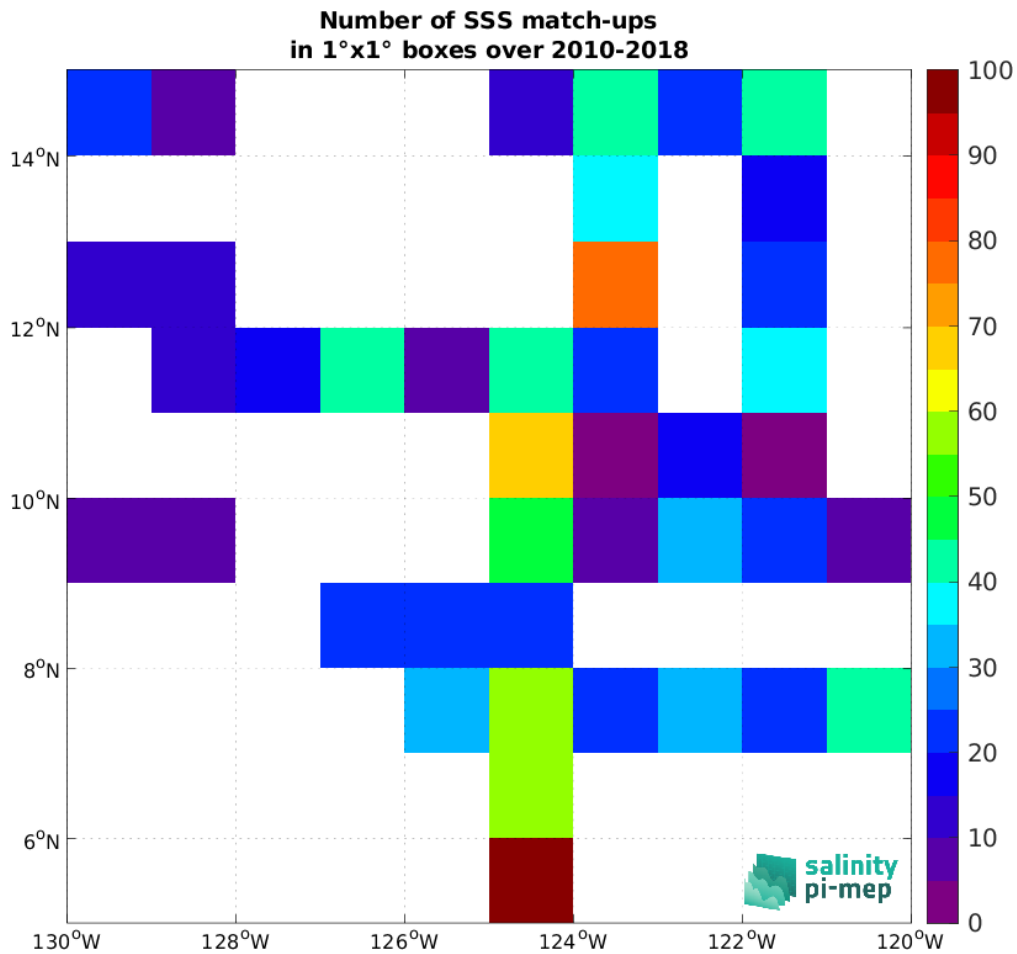
Figure 5: Number of SSS match-ups between TSG (SAMOS) SSS and the SMOS SSS L2Q v333 - 0.25 Deg (CATDS-CPDC) SSS product for the SPURS 2 Pi-MEP region over 1°x1° boxes and for the full satellite product period.
