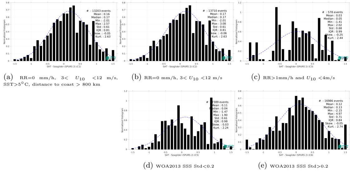
Figure 15: Normalized histogram of \Delta SSS (SMOS SSS L2Q v333 - 0.25 Deg (CATDS-CPDC) - Seaglider (SPURS 2)) for 5 different subdatasets corresponding to: RR=0 mm/h, 3 < U_{10} < 12 m/s, SST>5°C, distance to coast > 800 km (a), RR=0 mm/h, 3 < U_{10} < 12 m/s (b), RR>1mm/h and U_{10} < 4 m/s (c), WOA2013 SSS Std<0.2 (d), WOA2013 SSS Std>0.2 (e).
