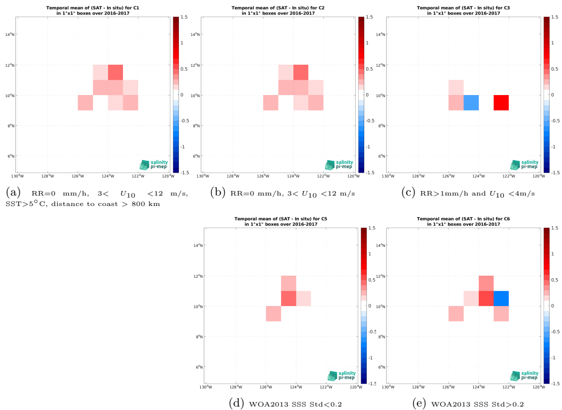
Figure 14: Temporal mean gridded over spatial boxes of size 1^\circ \times 1^\circ of \Delta SSS (SMOS SSS L2Q v333 - 0.25 Deg (CATDS-CPDC) - Seaglider (SPURS 2)) for 5 different subdatasets corresponding to:RR=0 mm/h, 3 < U_{10} < 12 m/s, SST >5^\circ C, distance to coast > 800 km (a), RR=0 mm/h, 3 < U_{10} < 12 m/s (b), RR >1 mm/h and U_{10} < 4 m/s (c), WOA2013 SSS Std <0.2 (d), WOA2013 SSS Std >0.2 (e).
