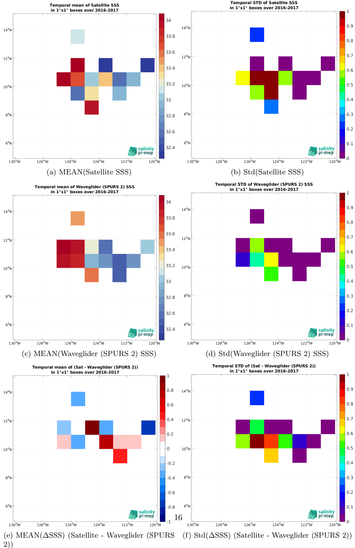
Figure 6: Temporal mean (left) and Std (right) of SSS from SMOS SSS L2Q v331 - 0.25 Deg (CATDS-CPDC) (top), Waveglider (SPURS 2) (middle), and of \Delta SSS (Satellite - Waveglider (SPURS 2)). Only match-up pairs are used to generate these maps.
