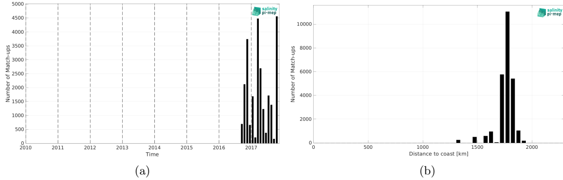
Figure 1: Number of match-ups between Waveglider (SPURS 2) and SMOS SSS L2Q v331 - 0.25 Deg (CATDS-CPDC) SSS as a function of time (a) and as function of the distance to coast (b) over the SPURS 2 Pi-MEP region and for the full satellite product period.
