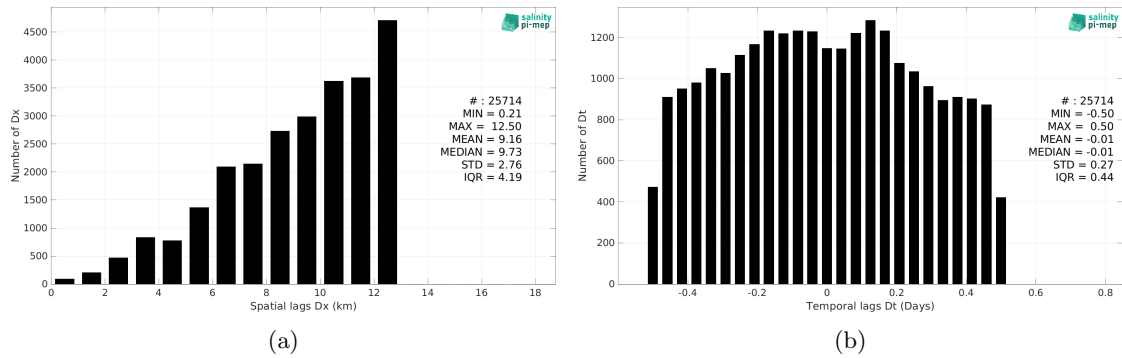
Figure 5: Histograms of the spatial (a) and temporal (b) lags between the location/time of the Waveglider (SPURS 2) measurement and the date of the corresponding SMOS SSS L2Q v331 - 0.25 Deg (CATDS-CPDC) SSS pixel.
