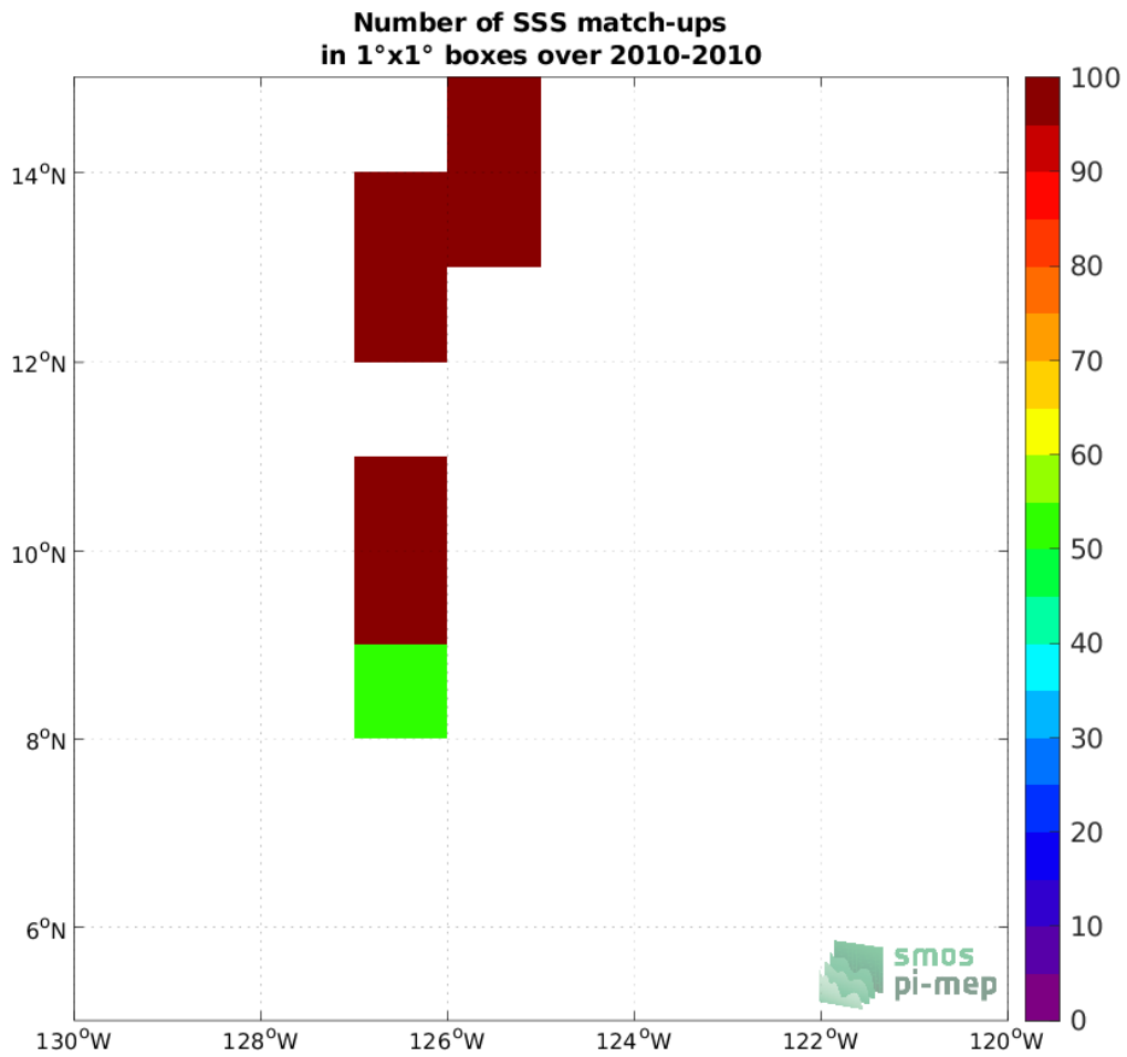
Figure 4: Number of SSS match-ups between TSG (GOSUD-Sailing-ship) SSS and the SMOS SSS L2Q v331 - 0.25 Deg (CATDS-CPDC) SSS product for the SPURS 2 Pi-MEP region over 1^\circ \times 1^\circ boxes and for the full satellite product period.
