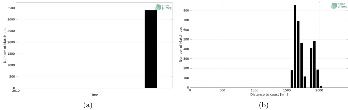
Figure 1: Number of match-ups between TSG (GOSUD-Sailing-ship) and SMOS SSS L2Q v331 - 0.25 Deg (CATDS-CPDC) SSS as a function of time (a) and as function of the distance to coast (b) over the SPURS 2 Pi-MEP region and for the full satellite product period.
