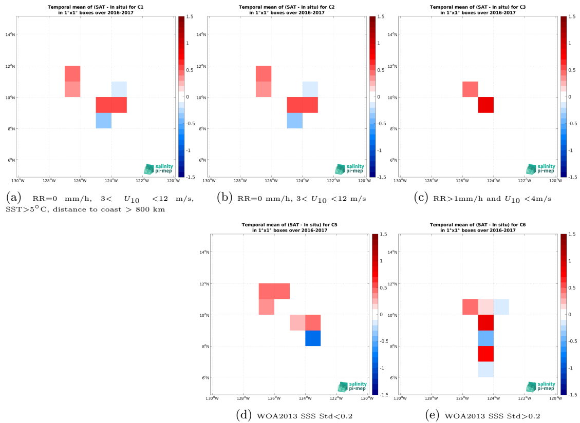
Figure 12: Temporal mean gridded over spatial boxes of size 1^\circ \times 1^\circ of \Delta\text{SSS} (SMOS SSS L2Q v331 - 0.25 Deg (CATDS-CPDC) - Salinity Snake (SPURS 2)) for 5 different subdatasets corresponding to:RR=0 mm/h, 3 < U_{10} < 12 m/s, SST >5^\circ\text{C} , distance to coast > 800 km (a), RR=0 mm/h, 3 < U_{10} < 12 m/s (b), RR >1 mm/h and U_{10} < 4 m/s (c), WOA2013 SSS Std <0.2 (d), WOA2013 SSS Std >0.2 (e).
