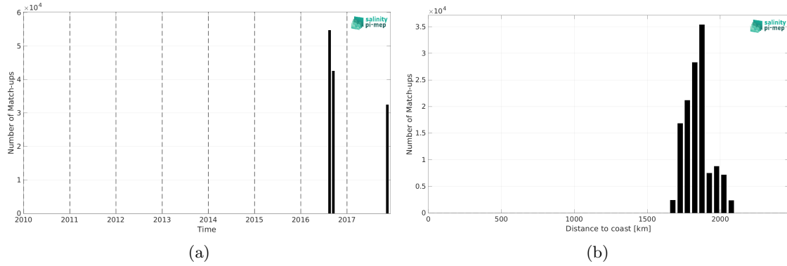
Figure 1: Number of match-ups between Salinity Snake (SPURS 2) and SMOS SSS L2Q v331 - 0.25 Deg (CATDS-CPDC) SSS as a function of time (a) and as function of the distance to coast (b) over the SPURS 2 Pi-MEP region and for the full satellite product period.
