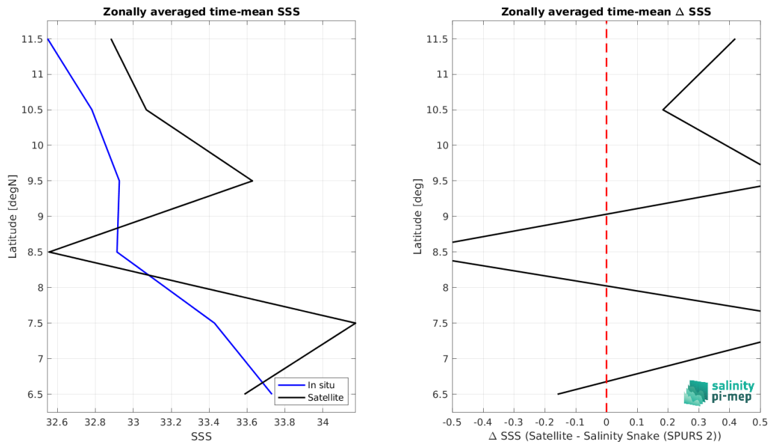
Figure 8: Left panel: Zonal mean SSS from SMOS SSS L2Q v331 - 0.25 Deg (CATDS-CPDC) satellite product (black) and from Salinity Snake (SPURS 2) (blue). Right panel: Zonal mean of \Delta SSS (Satellite - Salinity Snake (SPURS 2)) for all the collected Pi-MEP match-up pairs estimated over the full satellite product period.
