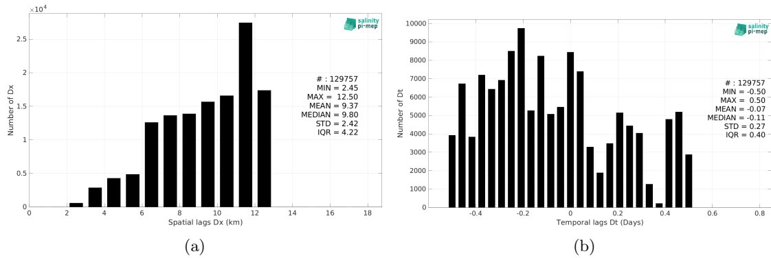
Figure 5: Histograms of the spatial (a) and temporal (b) lags between the location/time of the Salinity Snake (SPURS 2) measurement and the date of the corresponding SMOS SSS L2Q v331 - 0.25 Deg (CATDS-CPDC) SSS pixel.
