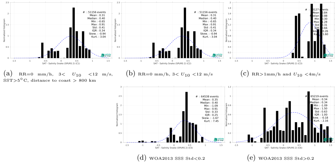
Figure 13: Normalized histogram of \Delta SSS (SMOS SSS L2Q v331 - 0.25 Deg (CATDS-CPDC) - Salinity Snake (SPURS 2)) for 5 different subdatasets corresponding to: RR=0 mm/h, 3 < U_{10} < 12 m/s, SST > 5°C, distance to coast > 800 km (a), RR=0 mm/h, 3 < U_{10} < 12 m/s (b), RR > 1mm/h and U_{10} < 4 m/s (c), WOA2013 SSS Std < 0.2 (d), WOA2013 SSS Std > 0.2 (e).
