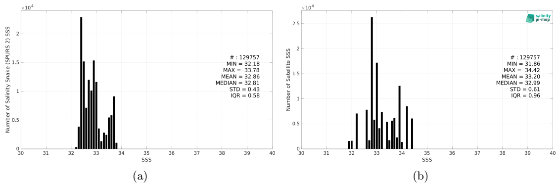
Figure 2: Histograms of SSS from Salinity Snake (SPURS 2) (a) and SMOS SSS L2Q v331 - 0.25 Deg (CATDS-CPDC) (b) considering all match-up pairs per bins of 0.1 over the SPURS 2 Pi-MEP region and for the full satellite product period.
