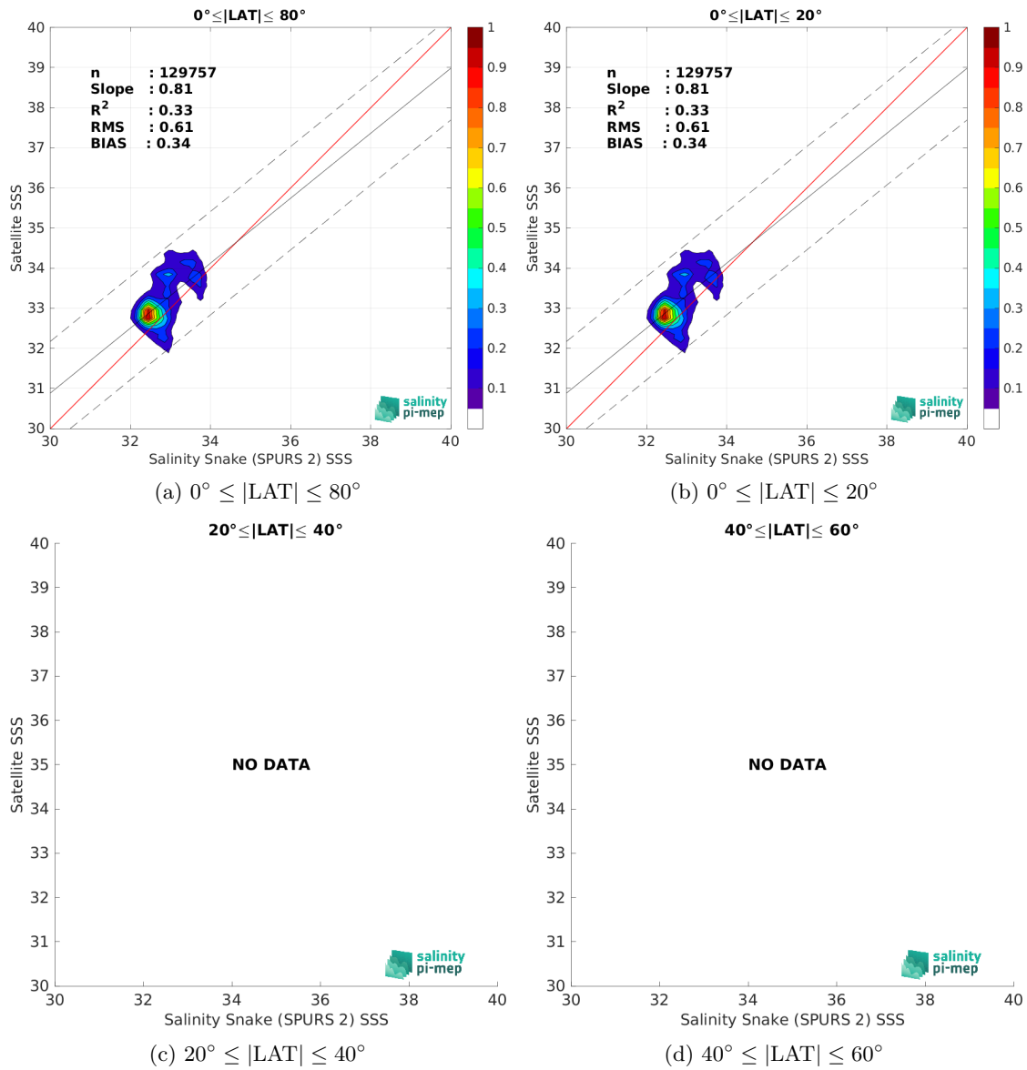
Figure 9: Contour maps of the concentration of SMOS SSS L2Q v331 - 0.25 Deg (CATDS-CPDC) SSS (y-axis) versus Salinity Snake (SPURS 2) SSS (x-axis) at match-up pairs for different latitude bands. For each plot, the red line shows x=y . The black thin and dashed lines indicate a linear fit through the data cloud and the \pm 95\% confidence levels, respectively. The number match-up pairs n , the slope and R^2 coefficient of the linear fit, the root mean square (RMS) and the mean bias between satellite and in situ data are indicated for each latitude band in each plots.
