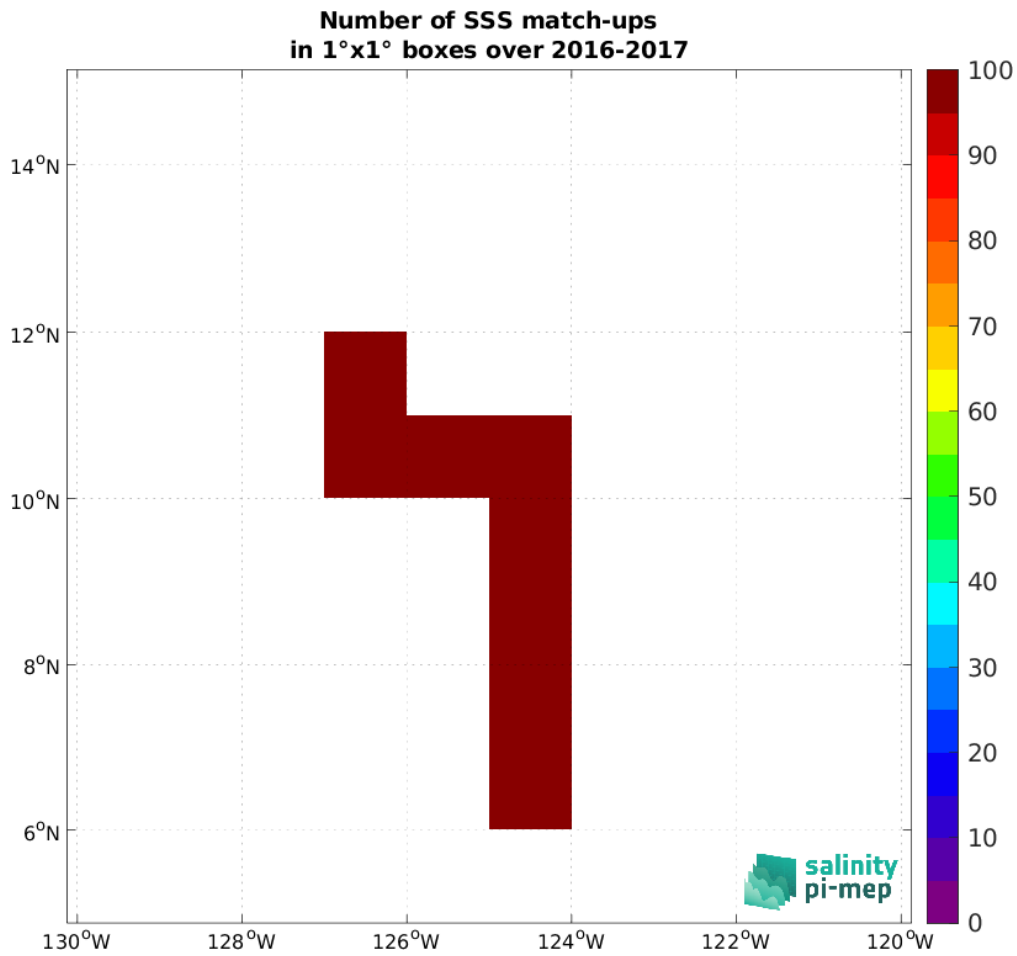
Figure 4: Number of SSS match-ups between Salinity Snake (SPURS 2) SSS and the SMOS SSS L2Q v331 - 0.25 Deg (CATDS-CPDC) SSS product for the SPURS 2 Pi-MEP region over 1^\circ \times 1^\circ boxes and for the full satellite product period.
