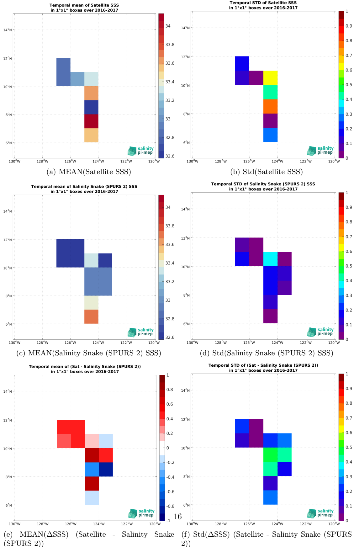
Figure 6: Temporal mean (left) and Std (right) of SSS from SMOS SSS L2Q v331 - 0.25 Deg (CATDS-CPDC) (top), Salinity Snake (SPURS 2) (middle), and of \Delta SSS (Satellite - Salinity Snake (SPURS 2)). Only match-up pairs are used to generate these maps.
