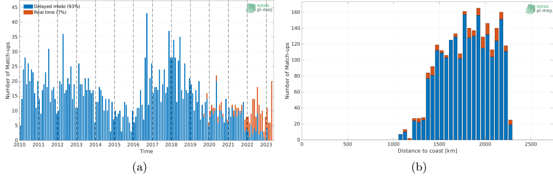
Figure 1: Number of match-ups between Argo and SMOS SSS L2Q v331 - 0.25 Deg (CATDS-CPDC) SSS as a function of time (a) and as function of the distance to coast (b) over the SPURS 2 Pi-MEP region and for the full satellite product period.
