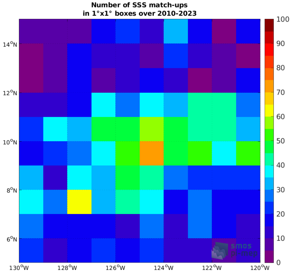
Figure 4: Number of SSS match-ups between Argo SSS and the SMOS SSS L2Q v331 - 0.25 Deg (CATDS-CPDC) SSS product for the SPURS 2 Pi-MEP region over 1°x1° boxes and for the full satellite product period.
