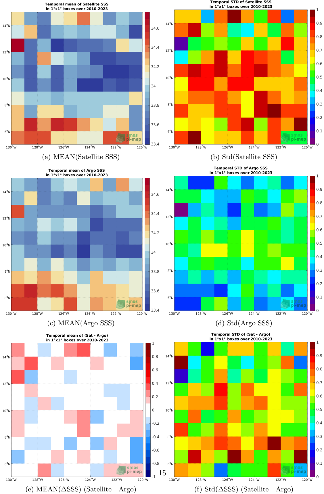
Figure 6: Temporal mean (left) and Std (right) of SSS from SMOS SSS L2Q v331 - 0.25 Deg (CATDS-CPDC) (top), Argo (middle), and of \Delta SSS (Satellite - Argo). Only match-up pairs are used to generate these maps.
