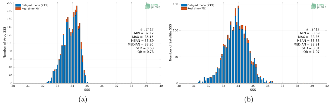
Figure 2: Histograms of SSS from Argo (a) and SMOS SSS L2Q v331 - 0.25 Deg (CATDS-CPDC) (b) considering all match-up pairs per bins of 0.1 over the SPURS 2 Pi-MEP region and for the full satellite product period.
