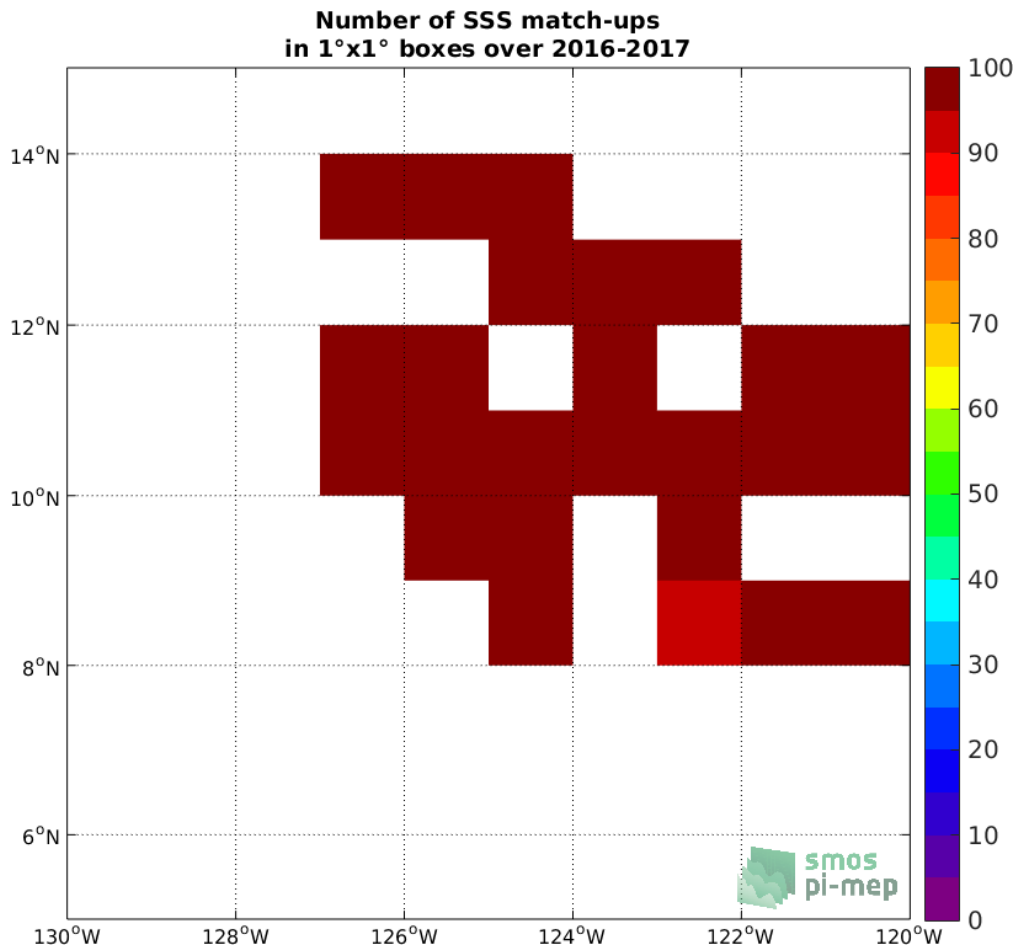
Figure 3: Number of SSS match-ups between Waveglider SSS and the SMOS SSS L2Q v321 - 0.25 Deg (CATDS-CPDC) SSS product for the SPURS 2 Pi-MEP region over 1°×1° boxes and for the full satellite product period.
