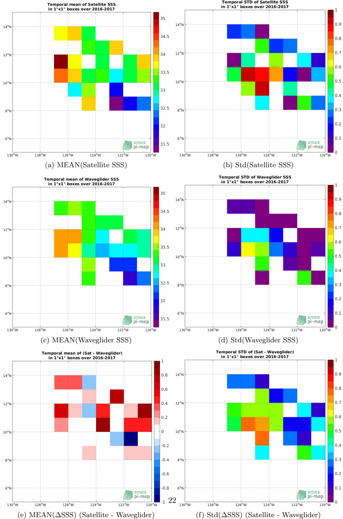
Figure 5: Temporal mean (left) and Std (right) of SSS from SMOS SSS L2Q v321 - 0.25 Deg (CATDS-CPDC) (top), Waveglider (middle), and of \Delta SSS (Satellite - Waveglider). Only match-pairs are used to generate these maps.
