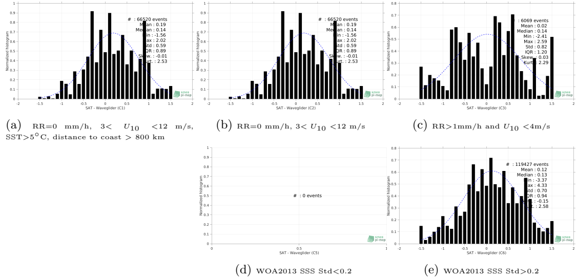
Figure 12: Normalized histogram of \Delta SSS (SMOS SSS L2Q v321 - 0.25 Deg (CATDS-CPDC) - Waveglider) for 5 different subdatasets corresponding to: RR=0 mm/h, 3 < U_{10} < 12 m/s, SST > 5°C, distance to coast > 800 km (a), RR=0 mm/h, 3 < U_{10} < 12 m/s (b), RR > 1mm/h and U_{10} < 4 m/s (c), WOA2013 SSS Std < 0.2 (d), WOA2013 SSS Std > 0.2 (e).
