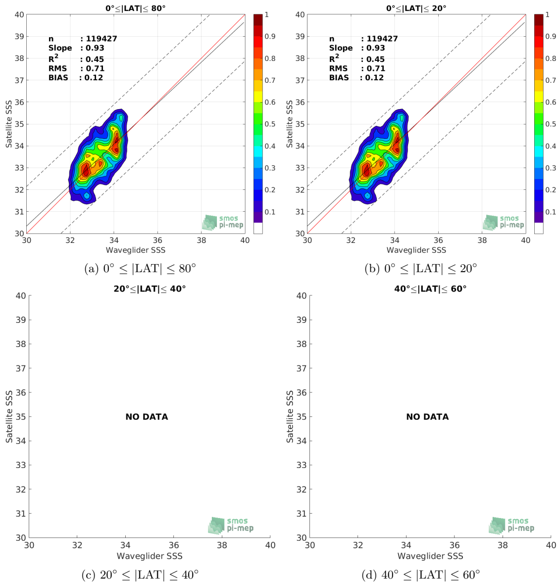
Figure 8: Contour maps of the concentration of SMOS SSS L2Q v321 - 0.25 Deg (CATDS-CPDC) SSS (y-axis) versus Waveglider SSS (x-axis) at match-up pairs for different latitude bands. For each plot, the red line shows x=y . The black thin and dashed lines indicate a linear fit through the data cloud and the \pm 95\% confidence levels, respectively. The number match-up pairs n , the slope and R^2 coefficient of the linear fit, the root mean square (RMS) and the mean bias between satellite and in situ data are indicated for each latitude band in each plots.
