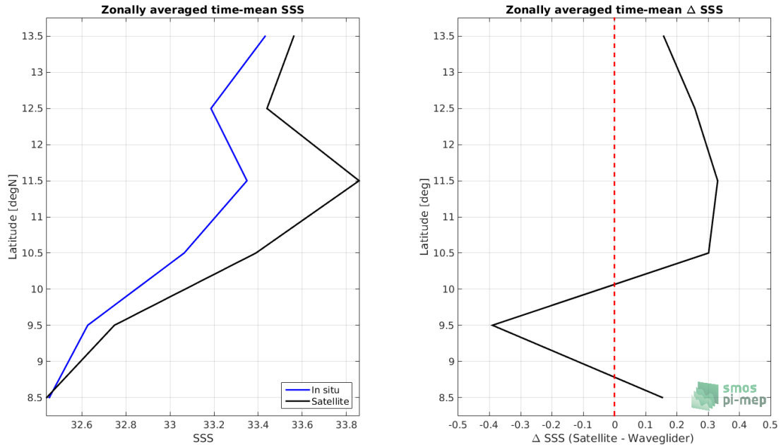
Figure 7: Left panel: Zonal mean SSS from SMOS SSS L2Q v321 - 0.25 Deg (CATDS-CPDC) satellite product (black) and from Waveglider (blue). Right panel: Zonal mean of \Delta SSS (Satellite - Waveglider) for all the collected Pi-MEP match-up pairs estimated over the full satellite product period.
