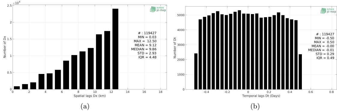
Figure 4: Histograms of the spatial (a) and temporal (b) lags between the location/time of the Waveglider measurement and the date of the corresponding SMOS SSS L2Q v321 - 0.25 Deg (CATDS-CPDC) SSS pixel.
