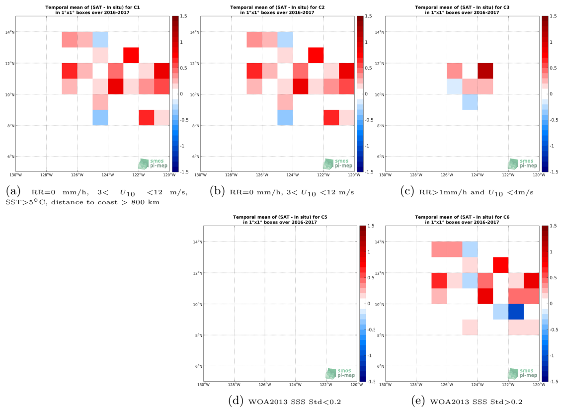
Figure 11: Temporal mean gridded over spatial boxes of size 1^\circ \times 1^\circ of \Delta SSS (SMOS SSS L2Q v321 - 0.25 Deg (CATDS-CPDC) - Waveglider) for 5 different subdatasets corresponding to:RR=0 mm/h, 3 < U_{10} < 12 m/s, SST >5^\circ\text{C} , distance to coast > 800 km (a), RR=0 mm/h, 3 < U_{10} < 12 m/s (b), RR >1 mm/h and U_{10} < 4 m/s (c), WOA2013 SSS Std <0.2 (d), WOA2013 SSS Std >0.2 (e).
