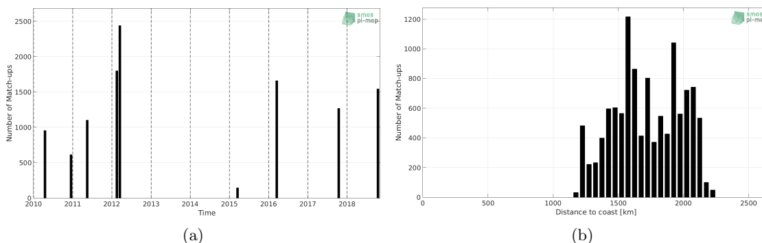
Figure 1: Number of match-ups between TSG-SAMOS and SMOS L2Q v321 - 0.25 Deg (CATDS-CPDC) SSS as a function of time (a) and as function of the distance to coast (b) over the SPURS 2 Pi-MEP region and for the full satellite product period.
