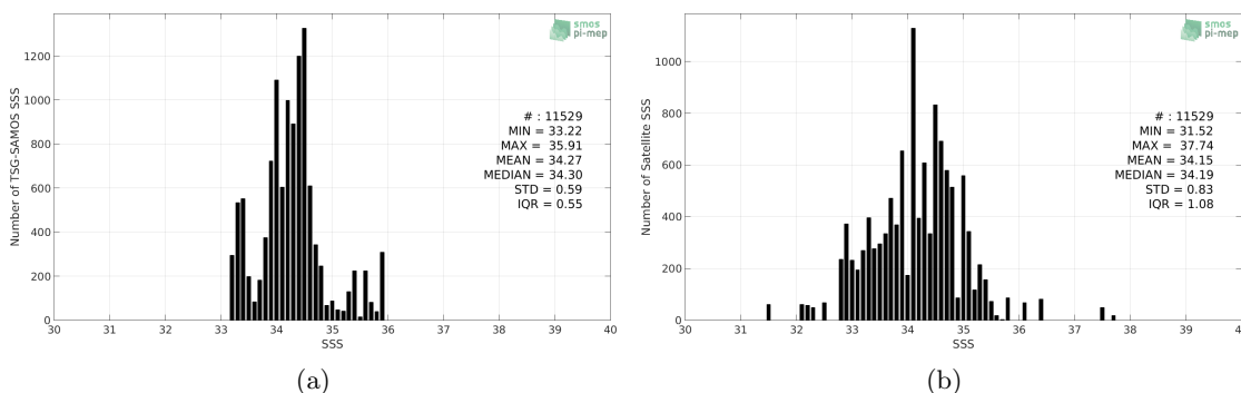
Figure 2: Histograms of SSS from TSG-SAMOS (a) and SMOS L2Q v321 - 0.25 Deg (CATDS-CPDC) (b) considering all match-up pairs per bins of 0.1 over the SPURS 2 Pi-MEP region and for the full satellite product period.
