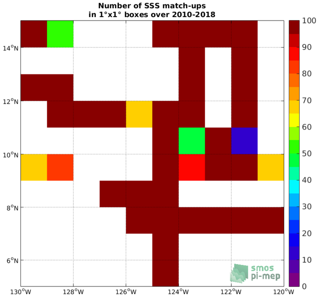
Figure 4: Number of SSS match-ups between TSG-SAMOS SSS and the SMOS L2Q v321 - 0.25 Deg (CATDS-CPDC) SSS product for the SPURS 2 Pi-MEP region over 1°x1° boxes and for the full satellite product period.
