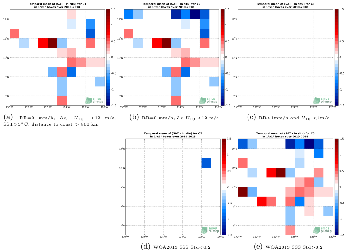
Figure 12: Temporal mean gridded over spatial boxes of size 1^\circ \times 1^\circ of \Delta SSS (SMOS L2Q v321 - 0.25 Deg (CATDS-CPDC) - TSG-SAMOS) for 5 different subdatasets corresponding to: RR=0 mm/h, 3 < U_{10} < 12 m/s, SST > 5^\circ C , distance to coast > 800 km (a), RR=0 mm/h, 3 < U_{10} < 12 m/s (b), RR > 1 mm/h and U_{10} < 4 m/s (c), WOA2013 SSS Std < 0.2 (d), WOA2013 SSS Std > 0.2 (e).
