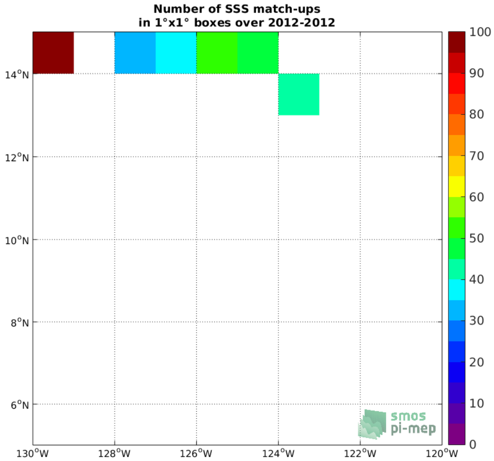
Figure 4: Number of SSS match-ups between TSG-GOSUD-Research-vessel SSS and the SMOS-L3-CATDS-CPDC-V321-L2Q SSS product for the SPURS 2 Pi-MEP region over 1°x1° boxes and for the full satellite product period.
