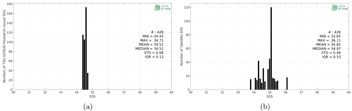
Figure 2: Histograms of SSS from TSG-GOSUD-Research-vessel (a) and SMOS-L3-CATDS-CPDC-V321-L2Q (b) considering all match-up pairs per bins of 0.1 over the SPURS 2 Pi-MEP region and for the full satellite product period.
