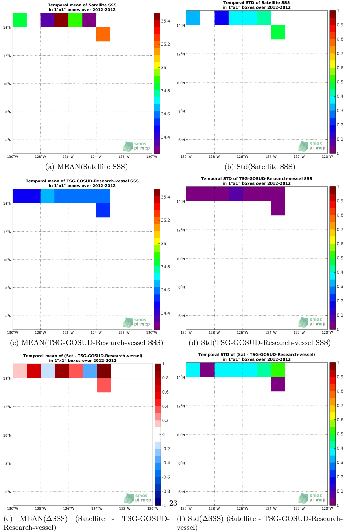
Figure 6: Temporal mean (left) and Std (right) of SSS from SMOS-L3-CATDS-CPDC-V321-L2Q (top), TSG-GOSUD-Research-vessel (middle), and of \Delta SSS (Satellite - TSG-GOSUD-Research-vessel). Only match-up pairs are used to generate these maps.
