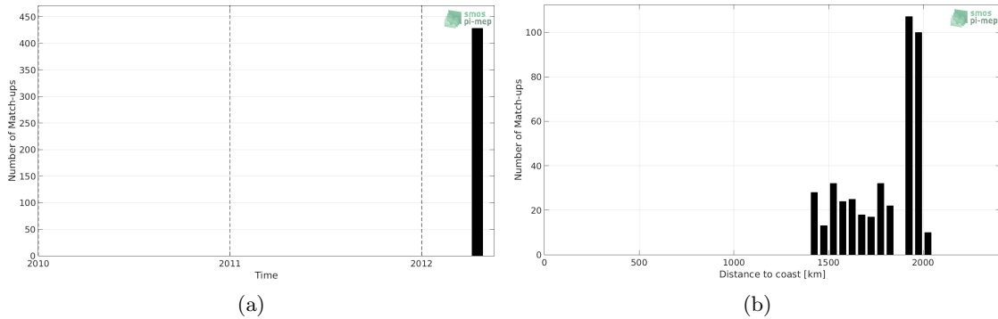
Figure 1: Number of match-ups between TSG-GOSUD-Research-vessel and SMOS-L3-CATDS-CPDC-V321-L2Q SSS as a function of time (a) and as function of the distance to coast (b) over the SPURS 2 Pi-MEP region and for the full satellite product period.
