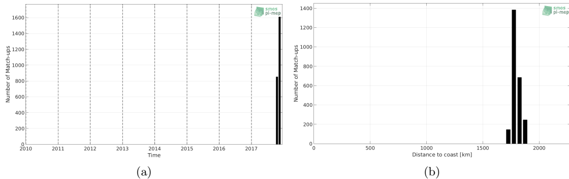
Figure 1: Number of match-ups between Saildrone and SMOS SSS L2Q v321 - 0.25 Deg (CATDS-CPDC) SSS as a function of time (a) and as function of the distance to coast (b) over the SPURS 2 Pi-MEP region and for the full satellite product period.
