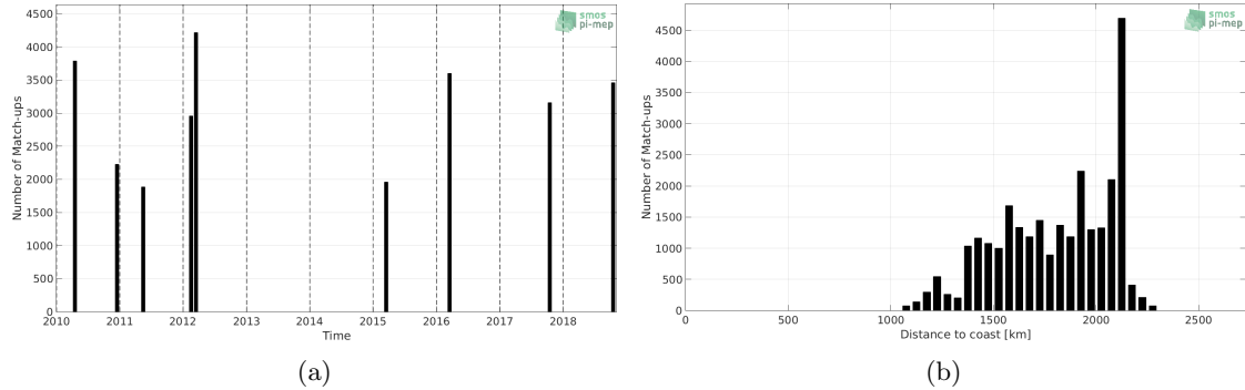
Figure 1: Number of match-ups between TSG-SAMOS and SMOS L3 v317 - Monthly - 25 km (CATDS-CPDC) SSS as a function of time (a) and as function of the distance to coast (b) over the SPURS 2 Pi-MEP region and for the full satellite product period.
