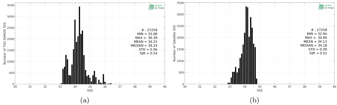
Figure 2: Histograms of SSS from TSG-SAMOS (a) and SMOS L3 v317 - Monthly - 25 km (CATDS-CPDC) (b) considering all match-up pairs per bins of 0.1 over the SPURS 2 Pi-MEP region and for the full satellite product period.
