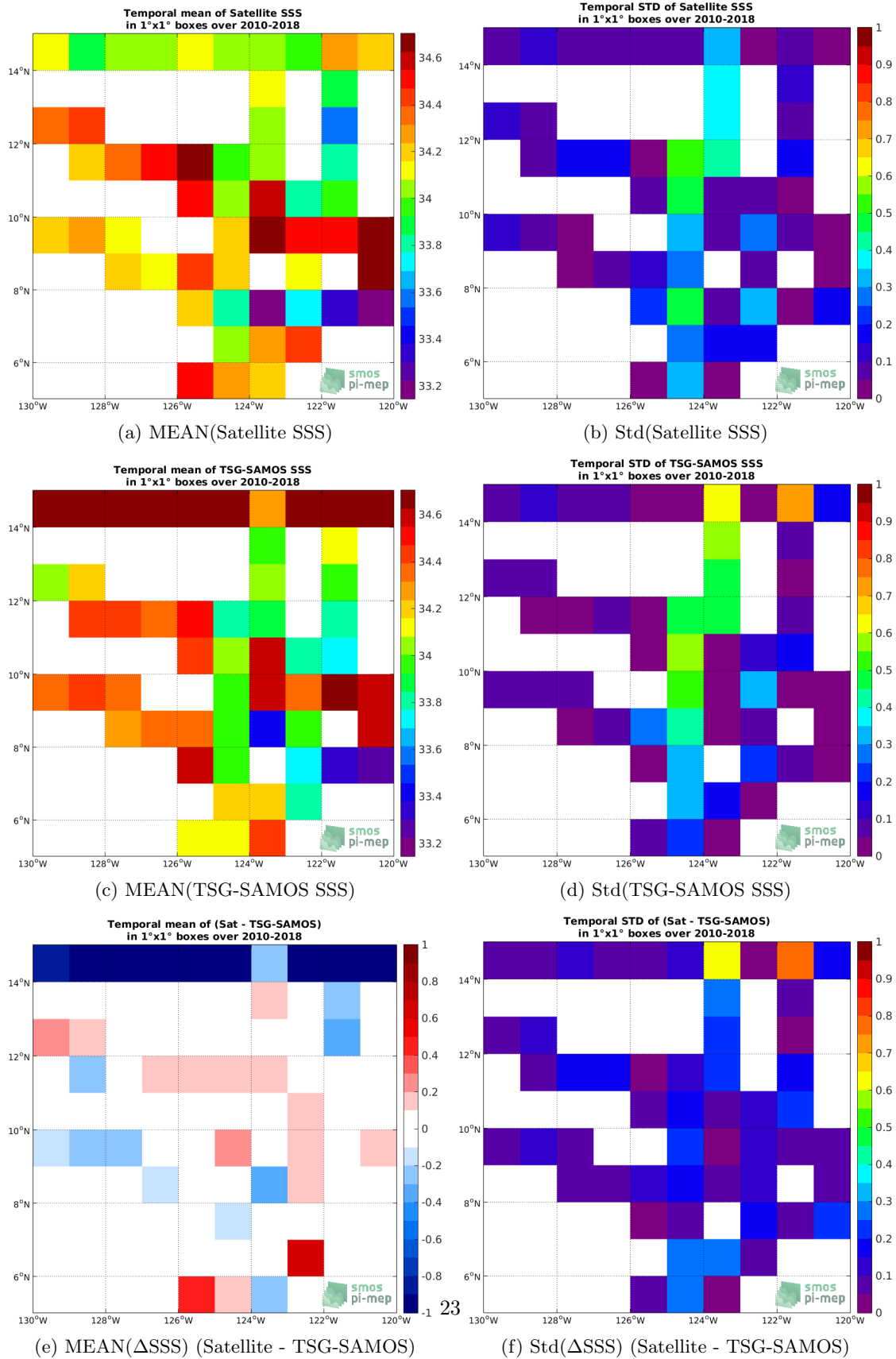
Figure 6: Temporal mean (left) and Std (right) of SSS from SMOS L3 v317 - Monthly - 25 km (CATDS-CPDC) (top), TSG-SAMOS (middle), and of \Delta SSS (Satellite - TSG-SAMOS). Only match-up pairs are used to generate these maps.
