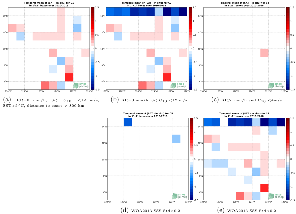
Figure 12: Temporal mean gridded over spatial boxes of size 1^\circ \times 1^\circ of \Delta SSS (SMOS-L3-CATDS-CPDC-V317-MONTHLY-25KM - TSG-SAMOS) for 5 different subdatasets corresponding to: RR=0 mm/h, 3 < U_{10} < 12 m/s, SST > 5^\circ C , distance to coast > 800 km (a), RR=0 mm/h, 3 < U_{10} < 12 m/s (b), RR > 1 mm/h and U_{10} < 4 m/s (c), WOA2013 SSS Std < 0.2 (d), WOA2013 SSS Std > 0.2 (e).
