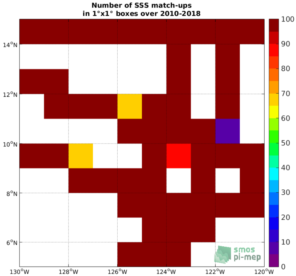
Figure 4: Number of SSS match-ups between TSG-SAMOS SSS and the SMOS-L3-CATDS-CPDC-V317-MONTHLY-25KM SSS product for the SPURS 2 Pi-MEP region over 1°x1° boxes and for the full satellite product period.
