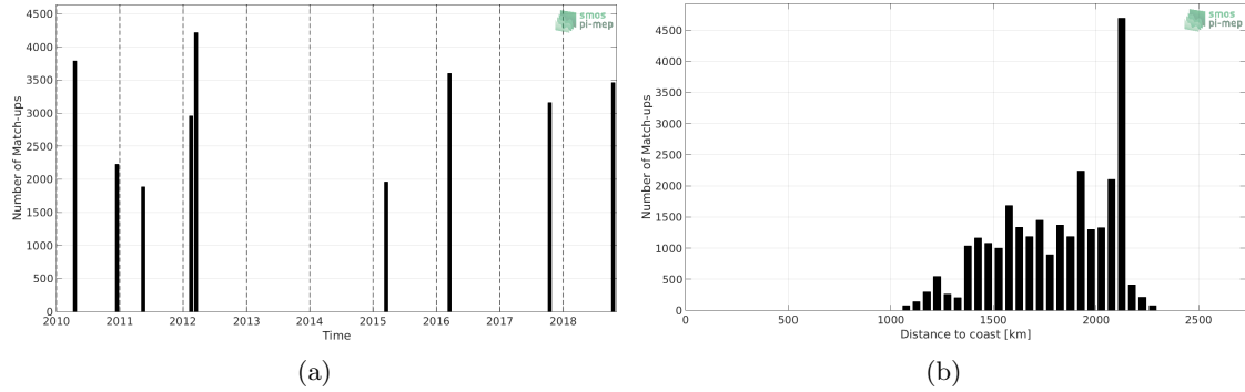
Figure 1: Number of match-ups between TSG-SAMOS and SMOS-L3-CATDS-CPDC-V317-MONTHLY-25KM SSS as a function of time (a) and as function of the distance to coast (b) over the SPURS 2 Pi-MEP region and for the full satellite product period.
