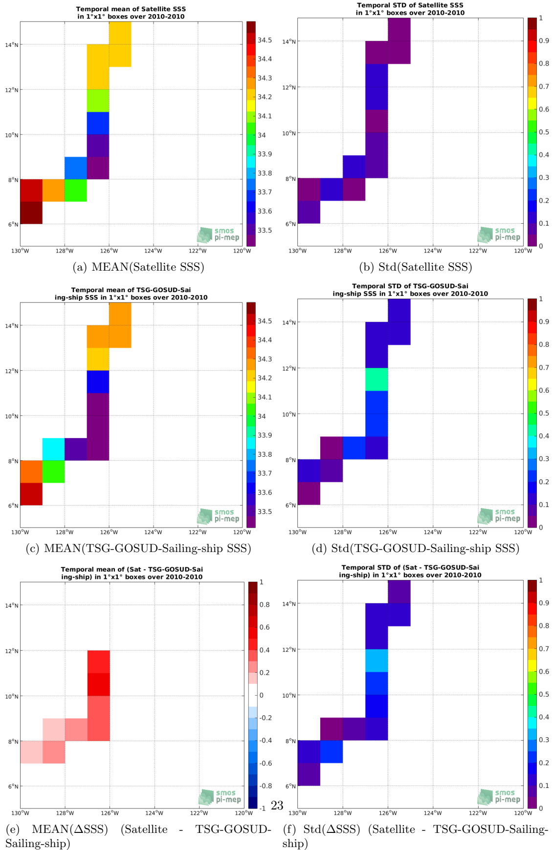
Figure 6: Temporal mean (left) and Std (right) of SSS from SMOS L3 v317 - Monthly - 25 km (CATDS-CPDC) (top), TSG-GOSUD-Sailing-ship (middle), and of \Delta SSS (Satellite - TSG-GOSUD-Sailing-ship). Only match-up pairs are used to generate these maps.
