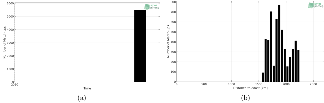
Figure 1: Number of match-ups between TSG-GOSUD-Sailing-ship and SMOS L3 v317 - Monthly - 25 km (CATDS-CPDC) SSS as a function of time (a) and as function of the distance to coast (b) over the SPURS 2 Pi-MEP region and for the full satellite product period.
