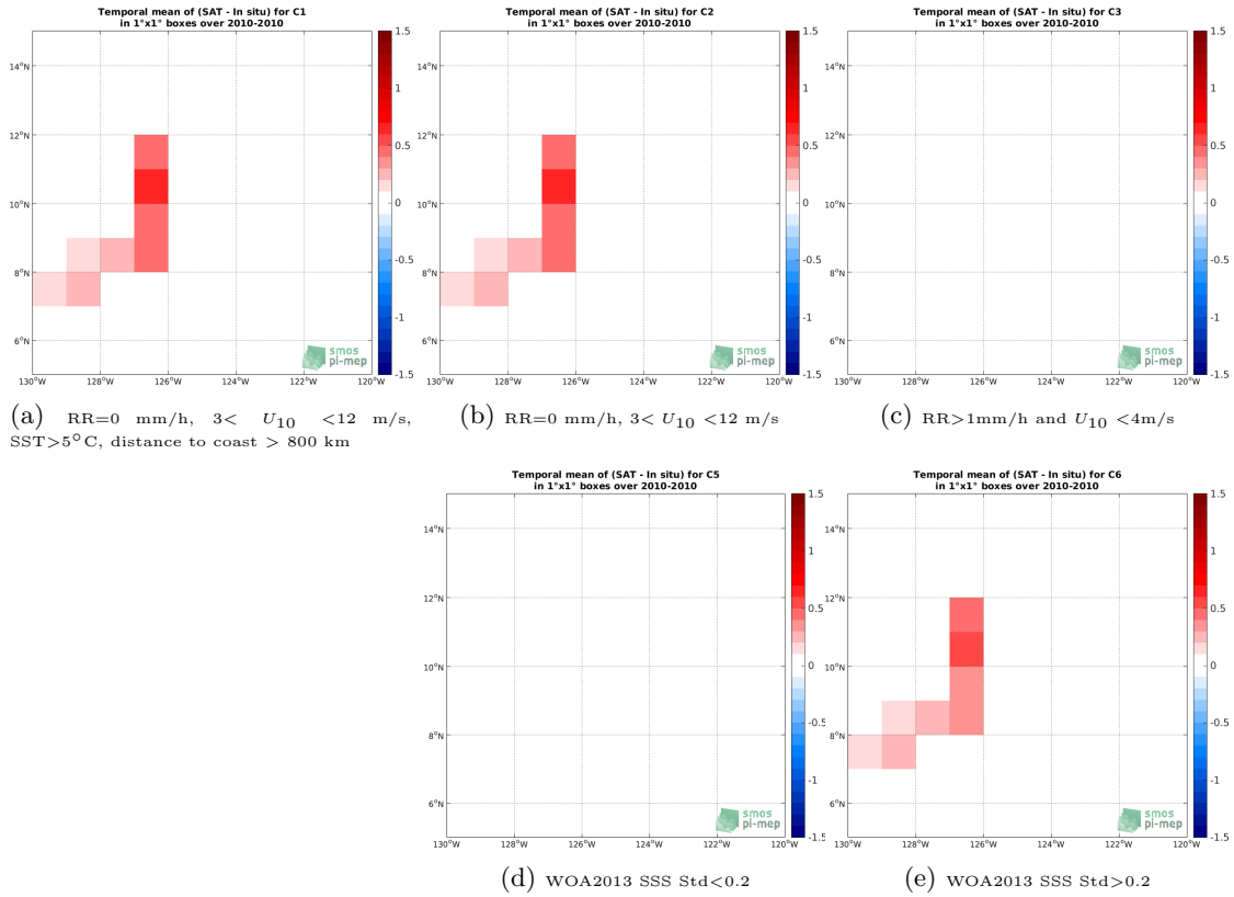
Figure 12: Temporal mean gridded over spatial boxes of size 1°x1° of \Delta SSS (SMOS L3 v317 - Monthly - 25 km (CATDS-CPDC) - TSG-GOSUD-Sailing-ship) for 5 different subdatasets corresponding to:RR=0 mm/h, 3 < U_{10} < 12 m/s, SST>5°C, distance to coast > 800 km (a), RR=0 mm/h, 3 < U_{10} < 12 m/s (b), RR>1mm/h and U_{10} < 4 m/s (c), WOA2013 SSS Std<0.2 (d), WOA2013 SSS Std>0.2 (e).
