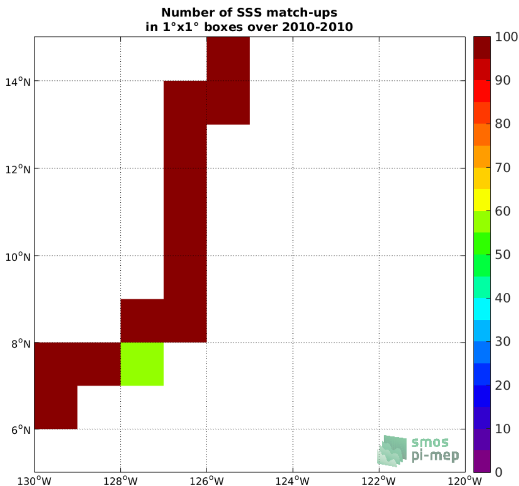
Figure 4: Number of SSS match-ups between TSG-GOSUD-Sailing-ship SSS and the SMOS L3 v317 - Monthly - 25 km (CATDS-CPDC) SSS product for the SPURS 2 Pi-MEP region over 1°x1° boxes and for the full satellite product period.
