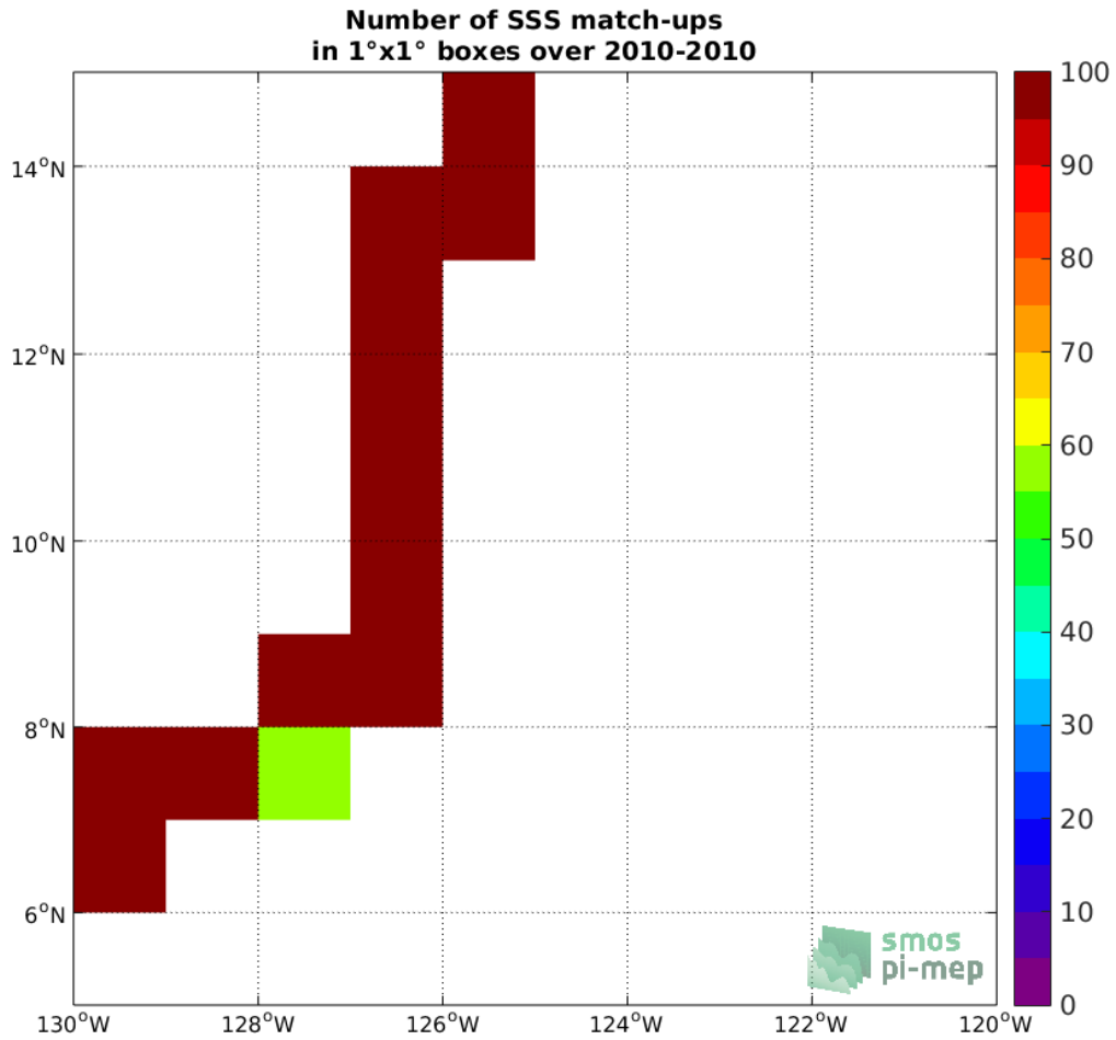
Figure 4: Number of SSS match-ups between TSG-GOSUD-Sailing-ship SSS and the SMOS-L3-CATDS-CPDC-V317-MONTHLY-25KM SSS product for the SPURS 2 Pi-MEP region over 1°x1° boxes and for the full satellite product period.
