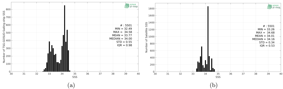
Figure 2: Histograms of SSS from TSG-GOSUD-Sailing-ship (a) and SMOS-L3-CATDS-CPDC-V317-MONTHLY-25KM (b) considering all match-up pairs per bins of 0.1 over the SPURS 2 Pi-MEP region and for the full satellite product period.
