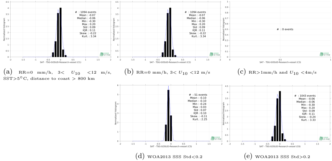
Figure 13: Normalized histogram of \Delta SSS (SMOS L3 v317 - Monthly - 25 km (CATDS-CPDC) - TSG-GOSUD-Research-vessel) for 5 different subdatasets corresponding to: RR=0 mm/h, 3 < U_{10} < 12 m/s, SST>5°C, distance to coast > 800 km (a), RR=0 mm/h, 3 < U_{10} < 12 m/s (b), RR>1mm/h and U_{10} < 4 m/s (c), WOA2013 SSS Std<0.2 (d), WOA2013 SSS Std>0.2 (e).
