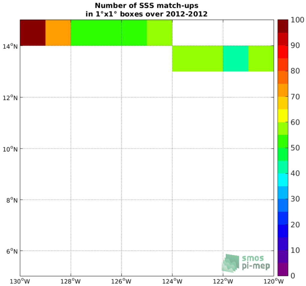
Figure 4: Number of SSS match-ups between TSG-GOSUD-Research-vessel SSS and the SMOS L3 v317 - Monthly - 25 km (CATDS-CPDC) SSS product for the SPURS 2 Pi-MEP region over 1°x1° boxes and for the full satellite product period.
