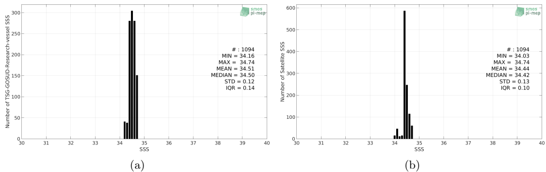
Figure 2: Histograms of SSS from TSG-GOSUD-Research-vessel (a) and SMOS L3 v317 - Monthly - 25 km (CATDS-CPDC) (b) considering all match-up pairs per bins of 0.1 over the SPURS 2 Pi-MEP region and for the full satellite product period.
