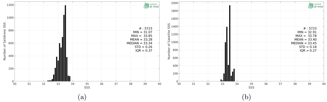
Figure 2: Histograms of SSS from Sairdrone (a) and SMOS SSS L3 v317 - Monthly - 25 km (CATDS-CPDC) (b) considering all match-up pairs per bins of 0.1 over the SPURS 2 Pi-MEP region and for the full satellite product period.
