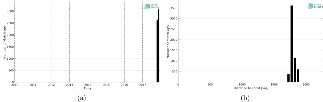
Figure 1: Number of match-ups between Saifdrone and SMOS SSS L3 v317 - Monthly - 25 km (CATDS-CPDC) SSS as a function of time (a) and as function of the distance to coast (b) over the SPURS 2 Pi-MEP region and for the full satellite product period.
