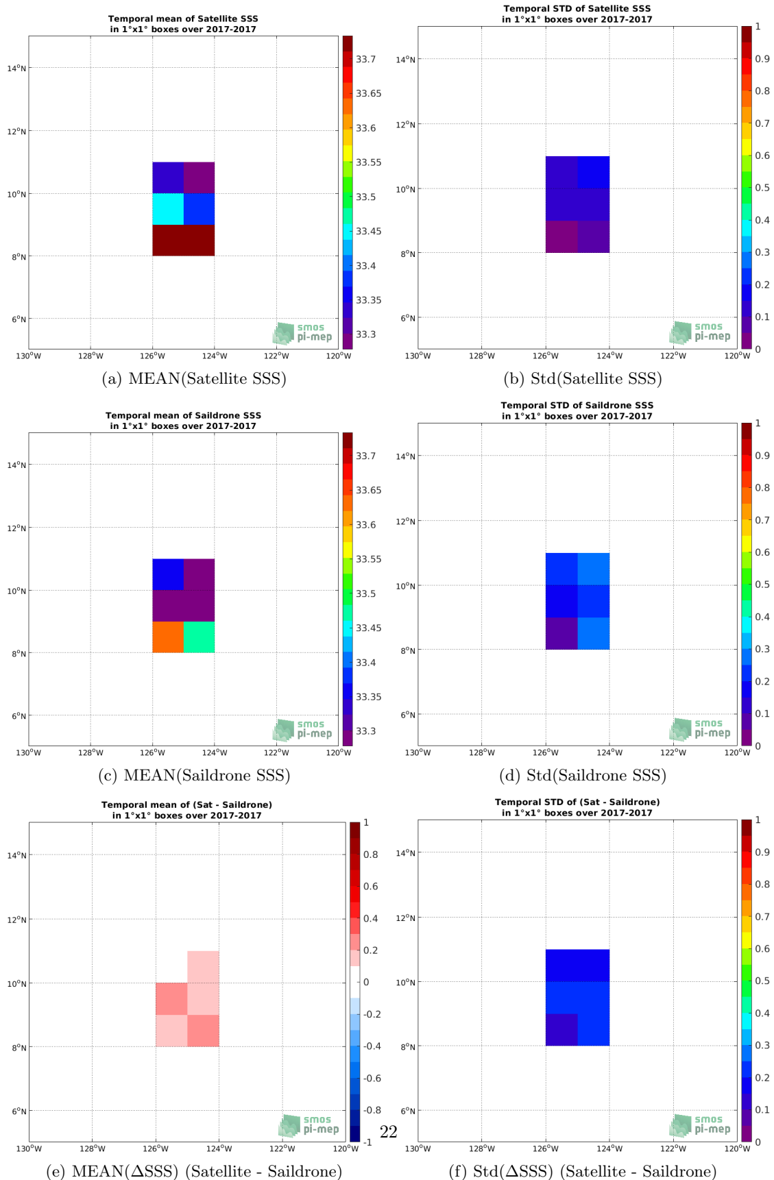
Figure 5: Temporal mean (left) and Std (right) of SSS from SMOS SSS L3 v317 - Monthly - 25 km (CATDS-CPDC) (top), Saildrone (middle), and of \Delta SSS (Satellite - Saildrone). Only match-up pairs are used to generate these maps.
