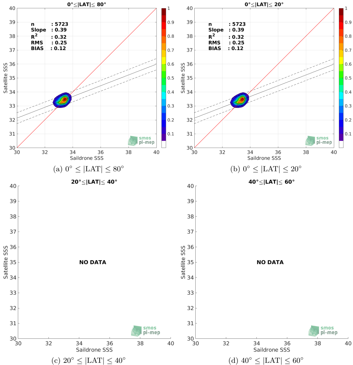
Figure 8: Contour maps of the concentration of SMOS SSS L3 v317 - Monthly - 25 km (CATDS-CPDC) SSS (y-axis) versus Saildrone SSS (x-axis) at match-up pairs for different latitude bands. For each plot, the red line shows x=y . The black thin and dashed lines indicate a linear fit through the data cloud and the \pm 95\% confidence levels, respectively. The number match-up pairs n , the slope and R^2 coefficient of the linear fit, the root mean square (RMS) and the mean bias between satellite and in situ data are indicated for each latitude band in each plots.
