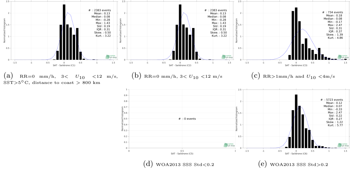
Figure 12: Normalized histogram of \Delta SSS (SMOS SSS L3 v317 - Monthly - 25 km (CATDS-CPDC) - Sairdrone) for 5 different subdatasets corresponding to: RR=0 mm/h, 3 < U_{10} < 12 m/s, SST > 5°C, distance to coast > 800 km (a), RR=0 mm/h, 3 < U_{10} < 12 m/s (b), RR > 1mm/h and U_{10} < 4 m/s (c), WOA2013 SSS Std < 0.2 (d), WOA2013 SSS Std > 0.2 (e).
