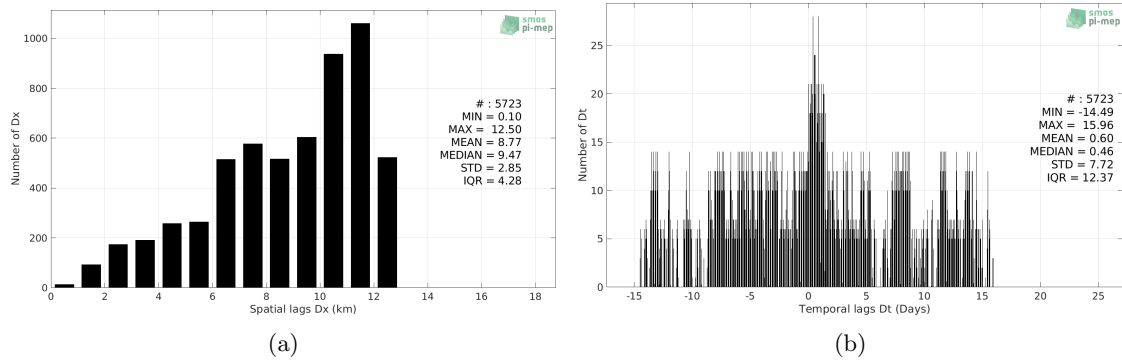
Figure 4: Histograms of the spatial (a) and temporal (b) lags between the location/time of the Sairdrone measurement and the date of the corresponding SMOS SSS L3 v317 - Monthly - 25 km (CATDS-CPDC) SSS pixel.
