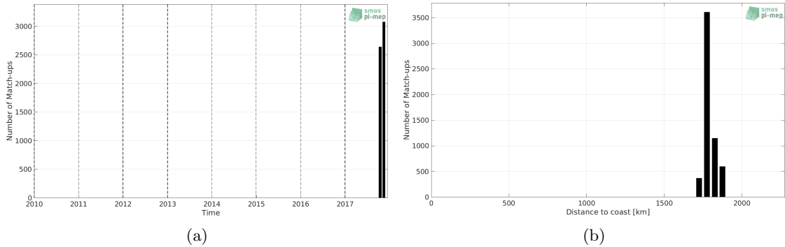
Figure 1: Number of match-ups between Saildrone and SMOS SSS L3 v317 - Monthly - 25 km (CATDS-CPDC) SSS as a function of time (a) and as function of the distance to coast (b) over the SPURS 2 Pi-MEP region and for the full satellite product period.
