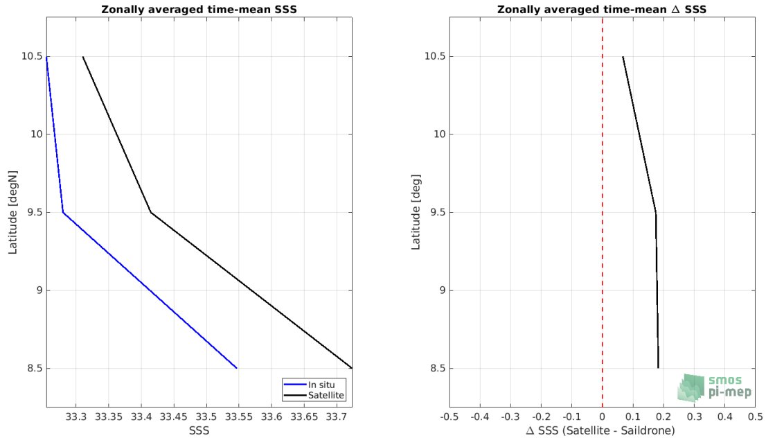
Figure 7: Left panel: Zonal mean SSS from SMOS SSS L3 v317 - Monthly - 25 km (CATDS-CPDC) satellite product (black) and from Saldrone (blue). Right panel: Zonal mean of \Delta SSS (Satellite - Saldrone) for all the collected Pi-MEP match-up pairs estimated over the full satellite product period.
