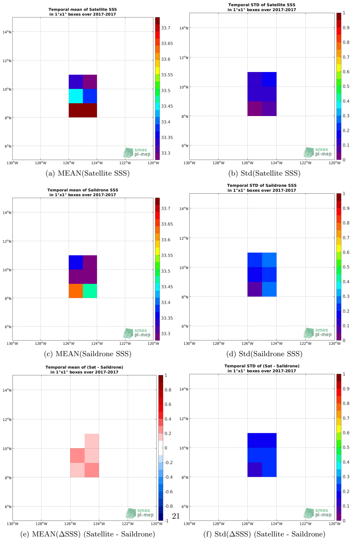
Figure 5: Temporal mean (left) and Std (right) of SSS from SMOS SSS L3 v317 - Monthly - 25 km (CATDS-CPDC) (top), Saildrone (middle), and of \Delta SSS (Satellite - Saildrone). Only match-up pairs are used to generate these maps.
