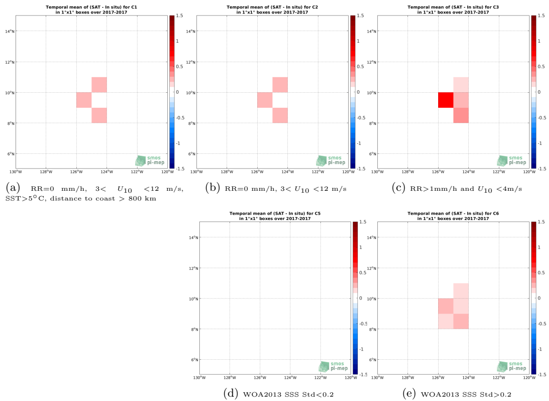
Figure 11: Temporal mean gridded over spatial boxes of size 1^\circ \times 1^\circ of \Delta SSS (SMOS SSS L3 v317 - Monthly - 25 km (CATDS-CPDC) - Saildrone) for 5 different subdatasets corresponding to:RR=0 mm/h, 3 < U_{10} < 12 m/s, SST >5^\circ\text{C} , distance to coast > 800 km (a), RR=0 mm/h, 3 < U_{10} < 12 m/s (b), RR >1 mm/h and U_{10} < 4 m/s (c), WOA2013 SSS Std <0.2 (d), WOA2013 SSS Std >0.2 (e).
