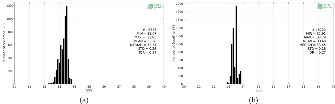
Figure 2: Histograms of SSS from Saildrone (a) and SMOS SSS L3 v317 - Monthly - 25 km (CATDS-CPDC) (b) considering all match-up pairs per bins of 0.1 over the SPURS 2 Pi-MEP region and for the full satellite product period.
