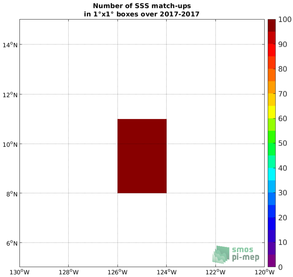
Figure 3: Number of SSS match-ups between Saildrone SSS and the SMOS SSS L3 v317 - Monthly - 25 km (CATDS-CPDC) SSS product for the SPURS 2 Pi-MEP region over 1°x1° boxes and for the full satellite product period.
