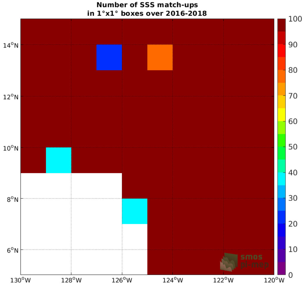
Figure 3: Number of SSS match-ups between Surface drifters SSS and the SMOS SSS L3 v317 - Monthly - 25 km (CATDS-CPDC) SSS product for the SPURS 2 Pi-MEP region over 1^\circ \times 1^\circ boxes and for the full satellite product period.
