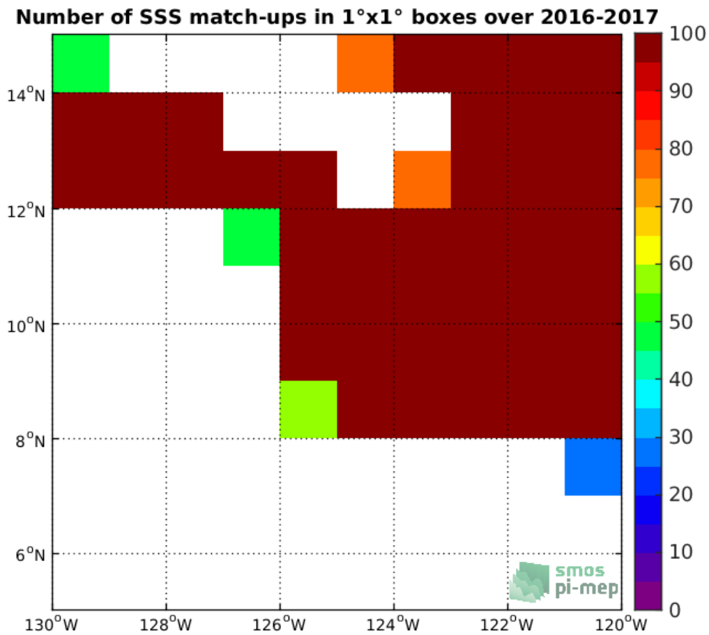
Figure 3: Number of SSS match-ups between Surface drifters SSS and the SMOS-L3-CATDS-CPDC-V317-MONTHLY-25KM SSS product for the SPURS 2 Pi-MEP region over 1°x1° boxes and for the full satellite product period.
