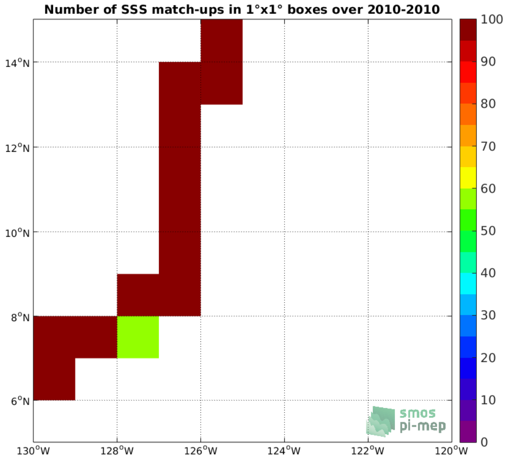
Figure 4: Number of SSS match-ups between TSG-GOSUD-Sailing-ship SSS and the SMOS-L3-CATDS-CPDC-V317-10DAYS-25KM SSS product for the SPURS 2 Pi-MEP region over 1°x1° boxes and for the full satellite product period.
