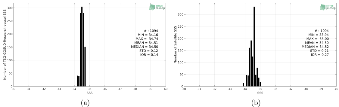
Figure 2: Histograms of SSS from TSG-GOSUD-Research-vessel (a) and SMOS L3 v317 - 10 Days - 25 km (CATDS-CPDC) (b) considering all match-up pairs per bins of 0.1 over the SPURS 2 Pi-MEP region and for the full satellite product period.
