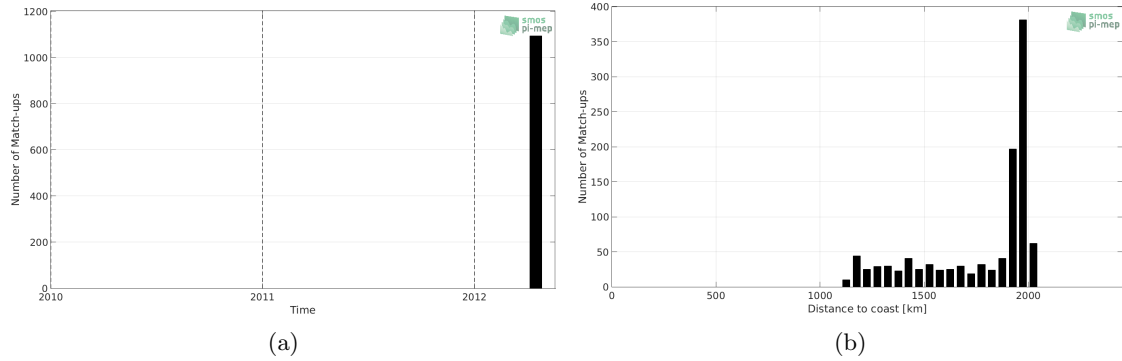
Figure 1: Number of match-ups between TSG-GOSUD-Research-vessel and SMOS L3 v317 - 10 Days - 25 km (CATDS-CPDC) SSS as a function of time (a) and as function of the distance to coast (b) over the SPURS 2 Pi-MEP region and for the full satellite product period.
