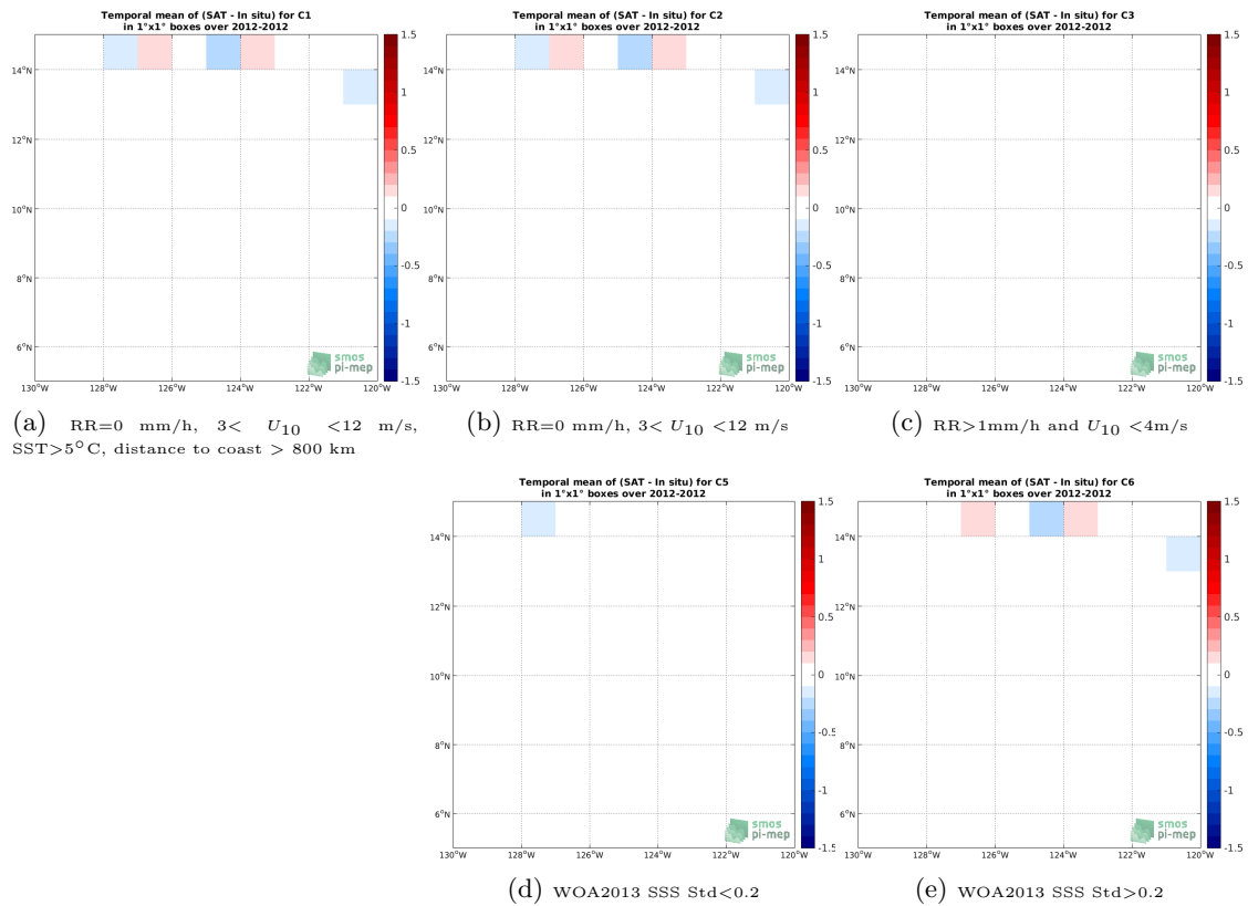
Figure 12: Temporal mean gridded over spatial boxes of size 1°x1° of \Delta SSS (SMOS L3 v317 - 10 Days - 25 km (CATDS-CPDC) - TSG-GOSUD-Research-vessel) for 5 different subdatasets corresponding to:RR=0 mm/h, 3 < U_{10} < 12 m/s, SST>5°C, distance to coast > 800 km (a), RR=0 mm/h, 3 < U_{10} < 12 m/s (b), RR>1mm/h and U_{10} < 4 m/s (c), WOA2013 SSS Std<0.2 (d), WOA2013 SSS Std>0.2 (e).
