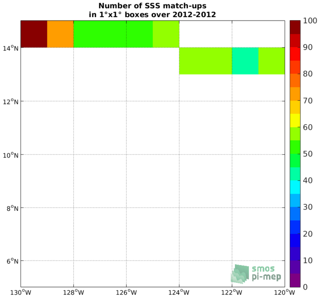
Figure 4: Number of SSS match-ups between TSG-GOSUD-Research-vessel SSS and the SMOS L3 v317 - 10 Days - 25 km (CATDS-CPDC) SSS product for the SPURS 2 Pi-MEP region over 1°x1° boxes and for the full satellite product period.
