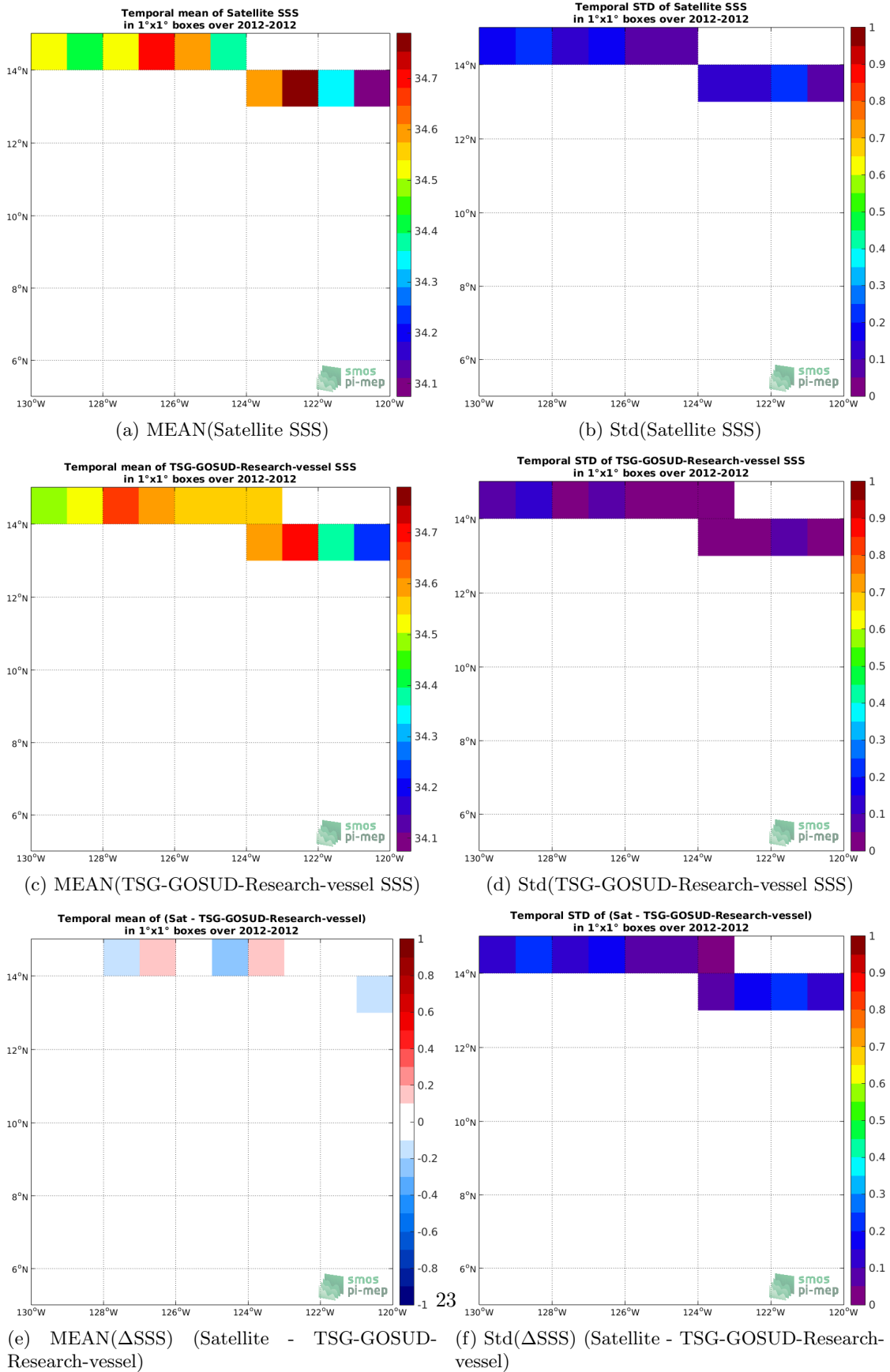
Figure 6: Temporal mean (left) and Std (right) of SSS from SMOS L3 v317 - 10 Days - 25 km (CATDS-CPDC) (top), TSG-GOSUD-Research-vessel (middle), and of \Delta SSS (Satellite - TSG-GOSUD-Research-vessel). Only match-up pairs are used to generate these maps.
