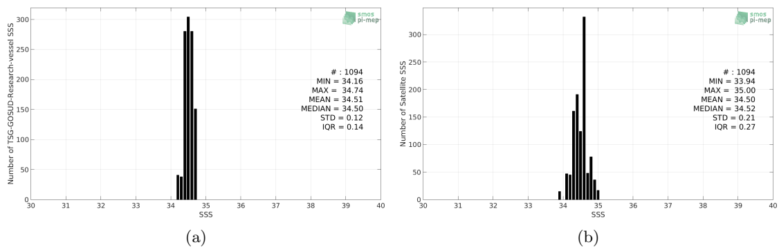
Figure 2: Histograms of SSS from TSG-GOSUD-Research-vessel (a) and SMOS-L3-CATDS-CPDC-V317-10DAYS-25KM (b) considering all match-up pairs per bins of 0.1 over the SPURS 2 Pi-MEP region and for the full satellite product period.
