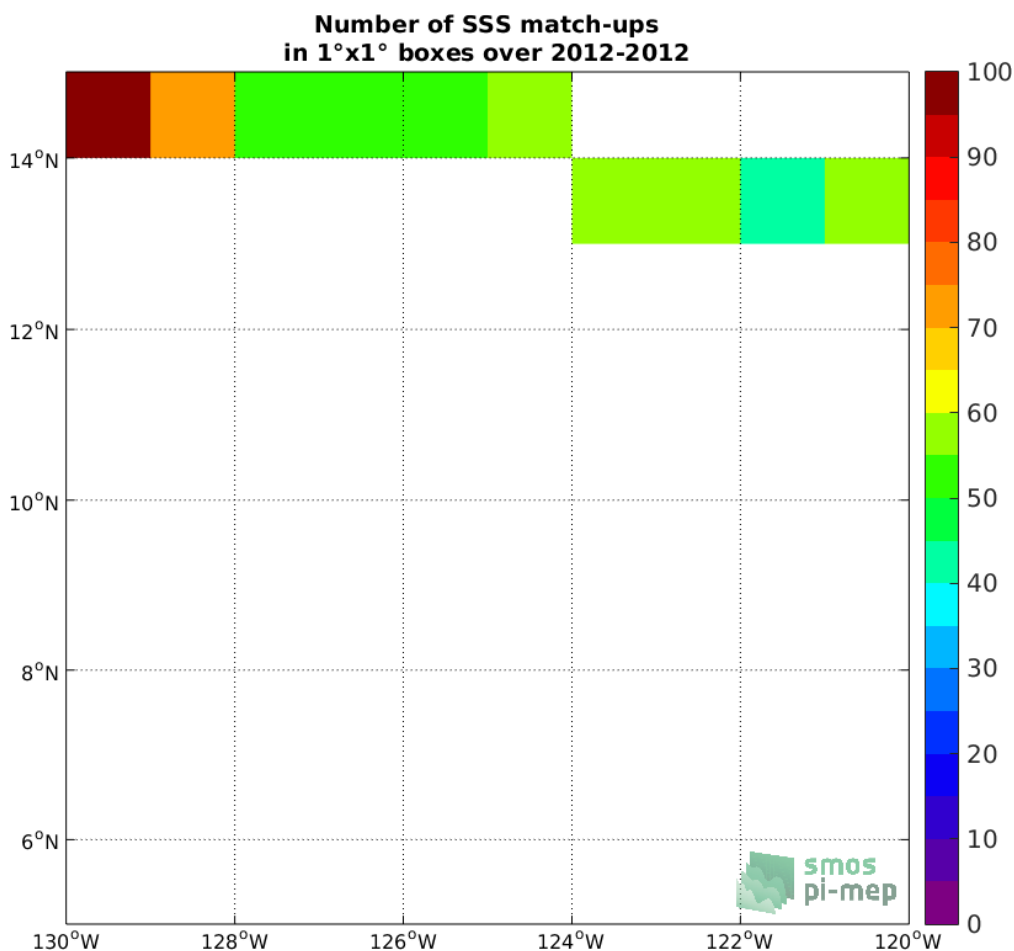
Figure 4: Number of SSS match-ups between TSG-GOSUD-Research-vessel SSS and the SMOS-L3-CATDS-CPDC-V317-10DAYS-25KM SSS product for the SPURS 2 Pi-MEP region over 1°x1° boxes and for the full satellite product period.
