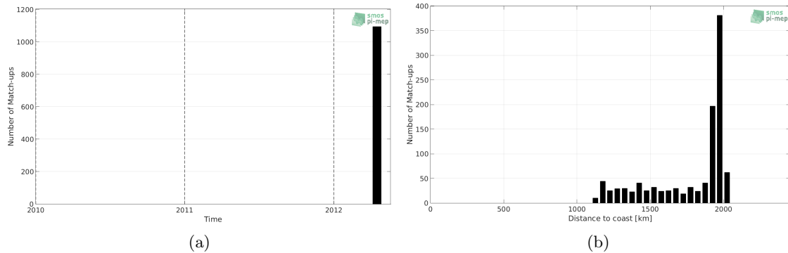
Figure 1: Number of match-ups between TSG-GOSUD-Research-vessel and SMOS-L3-CATDS-CPDC-V317-10DAYS-25KM SSS as a function of time (a) and as function of the distance to coast (b) over the SPURS 2 Pi-MEP region and for the full satellite product period.
