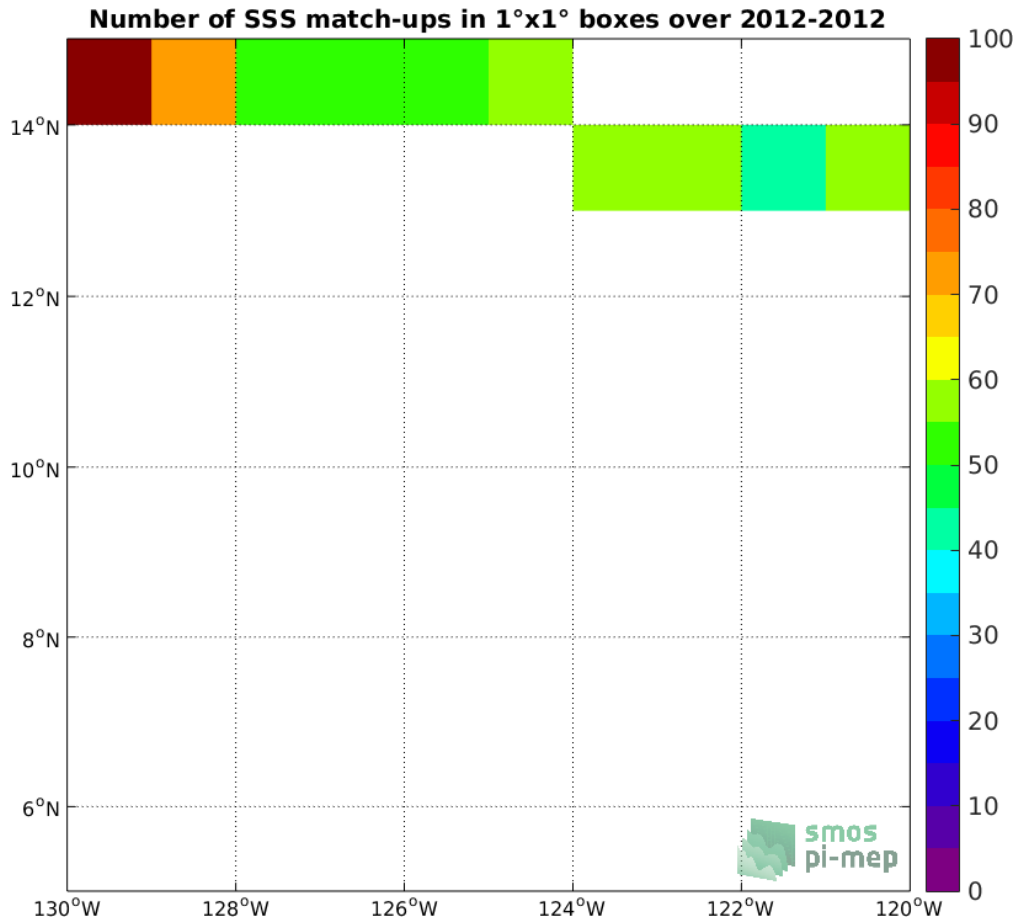
Figure 4: Number of SSS match-ups between TSG-GOSUD-Research-vessel SSS and the SMOS-L3-CATDS-CPDC-V317-10DAYS-25KM SSS product for the SPURS 2 Pi-MEP region over 1°x1° boxes and for the full satellite product period.
