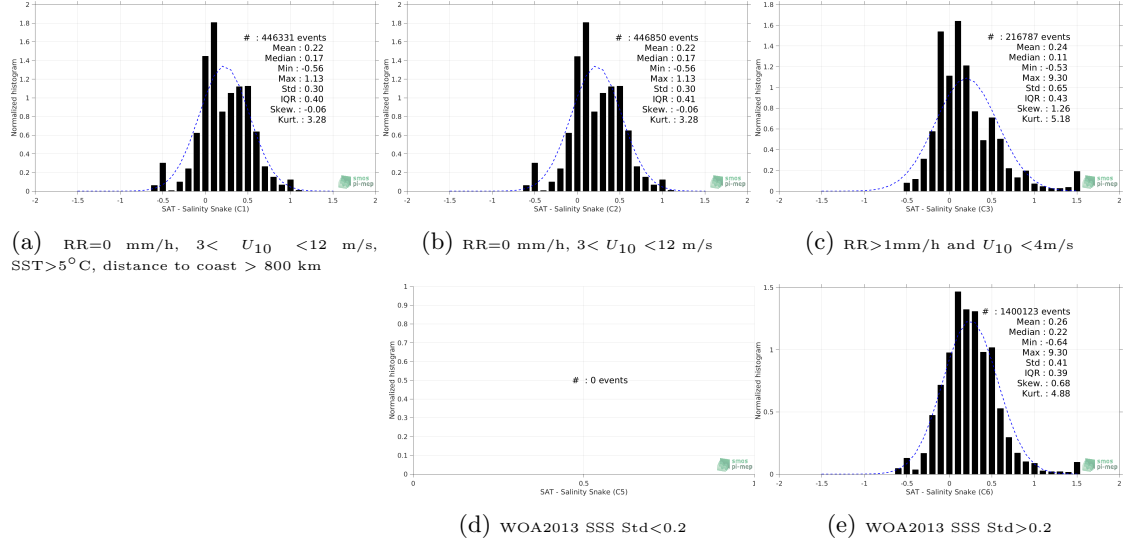
Figure 13: Normalized histogram of \Delta SSS (SMOS SSS L3 v317 - 10 Days - 25 km (CATDS-CPDC) - Salinity Snake) for 5 different subdatasets corresponding to: RR=0 mm/h, 3 < U_{10} < 12 m/s, SST > 5°C, distance to coast > 800 km (a), RR=0 mm/h, 3 < U_{10} < 12 m/s (b), RR > 1mm/h and U_{10} < 4 m/s (c), WOA2013 SSS Std < 0.2 (d), WOA2013 SSS Std > 0.2 (e).
