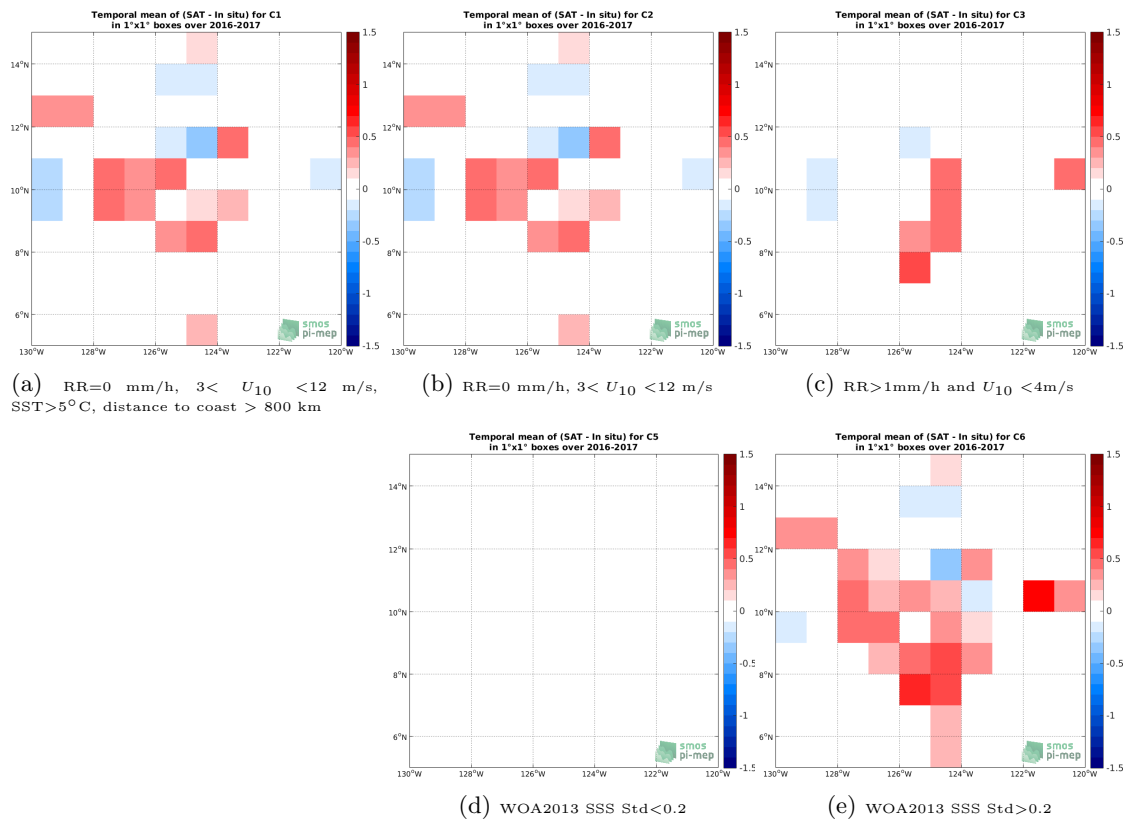
Figure 12: Temporal mean gridded over spatial boxes of size 1^\circ \times 1^\circ of \Delta SSS (SMOS SSS L3 v317 - 10 Days - 25 km (CATDS-CPDC) - Salinity Snake) for 5 different subdatasets corresponding to:RR=0 mm/h, 3 < U_{10} < 12 m/s, SST >5^\circ\text{C} , distance to coast > 800 km (a), RR=0 mm/h, 3 < U_{10} < 12 m/s (b), RR >1 mm/h and U_{10} < 4 m/s (c), WOA2013 SSS Std <0.2 (d), WOA2013 SSS Std >0.2 (e).
