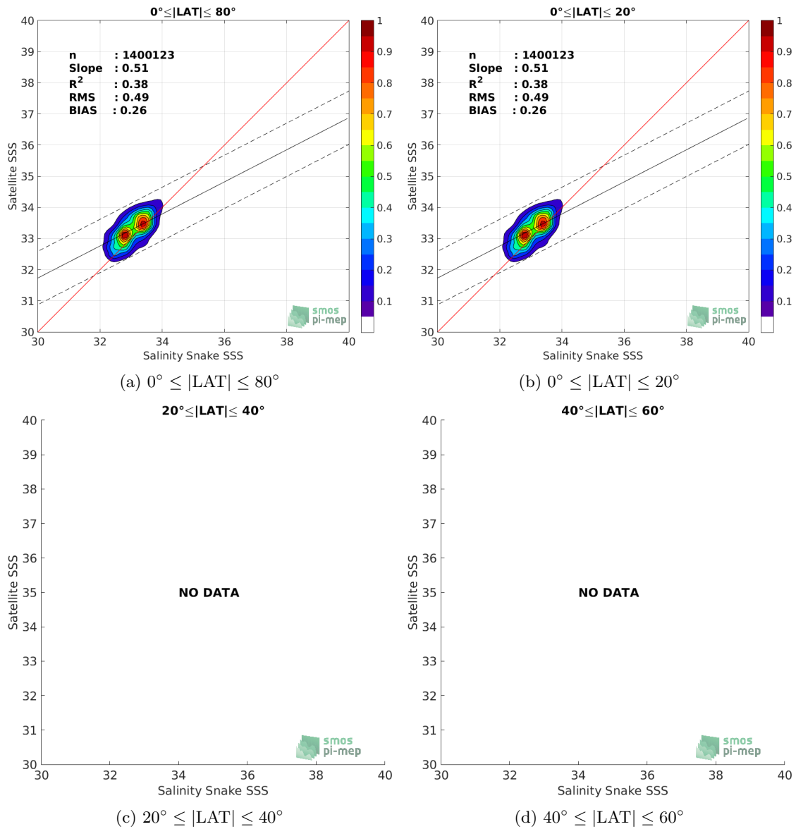
Figure 9: Contour maps of the concentration of SMOS SSS L3 v317 - 10 Days - 25 km (CATDS-CPDC) SSS (y-axis) versus Salinity Snake SSS (x-axis) at match-up pairs for different latitude bands. For each plot, the red line shows x=y . The black thin and dashed lines indicate a linear fit through the data cloud and the \pm 95\% confidence levels, respectively. The number match-up pairs n , the slope and R^2 coefficient of the linear fit, the root mean square (RMS) and the mean bias between satellite and in situ data are indicated for each latitude band in each plots.
