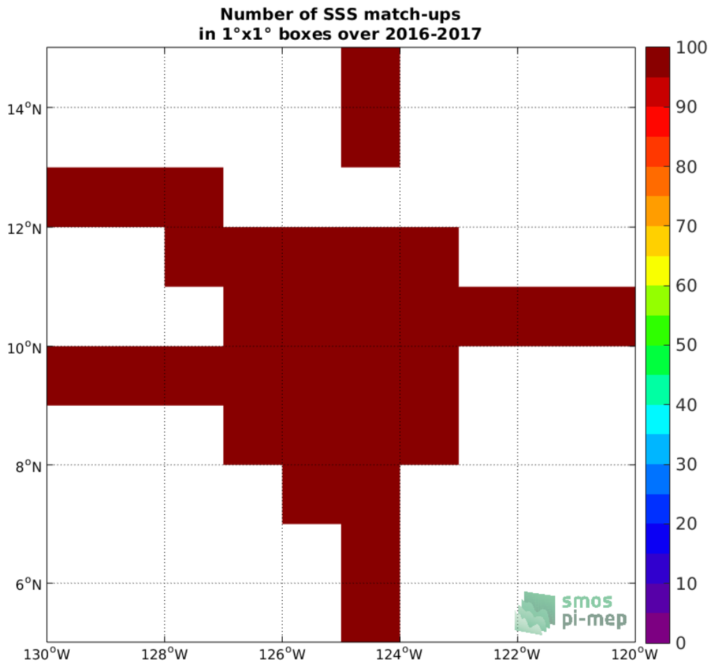
Figure 4: Number of SSS match-ups between Salinity Snake SSS and the SMOS SSS L3 v317 - 10 Days - 25 km (CATDS-CPDC) SSS product for the SPURS 2 Pi-MEP region over 1°x1° boxes and for the full satellite product period.
