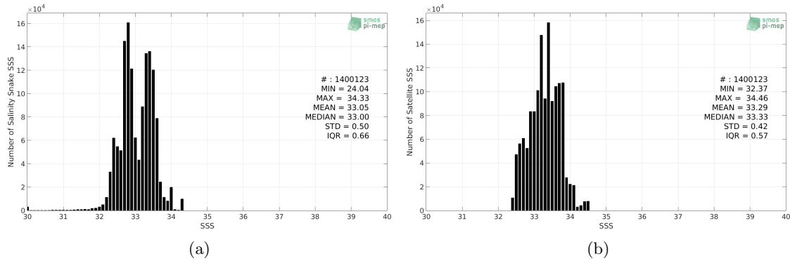
Figure 2: Histograms of SSS from Salinity Snake (a) and SMOS SSS L3 v317 - 10 Days - 25 km (CATDS-CPDC) (b) considering all match-up pairs per bins of 0.1 over the SPURS 2 Pi-MEP region and for the full satellite product period.
