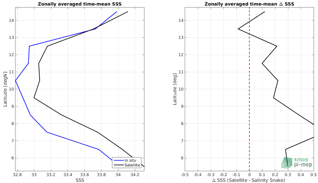
Figure 8: Left panel: Zonal mean SSS from SMOS SSS L3 v317 - 10 Days - 25 km (CATDS-CPDC) satellite product (black) and from Salinity Snake (blue). Right panel: Zonal mean of \Delta SSS (Satellite - Salinity Snake) for all the collected Pi-MEP match-up pairs estimated over the full satellite product period.
