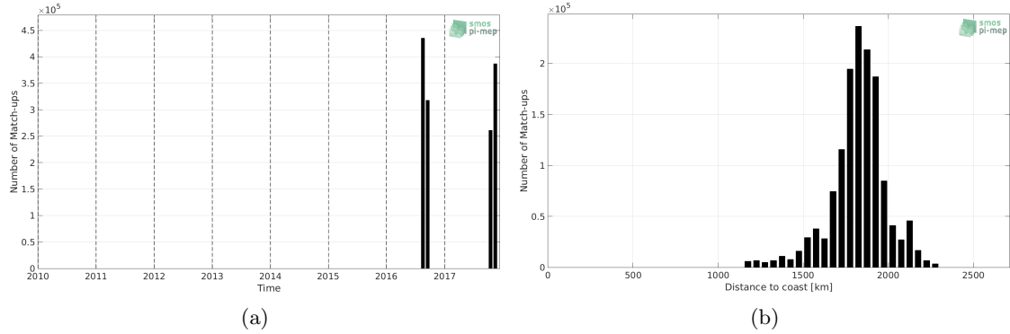
Figure 1: Number of match-ups between Salinity Snake and SMOS SSS L3 v317 - 10 Days - 25 km (CATDS-CPDC) SSS as a function of time (a) and as function of the distance to coast (b) over the SPURS 2 Pi-MEP region and for the full satellite product period.
