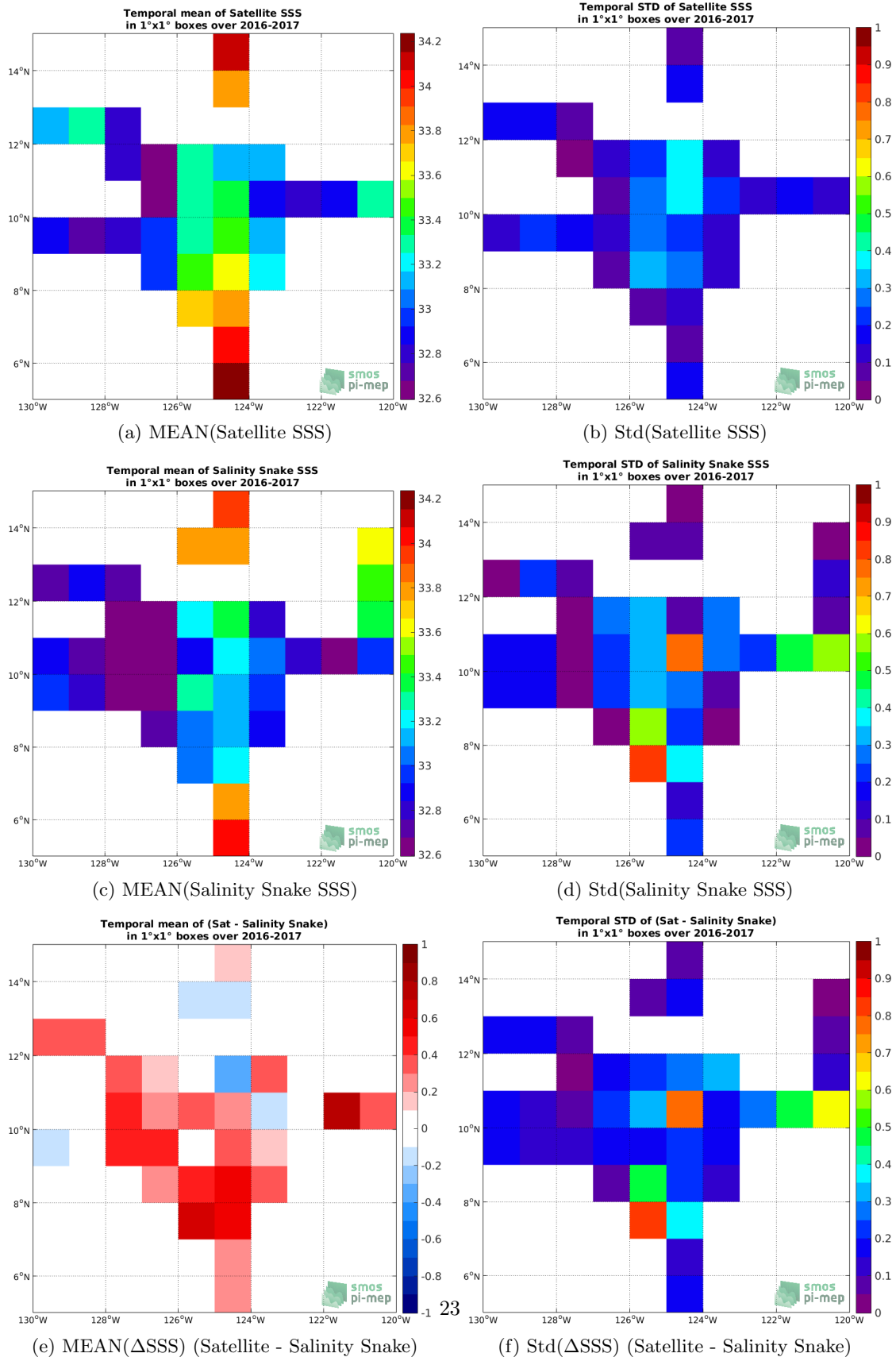
Figure 6: Temporal mean (left) and Std (right) of SSS from SMOS SSS L3 v317 - 10 Days - 25 km (CATDS-CPDC) (top), Salinity Snake (middle), and of \Delta SSS (Satellite - Salinity Snake). Only match-up pairs are used to generate these maps.
