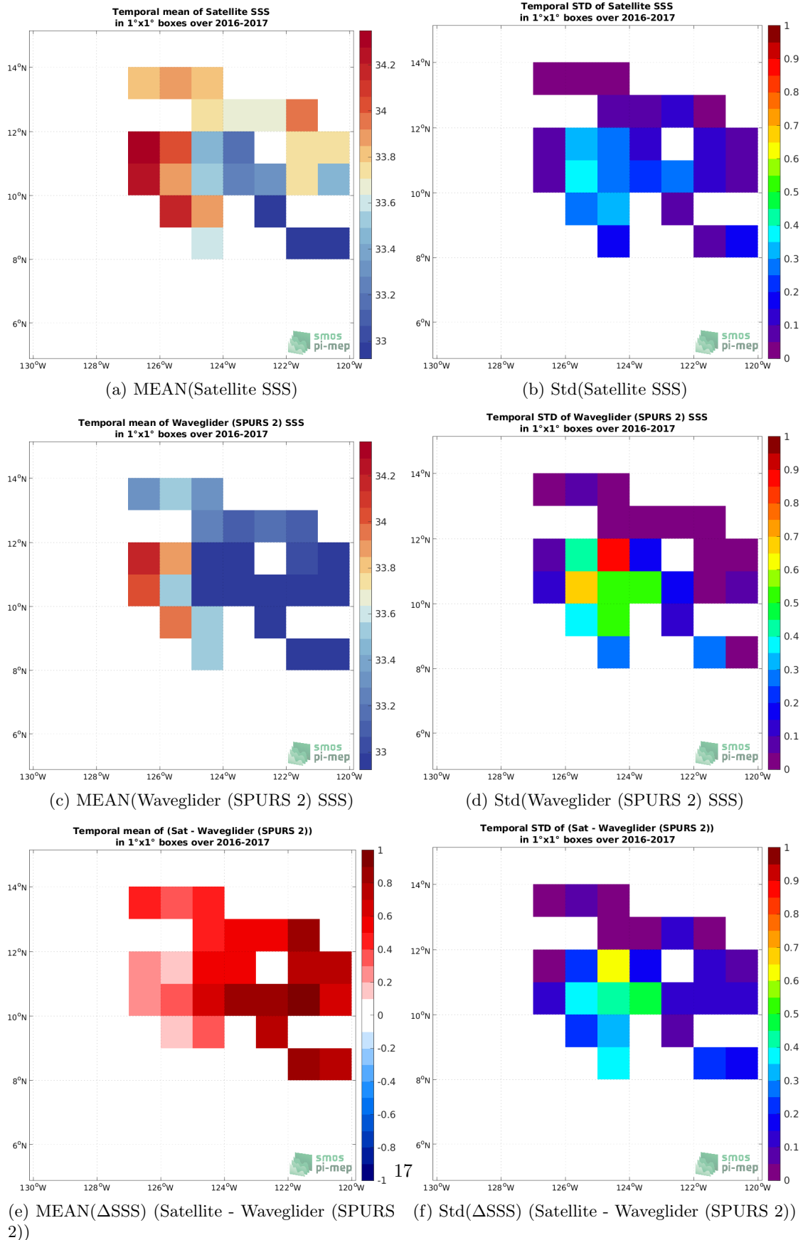
Figure 6: Temporal mean (left) and Std (right) of SSS from SMOS SSS L3 v2 - 9-Days (BEC) (top), Waveglider (SPURS 2) (middle), and of \Delta SSS (Satellite - Waveglider (SPURS 2)). Only match-up pairs are used to generate these maps.
