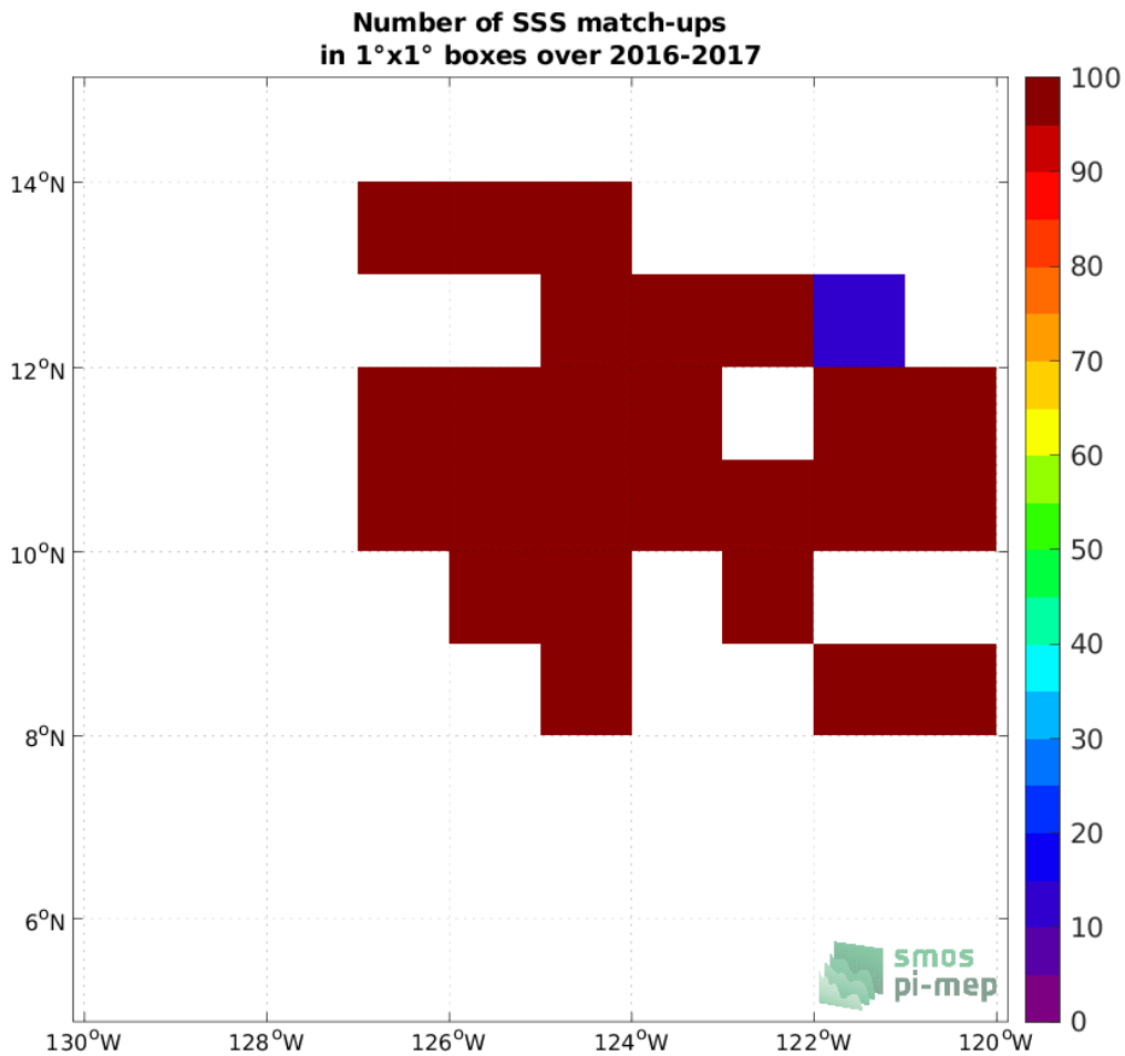
Figure 4: Number of SSS match-ups between Waveglider (SPURS 2) SSS and the SMOS SSS L3 v2 - 9-Days (BEC) SSS product for the SPURS 2 Pi-MEP region over 1°x1° boxes and for the full satellite product period.
