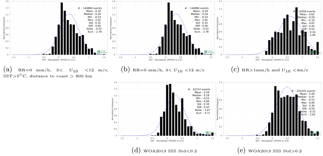
Figure 13: Normalized histogram of \Delta SSS (SMOS SSS L3 v2 - 9-Days (BEC) - Waveglider (SPURS 2)) for 5 different subdatasets corresponding to: RR=0 mm/h, 3 < U_{10} < 12 m/s, SST > 5°C, distance to coast > 800 km (a), RR=0 mm/h, 3 < U_{10} < 12 m/s (b), RR > 1mm/h and U_{10} < 4 m/s (c), WOA2013 SSS Std < 0.2 (d), WOA2013 SSS Std > 0.2 (e).
