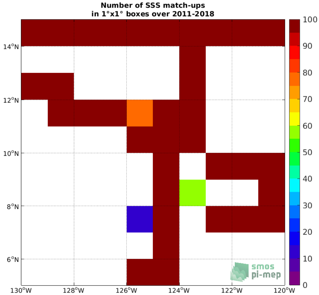
Figure 4: Number of SSS match-ups between TSG (SAMOS) SSS and the SMOS SSS L3 v2 - 9-Days (BEC) SSS product for the SPURS 2 Pi-MEP region over 1°x1° boxes and for the full satellite product period.
