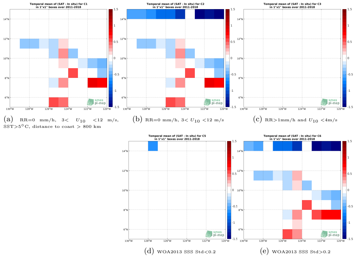
Figure 12: Temporal mean gridded over spatial boxes of size 1^\circ \times 1^\circ of \Delta SSS (SMOS SSS L3 v2 - 9-Days (BEC) - TSG (SAMOS)) for 5 different subdatasets corresponding to:RR=0 mm/h, 3 < U_{10} < 12 m/s, SST >5^\circ\text{C} , distance to coast > 800 km (a), RR=0 mm/h, 3 < U_{10} < 12 m/s (b), RR >1 mm/h and U_{10} < 4 m/s (c), WOA2013 SSS Std <0.2 (d), WOA2013 SSS Std >0.2 (e).
