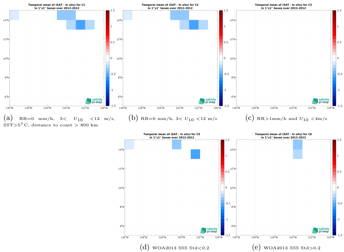
Figure 14: Temporal mean gridded over spatial boxes of size 1^\circ \times 1^\circ of \Delta\text{SSS} (SMOS SSS L3 v2 - 9-Days (BEC) - TSG (GOSUD-Research-vessel)) for 5 different subdatasets corresponding to:RR=0 mm/h, 3 < U_{10} < 12 m/s, SST>5°C, distance to coast > 800 km (a), RR=0 mm/h, 3 < U_{10} < 12 m/s (b), RR>1mm/h and U_{10} < 4 m/s (c), WOA2013 SSS Std<0.2 (d), WOA2013 SSS Std>0.2 (e).
