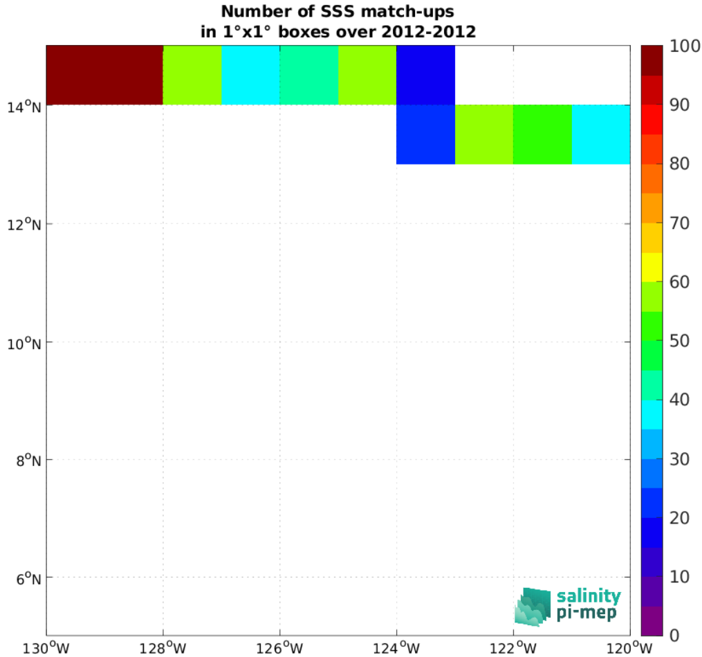
Figure 5: Number of SSS match-ups between TSG (GOSUD-Research-vessel) SSS and the SMOS SSS L3 v2 - 9-Days (BEC) SSS product for the SPURS 2 Pi-MEP region over 1^\circ \times 1^\circ boxes and for the full satellite product period.
