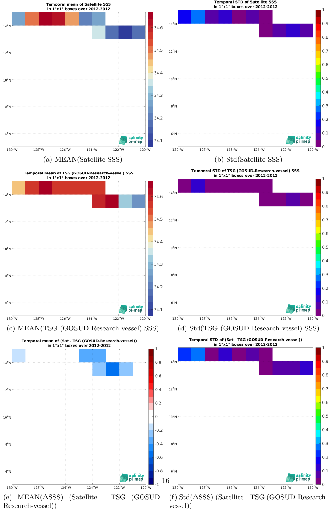
Figure 7: Temporal mean (left) and Std (right) of SSS from SMOS SSS L3 v2 - 9-Days (BEC) (top), TSG (GOSUD-Research-vessel) (middle), and of \Delta SSS (Satellite - TSG (GOSUD-Research-vessel)). Only match-up pairs are used to generate these maps.
