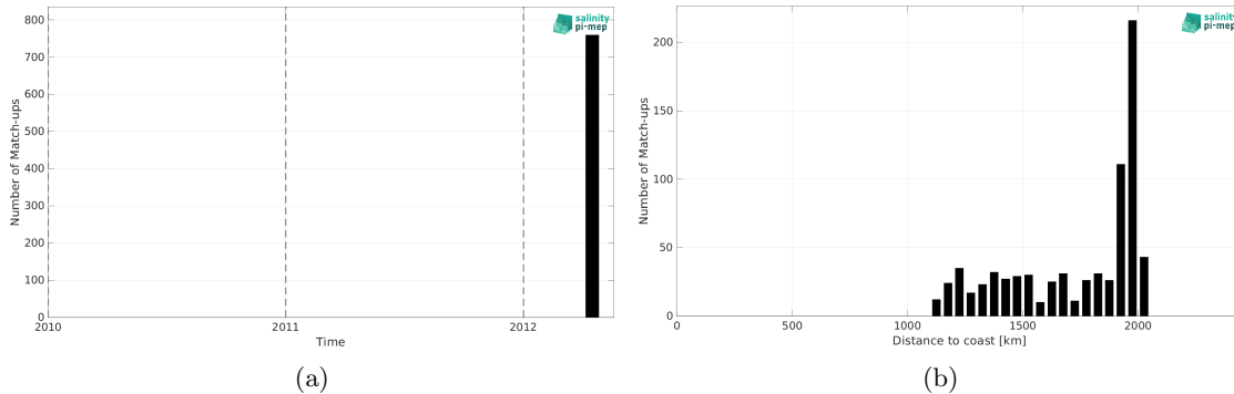
Figure 2: Number of match-ups between TSG (GOSUD-Research-vessel) and SMOS SSS L3 v2 - 9-Days (BEC) SSS as a function of time (a) and as function of the distance to coast (b) over the SPURS 2 Pi-MEP region and for the full satellite product period.
