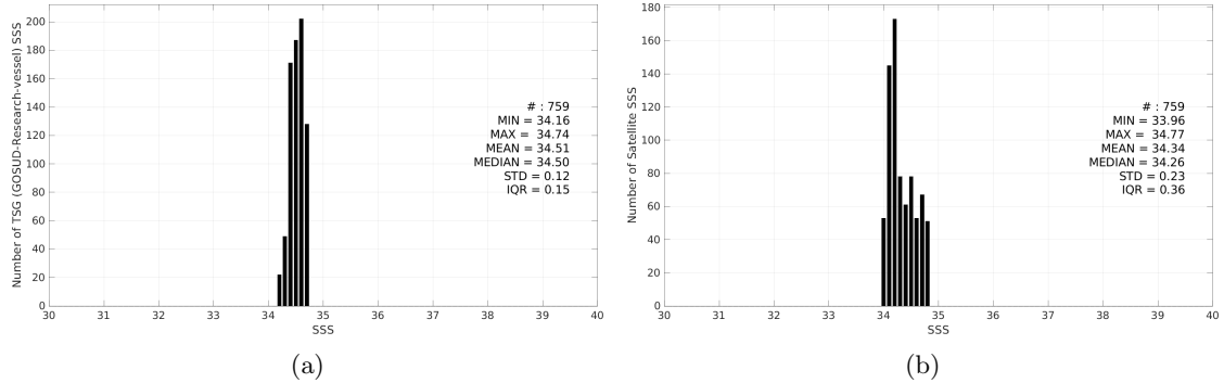
Figure 3: Histograms of SSS from TSG (GOSUD-Research-vessel) (a) and SMOS SSS L3 v2 - 9-Days (BEC) (b) considering all match-up pairs per bins of 0.1 over the SPURS 2 Pi-MEP region and for the full satellite product period.
