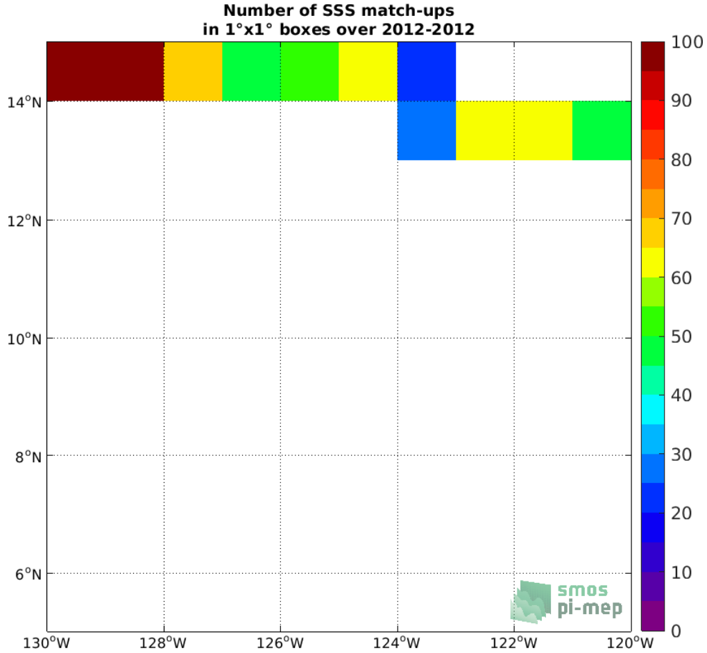
Figure 4: Number of SSS match-ups between TSG (GOSUD-Research-vessel) SSS and the SMOS SSS L3 v2 - 9-Days (BEC) SSS product for the SPURS 2 Pi-MEP region over 1°x1° boxes and for the full satellite product period.
