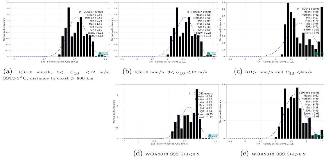
Figure 15: Normalized histogram of \Delta SSS (SMOS SSS L3 v2 - 9-Days (BEC) - Salinity Snake (SPURS 2)) for 5 different subdatasets corresponding to: RR=0 mm/h, 3 < U_{10} < 12 m/s, SST>5°C, distance to coast > 800 km (a), RR=0 mm/h, 3 < U_{10} < 12 m/s (b), RR>1mm/h and U_{10} < 4 m/s (c), WOA2013 SSS Std<0.2 (d), WOA2013 SSS Std>0.2 (e).
