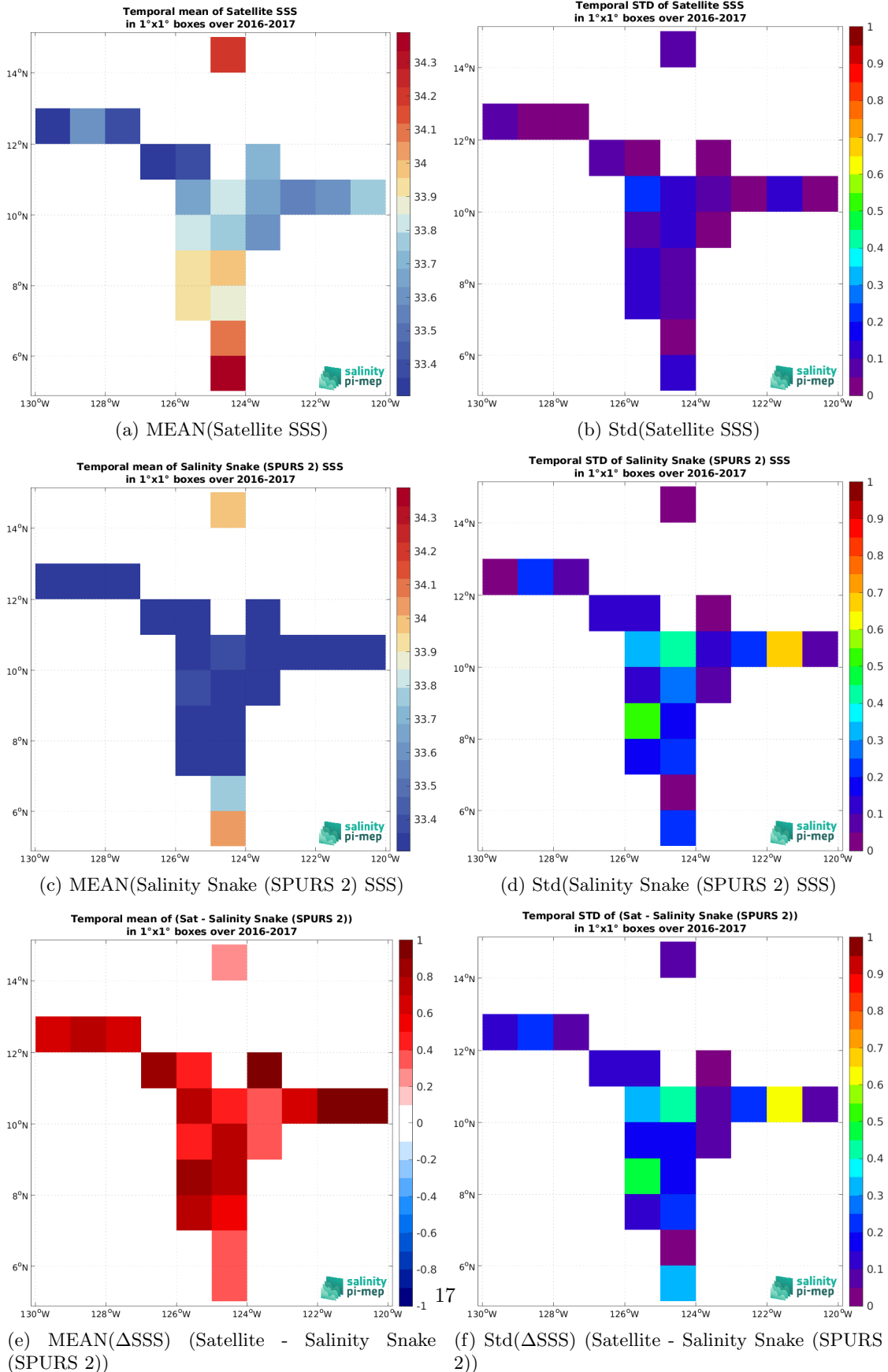
Figure 7: Temporal mean (left) and Std (right) of SSS from SMOS SSS L3 v2 - 9-Days (BEC) (top), Salinity Snake (SPURS 2) (middle), and of \Delta SSS (Satellite - Salinity Snake (SPURS 2)). Only match-up pairs are used to generate these maps.
