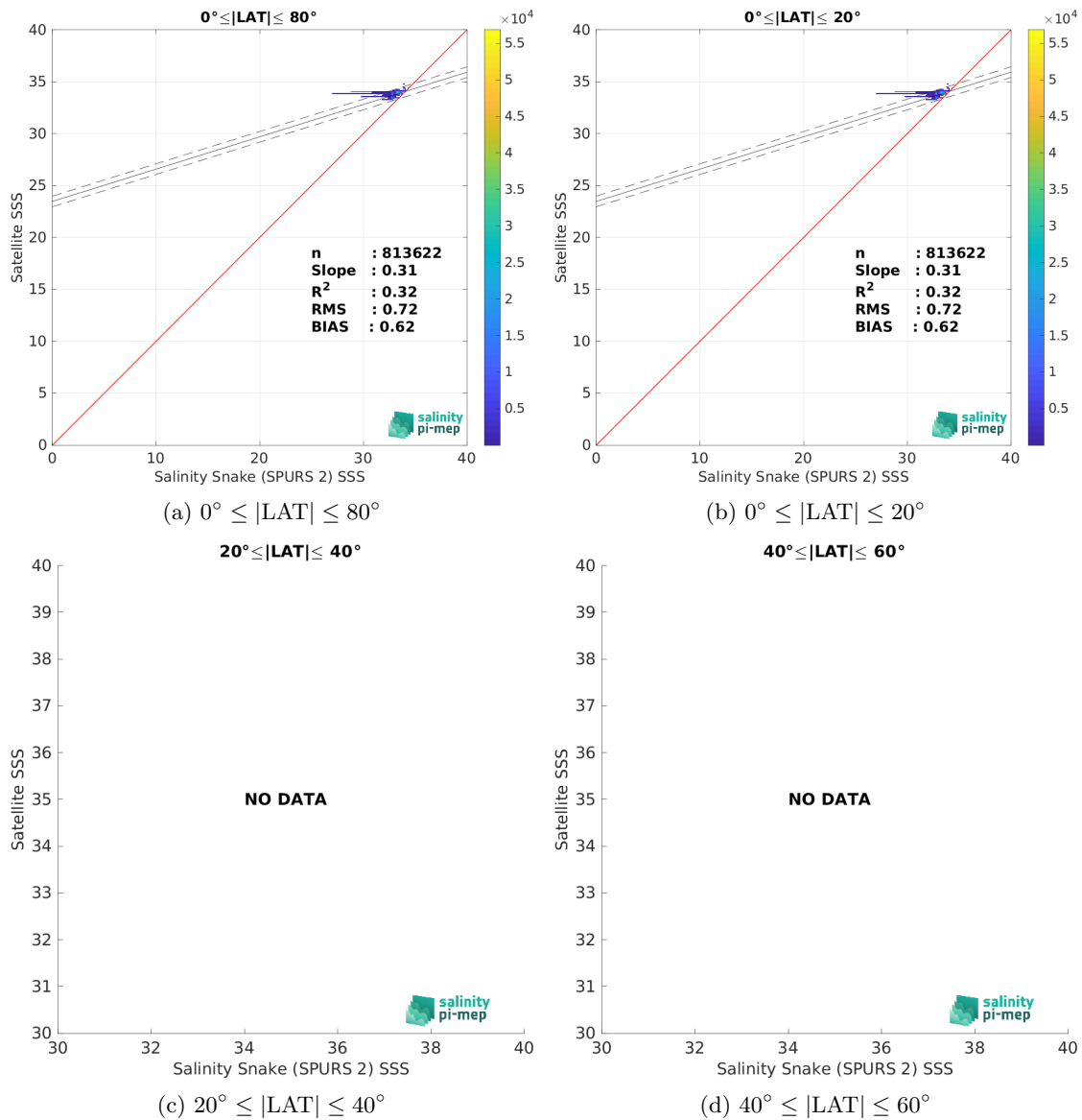
Figure 10: Contour maps of the concentration of SMOS SSS L3 v2 - 9-Days (BEC) SSS (y-axis) versus Salinity Snake (SPURS 2) SSS (x-axis) at match-up pairs for different latitude bands. For each plot, the red line shows x=y . The black thin and dashed lines indicate a linear fit through the data cloud and the \pm 95\% confidence levels, respectively. The number match-up pairs n , the slope and R^2 coefficient of the linear fit, the root mean square (RMS) and the mean bias between satellite and in situ data are indicated for each latitude band in each plots.
