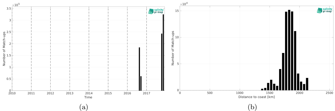
Figure 2: Number of match-ups between Salinity Snake (SPURS 2) and SMOS SSS L3 v2 - 9-Days (BEC) SSS as a function of time (a) and as function of the distance to coast (b) over the SPURS 2 Pi-MEP region and for the full satellite product period.
