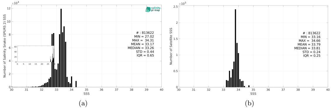
Figure 3: Histograms of SSS from Salinity Snake (SPURS 2) (a) and SMOS SSS L3 v2 - 9-Days (BEC) (b) considering all match-up pairs per bins of 0.1 over the SPURS 2 Pi-MEP region and for the full satellite product period.
