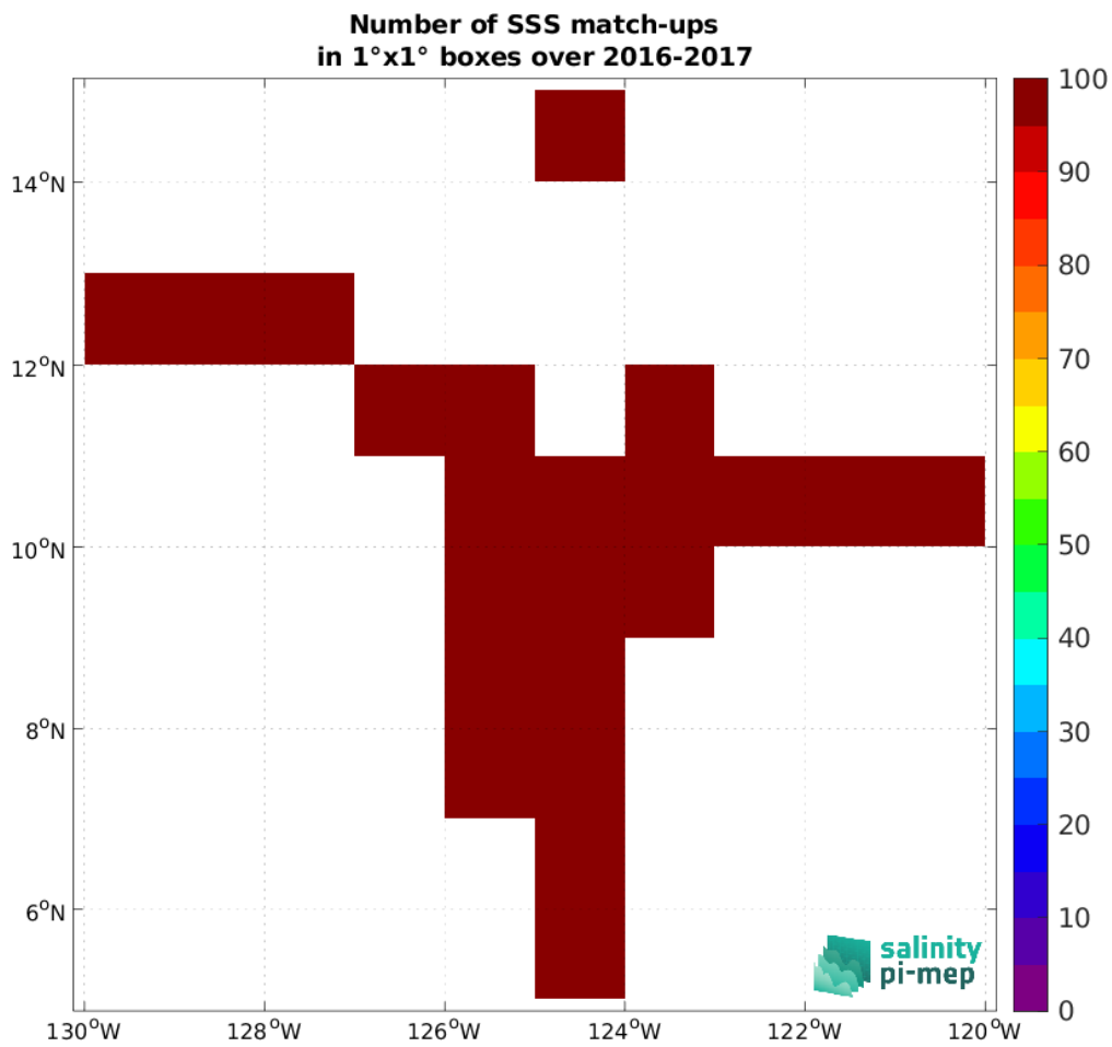
Figure 5: Number of SSS match-ups between Salinity Snake (SPURS 2) SSS and the SMOS SSS L3 v2 - 9-Days (BEC) SSS product for the SPURS 2 Pi-MEP region over 1^\circ \times 1^\circ boxes and for the full satellite product period.
