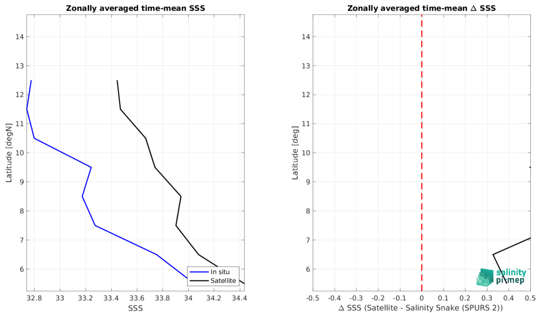
Figure 9: Left panel: Zonal mean SSS from SMOS SSS L3 v2 - 9-Days (BEC) satellite product (black) and from Salinity Snake (SPURS 2) (blue). Right panel: Zonal mean of \Delta SSS (Satellite - Salinity Snake (SPURS 2)) for all the collected Pi-MEP match-up pairs estimated over the full satellite product period.
