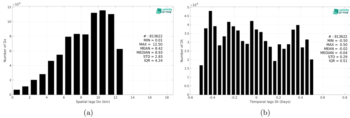
Figure 6: Histograms of the spatial (a) and temporal (b) lags between the location/time of the Salinity Snake (SPURS 2) measurement and the date of the corresponding SMOS SSS L3 v2 - 9-Days (BEC) SSS pixel.
