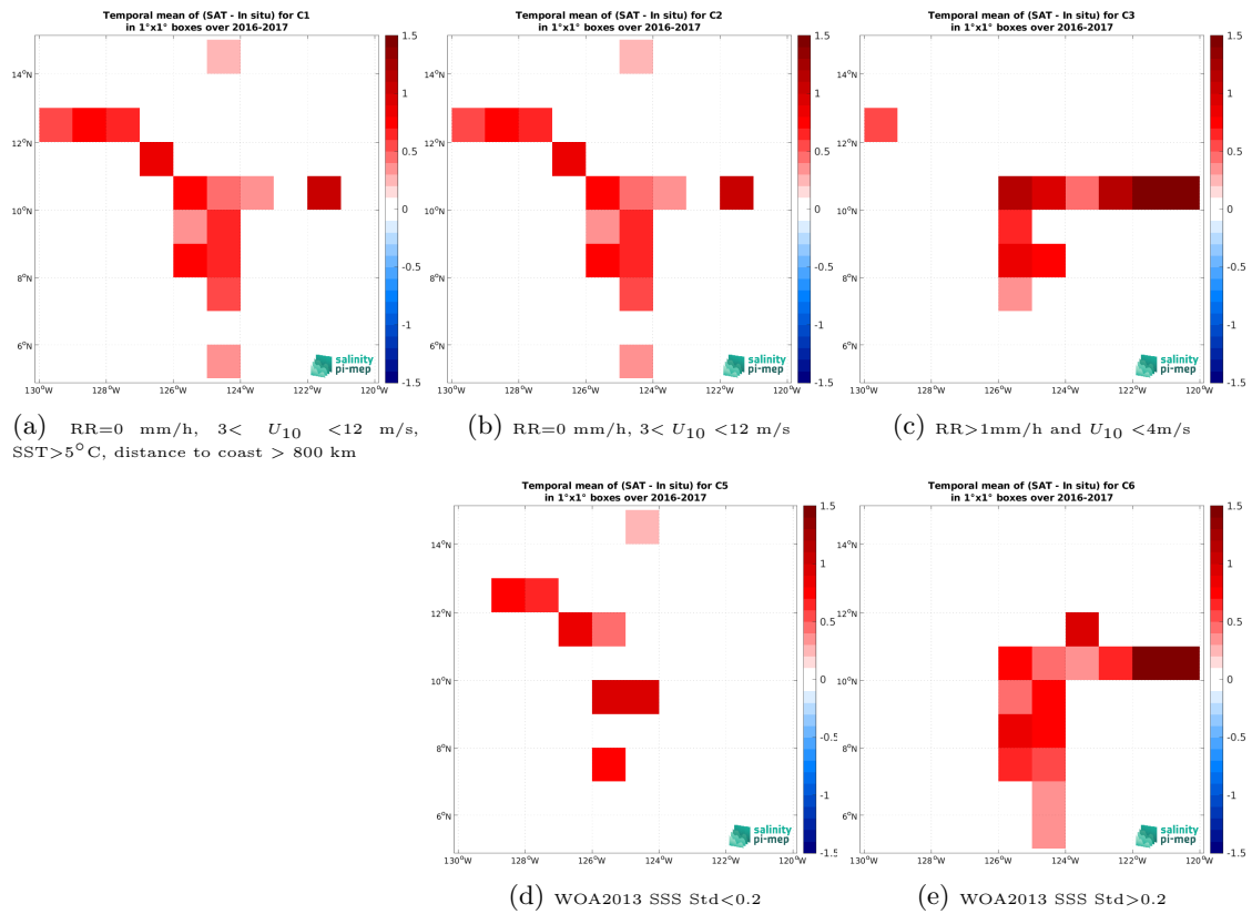
Figure 14: Temporal mean gridded over spatial boxes of size 1^\circ \times 1^\circ of \Delta SSS (SMOS SSS L3 v2 - 9-Days (BEC) - Salinity Snake (SPURS 2)) for 5 different subdatasets corresponding to:RR=0 mm/h, 3 < U_{10} < 12 m/s, SST >5^\circ\text{C} , distance to coast > 800 km (a), RR=0 mm/h, 3 < U_{10} < 12 m/s (b), RR >1 mm/h and U_{10} < 4 m/s (c), WOA2013 SSS Std <0.2 (d), WOA2013 SSS Std >0.2 (e).
