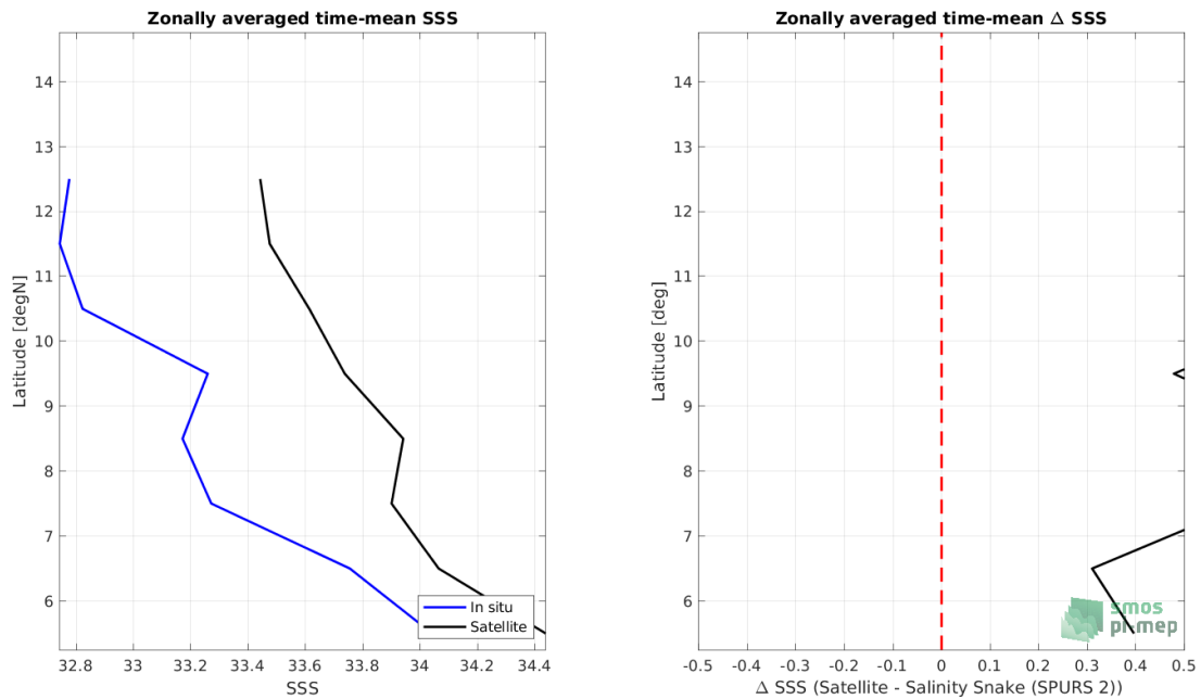
Figure 8: Left panel: Zonal mean SSS from SMOS SSS L3 v2 - 9-Days (BEC) satellite product (black) and from Salinity Snake (SPURS 2) (blue). Right panel: Zonal mean of \Delta SSS (Satellite - Salinity Snake (SPURS 2)) for all the collected Pi-MEP match-up pairs estimated over the full satellite product period.
