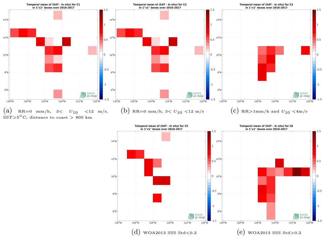
Figure 12: Temporal mean gridded over spatial boxes of size 1^\circ \times 1^\circ of \Delta SSS (SMOS SSS L3 v2 - 9-Days (BEC) - Salinity Snake (SPURS 2)) for 5 different subdatasets corresponding to:RR=0 mm/h, 3 < U_{10} < 12 m/s, SST >5^\circ\text{C} , distance to coast > 800 km (a), RR=0 mm/h, 3 < U_{10} < 12 m/s (b), RR >1 mm/h and U_{10} < 4 m/s (c), WOA2013 SSS Std <0.2 (d), WOA2013 SSS Std >0.2 (e).
