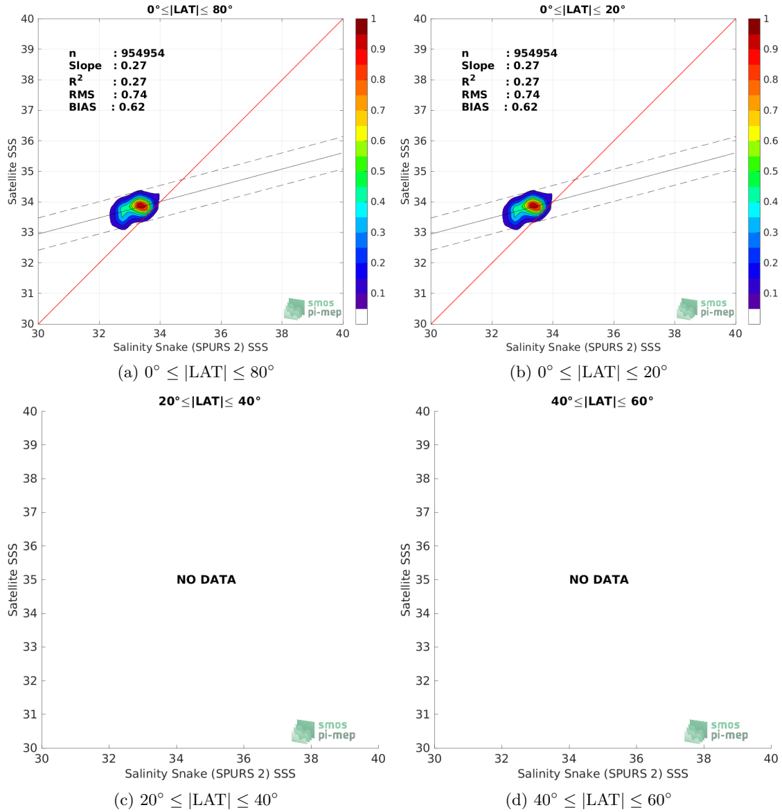
Figure 9: Contour maps of the concentration of SMOS SSS L3 v2 - 9-Days (BEC) SSS (y-axis) versus Salinity Snake (SPURS 2) SSS (x-axis) at match-up pairs for different latitude bands. For each plot, the red line shows x=y . The black thin and dashed lines indicate a linear fit through the data cloud and the \pm 95\% confidence levels, respectively. The number match-up pairs n , the slope and R^2 coefficient of the linear fit, the root mean square (RMS) and the mean bias between satellite and in situ data are indicated for each latitude band in each plots.
