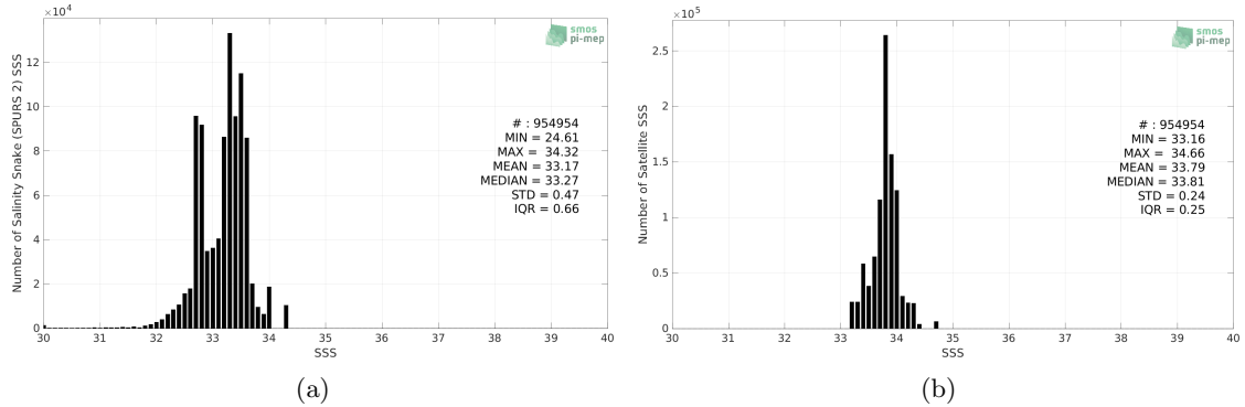
Figure 2: Histograms of SSS from Salinity Snake (SPURS 2) (a) and SMOS SSS L3 v2 - 9-Days (BEC) (b) considering all match-up pairs per bins of 0.1 over the SPURS 2 Pi-MEP region and for the full satellite product period.
