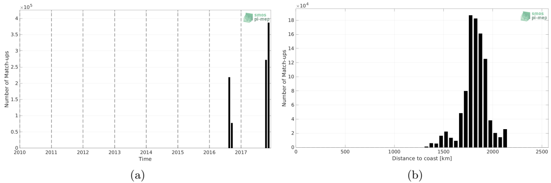
Figure 1: Number of match-ups between Salinity Snake (SPURS 2) and SMOS SSS L3 v2 - 9-Days (BEC) SSS as a function of time (a) and as function of the distance to coast (b) over the SPURS 2 Pi-MEP region and for the full satellite product period.
