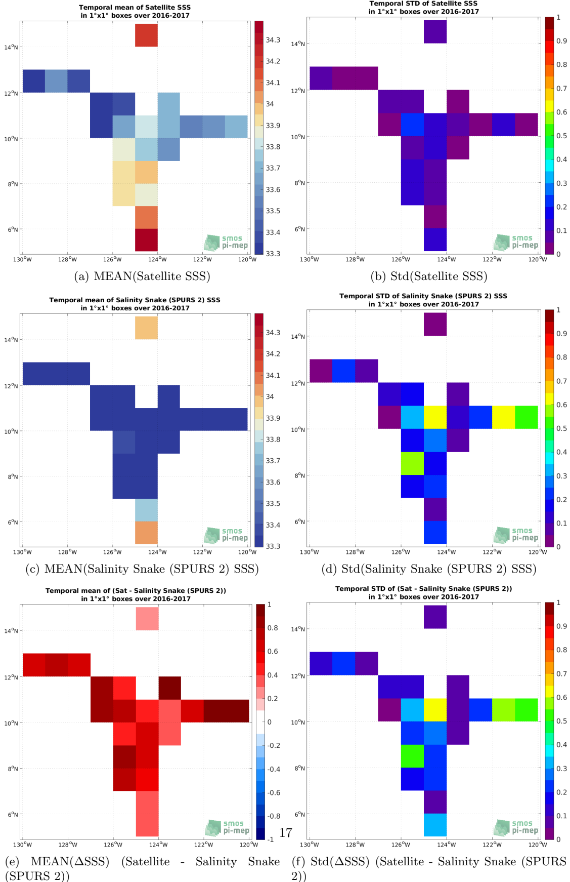
Figure 6: Temporal mean (left) and Std (right) of SSS from SMOS SSS L3 v2 - 9-Days (BEC) (top), Salinity Snake (SPURS 2) (middle), and of \Delta SSS (Satellite - Salinity Snake (SPURS 2)). Only match-up pairs are used to generate these maps.
