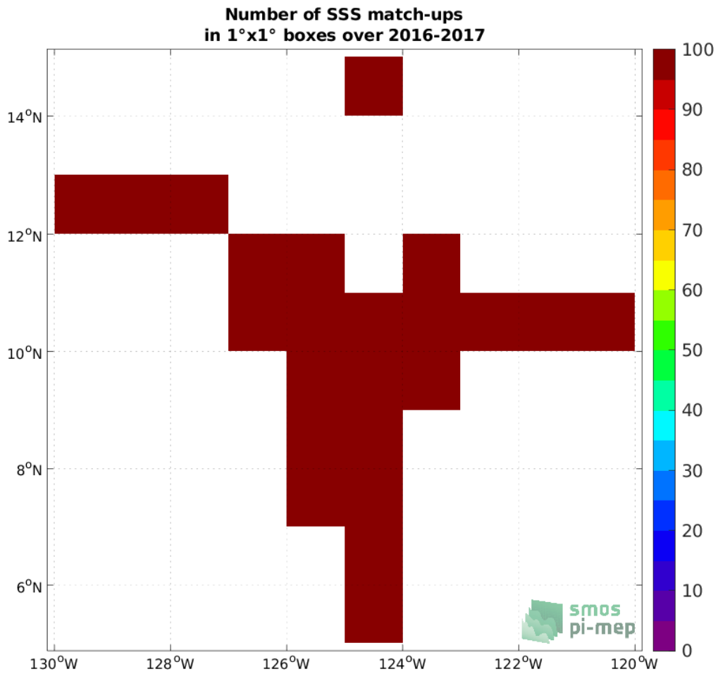
Figure 4: Number of SSS match-ups between Salinity Snake (SPURS 2) SSS and the SMOS SSS L3 v2 - 9-Days (BEC) SSS product for the SPURS 2 Pi-MEP region over 1°x1° boxes and for the full satellite product period.
