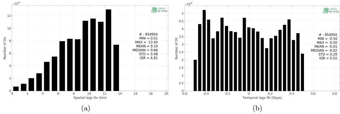
Figure 5: Histograms of the spatial (a) and temporal (b) lags between the location/time of the Salinity Snake (SPURS 2) measurement and the date of the corresponding SMOS SSS L3 v2 - 9-Days (BEC) SSS pixel.
