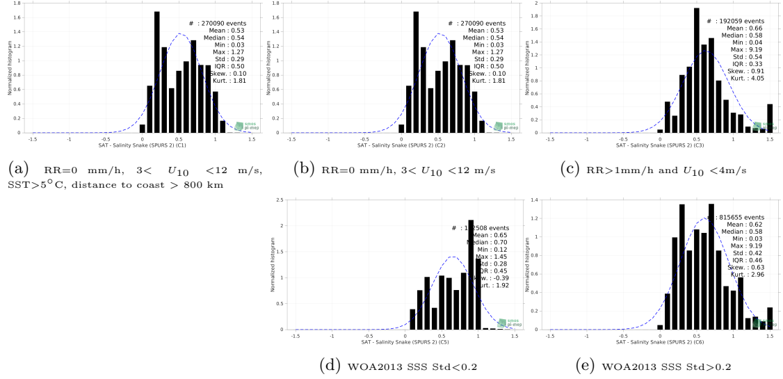
Figure 13: Normalized histogram of \Delta SSS (SMOS SSS L3 v2 - 9-Days (BEC) - Salinity Snake (SPURS 2)) for 5 different subdatasets corresponding to: RR=0 mm/h, 3 < U_{10} < 12 m/s, SST > 5°C, distance to coast > 800 km (a), RR=0 mm/h, 3 < U_{10} < 12 m/s (b), RR > 1mm/h and U_{10} < 4 m/s (c), WOA2013 SSS Std < 0.2 (d), WOA2013 SSS Std > 0.2 (e).
