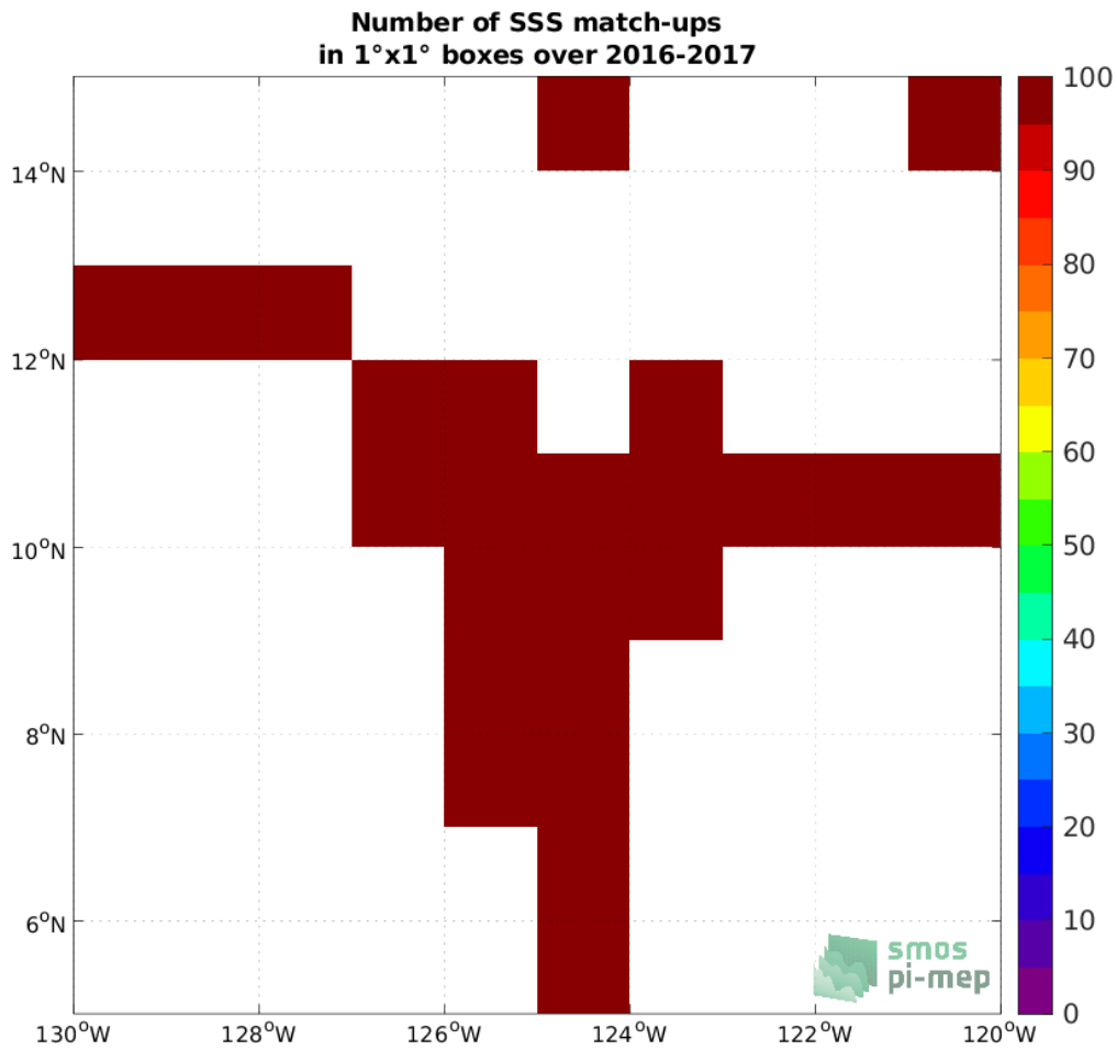
Figure 3: Number of SSS match-ups between Salinity Snake SSS and the SMOS SSS L3 v2 - 9-Days (BEC) SSS product for the SPURS 2 Pi-MEP region over 1°x1° boxes and for the full satellite product period.
