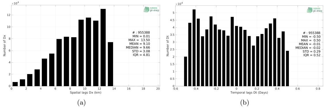
Figure 4: Histograms of the spatial (a) and temporal (b) lags between the location/time of the Salinity Snake measurement and the date of the corresponding SMOS SSS L3 v2 - 9-Days (BEC) SSS pixel.
