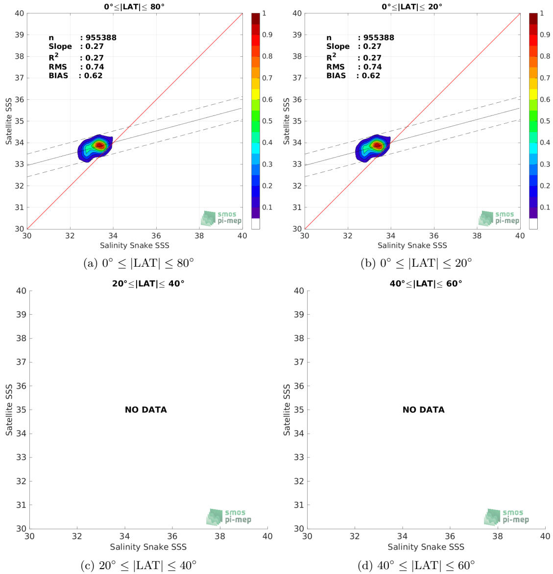
Figure 8: Contour maps of the concentration of SMOS SSS L3 v2 - 9-Days (BEC) SSS (y-axis) versus Salinity Snake SSS (x-axis) at match-up pairs for different latitude bands. For each plot, the red line shows x=y . The black thin and dashed lines indicate a linear fit through the data cloud and the \pm 95\% confidence levels, respectively. The number match-up pairs n , the slope and R^2 coefficient of the linear fit, the root mean square (RMS) and the mean bias between satellite and in situ data are indicated for each latitude band in each plots.
