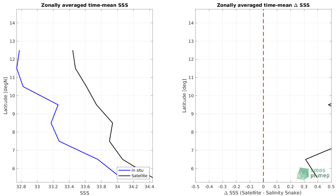
Figure 7: Left panel: Zonal mean SSS from SMOS SSS L3 v2 - 9-Days (BEC) satellite product (black) and from Salinity Snake (blue). Right panel: Zonal mean of \Delta SSS (Satellite - Salinity Snake) for all the collected Pi-MEP match-up pairs estimated over the full satellite product period.
