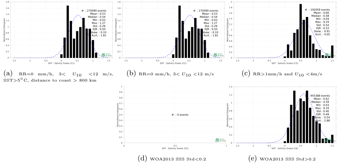
Figure 12: Normalized histogram of \Delta SSS (SMOS SSS L3 v2 - 9-Days (BEC) - Salinity Snake) for 5 different subdatasets corresponding to: RR=0 mm/h, 3 < U_{10} < 12 m/s, SST > 5°C, distance to coast > 800 km (a), RR=0 mm/h, 3 < U_{10} < 12 m/s (b), RR > 1mm/h and U_{10} < 4 m/s (c), WOA2013 SSS Std < 0.2 (d), WOA2013 SSS Std > 0.2 (e).
