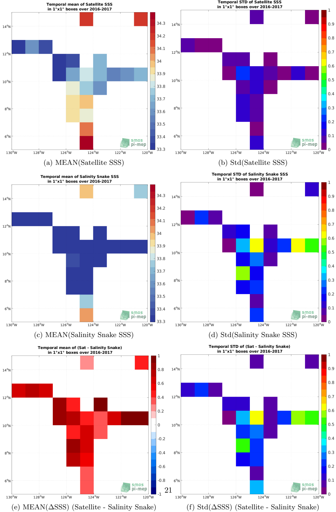
Figure 5: Temporal mean (left) and Std (right) of SSS from SMOS SSS L3 v2 - 9-Days (BEC) (top), Salinity Snake (middle), and of \Delta SSS (Satellite - Salinity Snake). Only match-up pairs are used to generate these maps.
