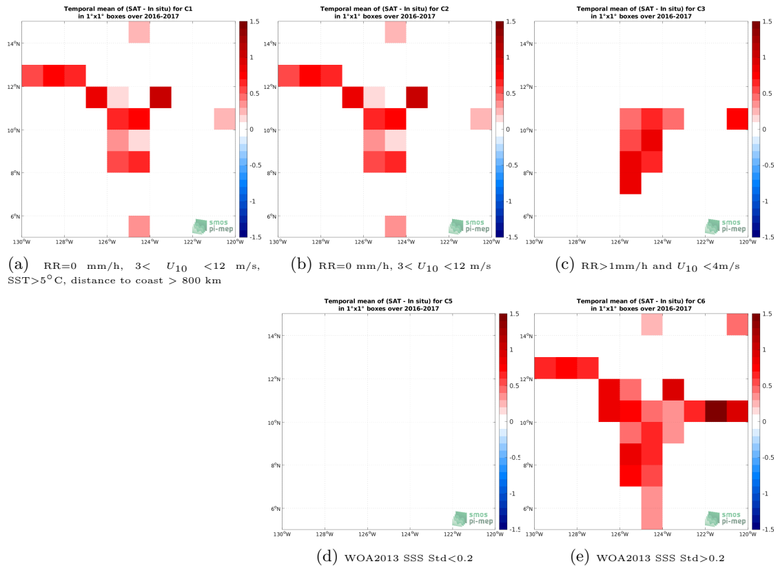
Figure 11: Temporal mean gridded over spatial boxes of size 1^\circ \times 1^\circ of \Delta SSS (SMOS SSS L3 v2 - 9-Days (BEC) - Salinity Snake) for 5 different subdatasets corresponding to:RR=0 mm/h, 3 < U_{10} < 12 m/s, SST >5^\circ\text{C} , distance to coast > 800 km (a), RR=0 mm/h, 3 < U_{10} < 12 m/s (b), RR >1 mm/h and U_{10} < 4 m/s (c), WOA2013 SSS Std <0.2 (d), WOA2013 SSS Std >0.2 (e).
