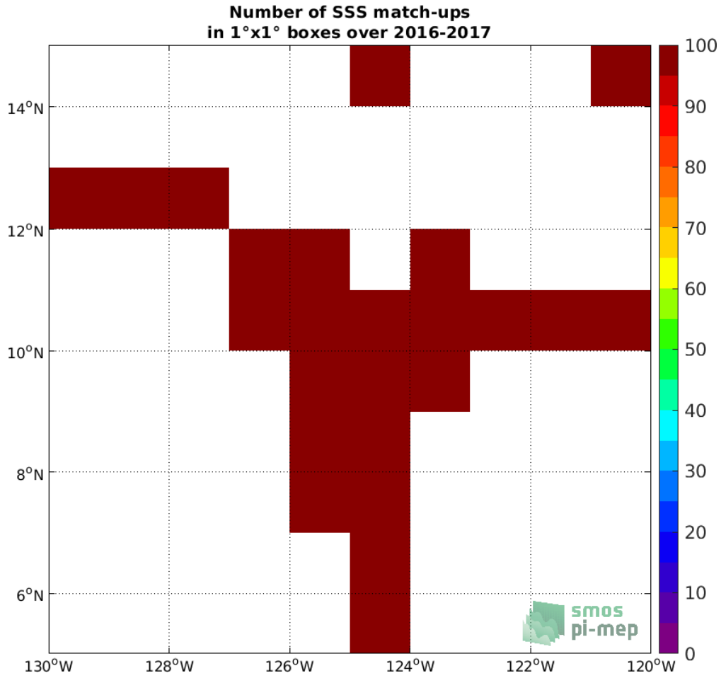
Figure 3: Number of SSS match-ups between Salinity Snake SSS and the SMOS SSS L3 v2 - 9-Days (BEC) SSS product for the SPURS 2 Pi-MEP region over 1^\circ \times 1^\circ boxes and for the full satellite product period.
